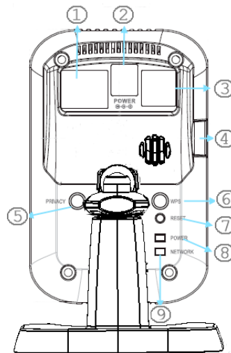
Figure 3: Rear Panel
