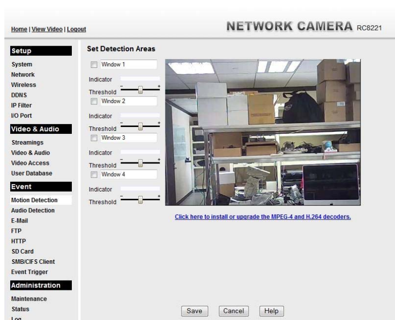
Figure 26: Motion Detection
