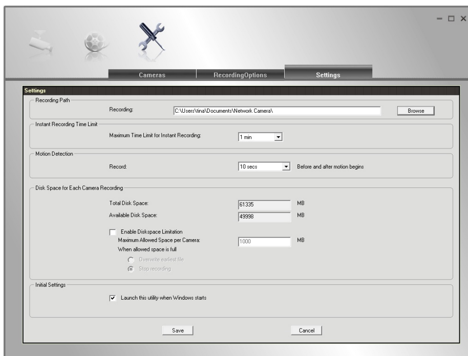
Figure 55: Settings Screen
