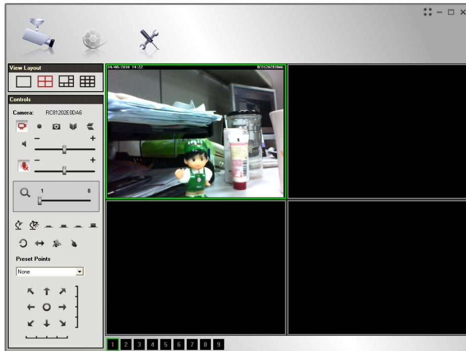
Figure 51: Main Screen
