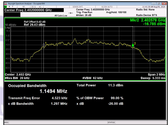
\pi/4 DQPSK_2-DH1_Channel 0
