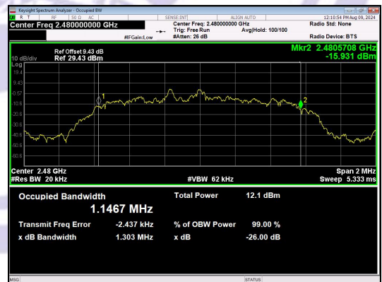
\pi/4 DQPSK_2-DH1_Channel 78
