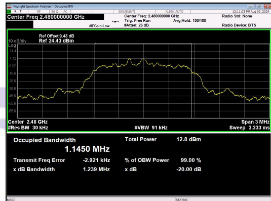
\pi/4 DQPSK_2-DH1_Channel 78
