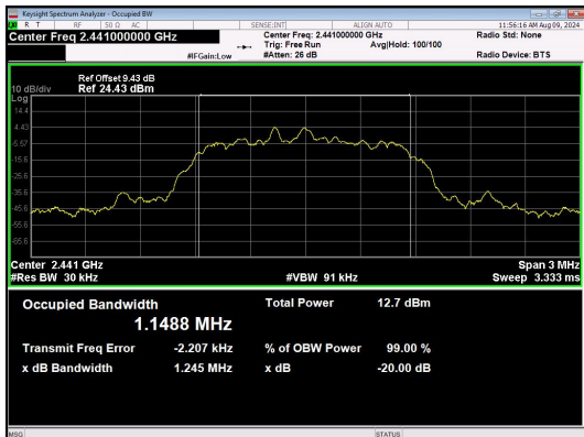
\pi/4 DQPSK_2-DH1_Channel 39
