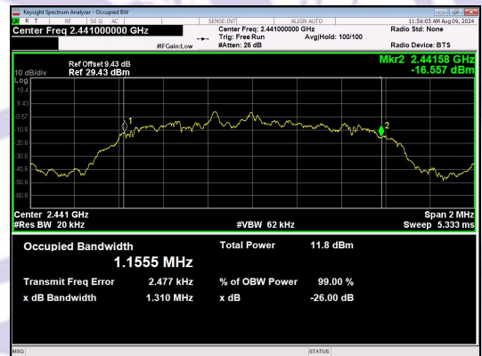
\pi/4 DQPSK_2-DH1_Channel 39
