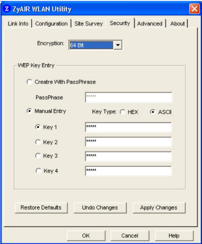
Figure 2-8 Security
