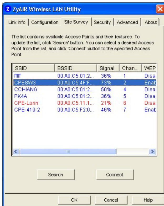
Figure 2-6 Site Survey
