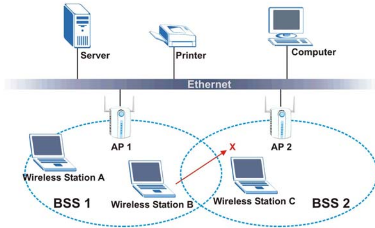
Figure 2-3 Roaming Example
