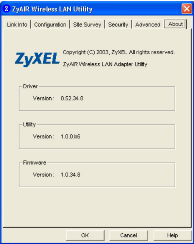
Figure 2-11 About
