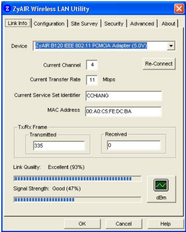
Figure 2-4 Link Info
