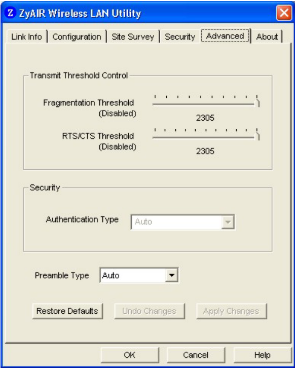
Figure 2-10 Advanced
