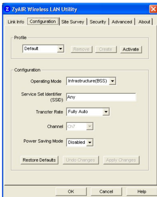
Figure 2-5 Configuration
