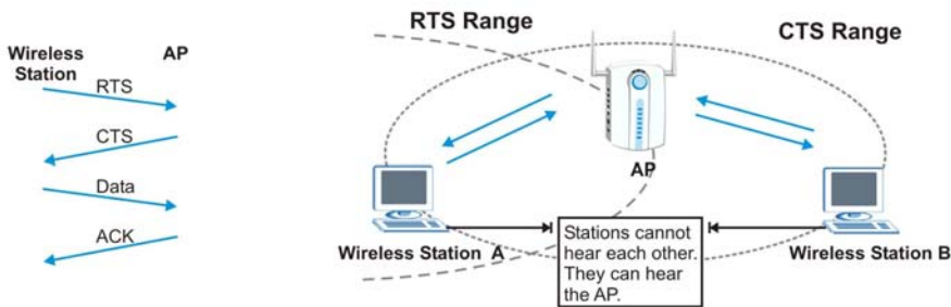
Figure 2-9 RTS Threshold
