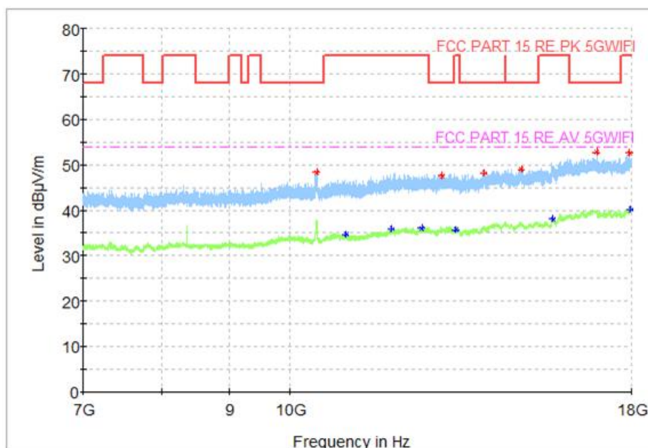
Fig. 58 Transmitter Spurious Emission (802. 11ac-VHT40, CH46 5230MHz)
