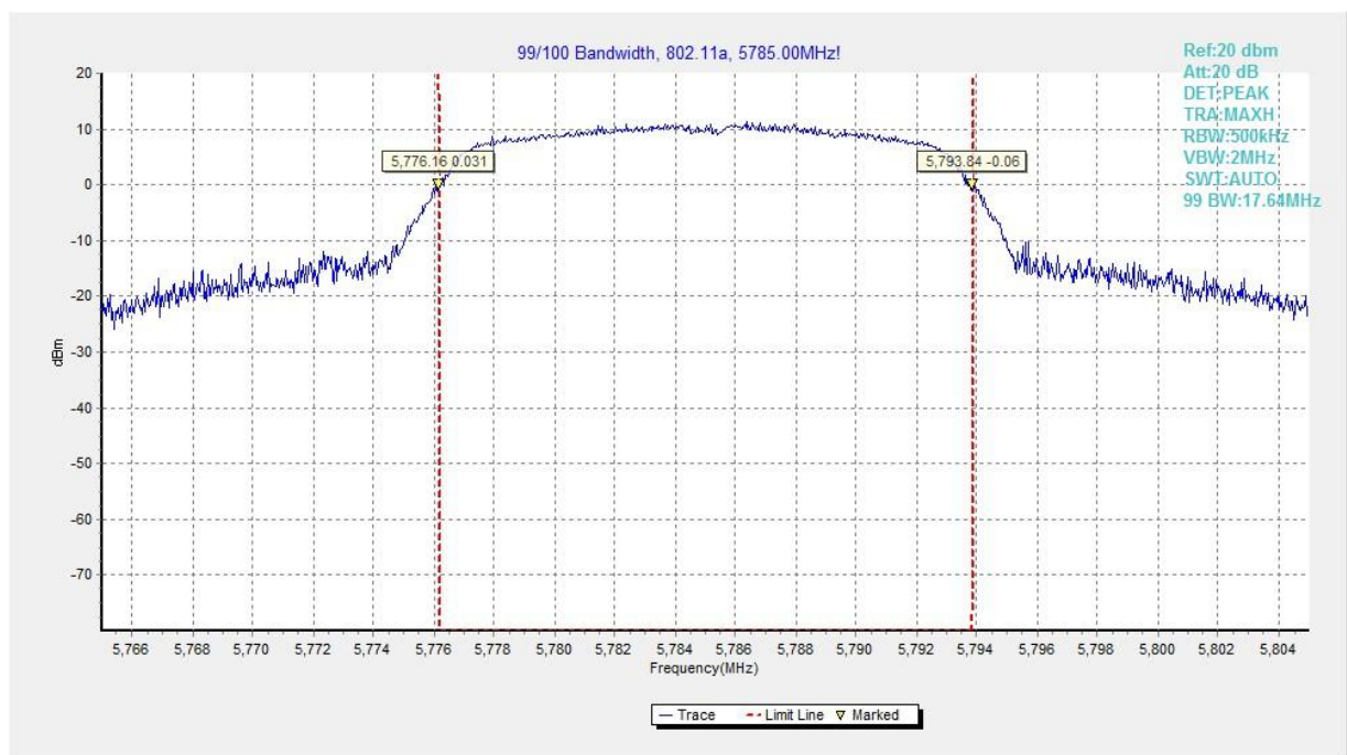
Fig. 26 99% Occupied Bandwidth (802.11a, 5785MHz)
