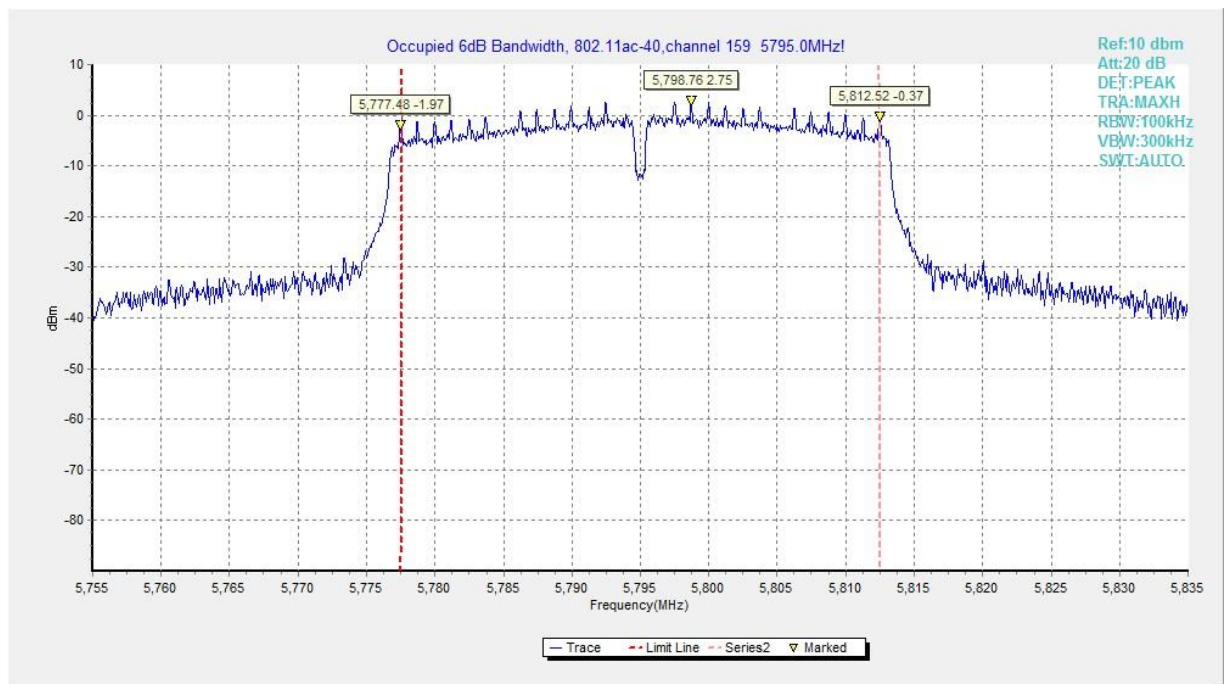
Fig. 17 Occupied 6dB Bandwidth (802.11ac-VHT40, 5795MHz)
