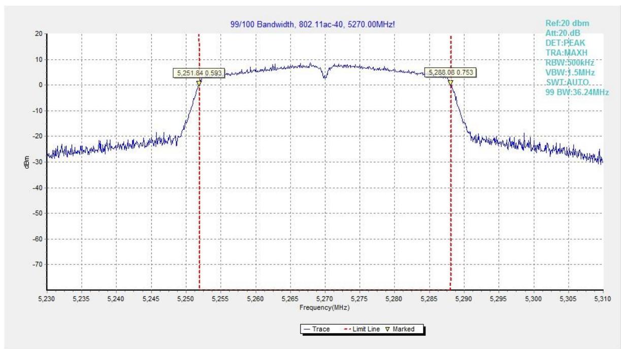
Fig. 30 99% Occupied Bandwidth (802.11ac-VHT40, 5270MHz)
