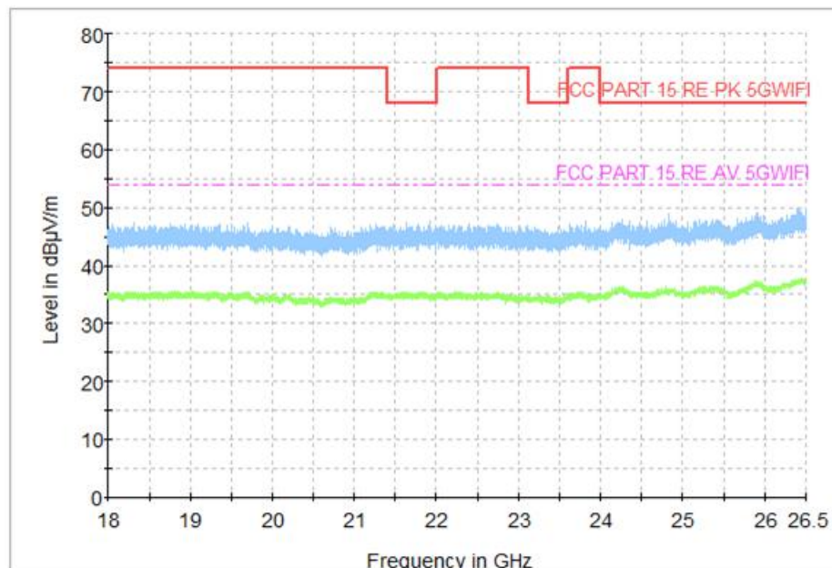
Fig. 69 Transmitter Spurious Emission (All channel, 18GHz~26.5GHz)
