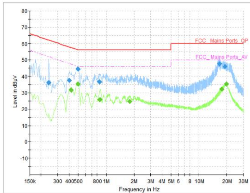
Fig. 72 AC Power line Conducted Emission (Traffic)
