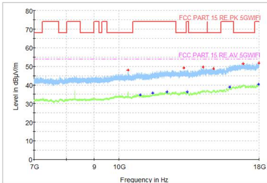
Fig. 57 Transmitter Spurious Emission (802. 11ac-VHT40, CH38 5190MHz)
