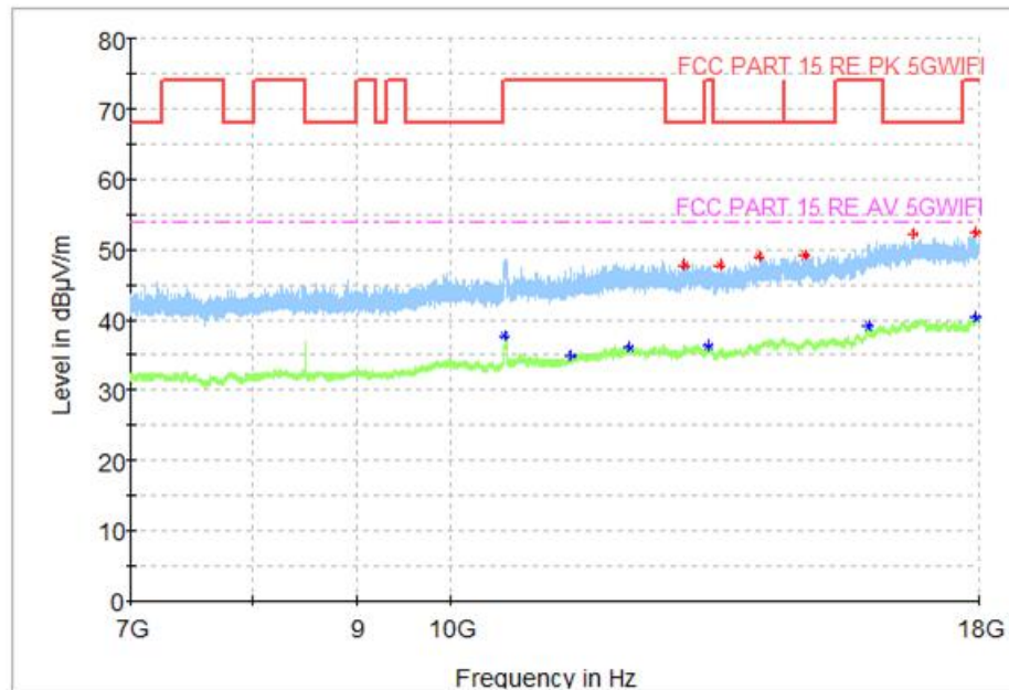
Fig. 60 Transmitter Spurious Emission (802. 11ac-VHT40, CH62 5310MHz)
