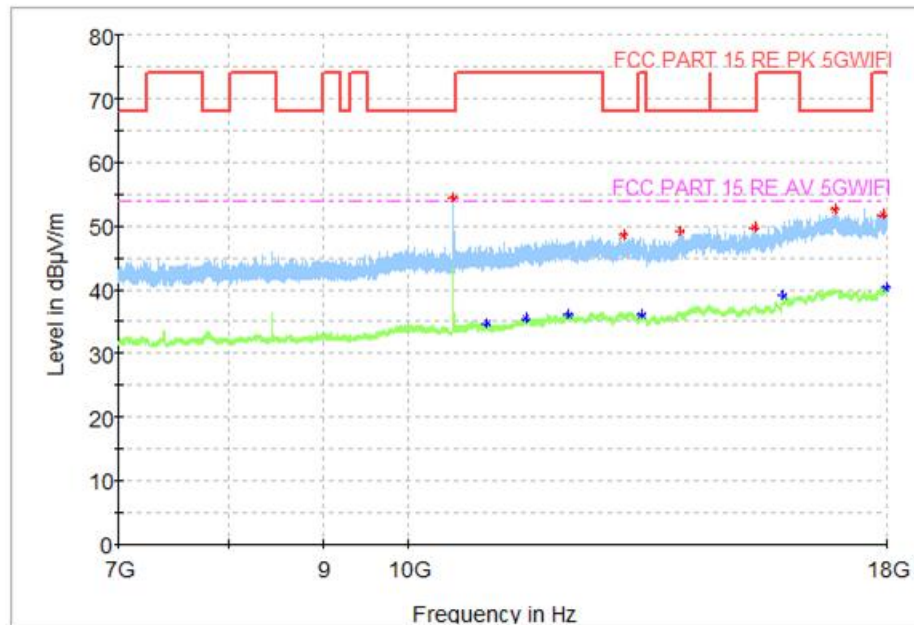
Fig. 52 Transmitter Spurious Emission (802.11a, CH56 5280MHz)
