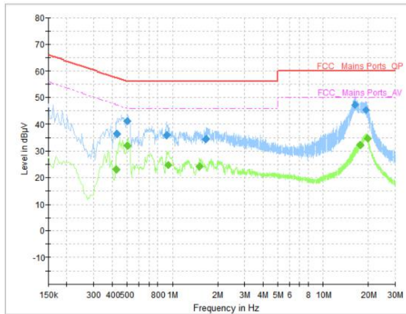
Fig. 73 AC Power line Conducted Emission (Idle)
