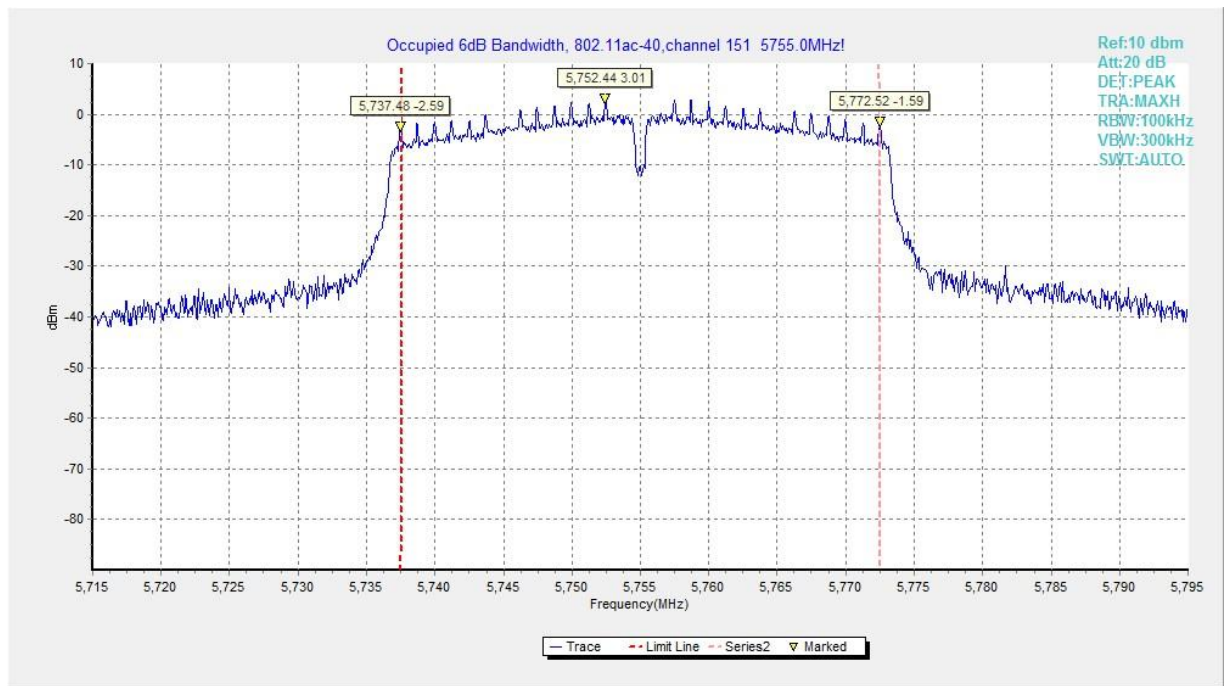
Fig. 16 Occupied 6dB Bandwidth (802.11ac-VHT40, 5755MHz)
