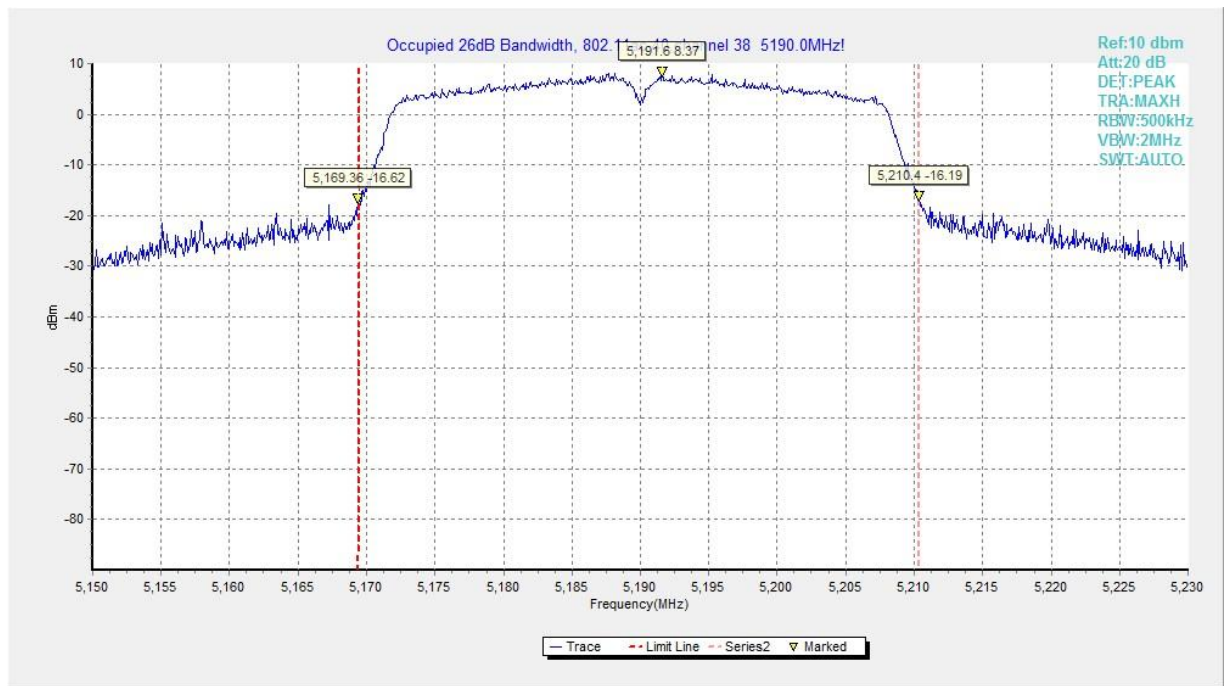
Fig. 7 Occupied 26dB Bandwidth (802.11ac-VHT40, 5190MHz)
