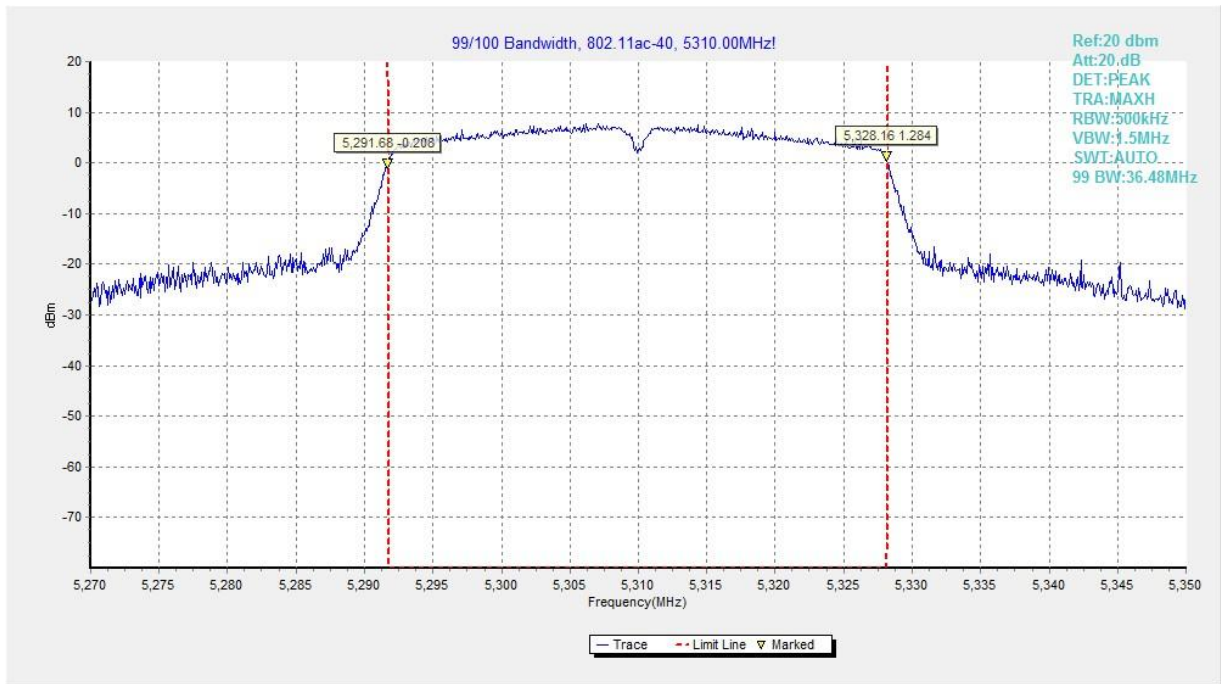
Fig. 31 99% Occupied Bandwidth (802. 11ac-VHT40, 5310MHz)
