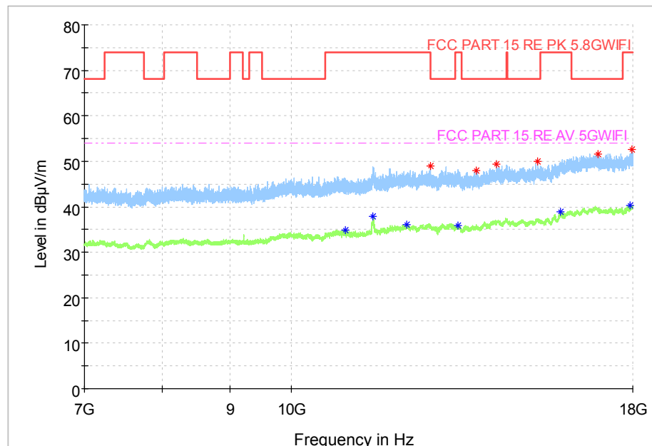
Fig. 61 Transmitter Spurious Emission (802. 11ac-VHT40, CH151 5755MHz)
