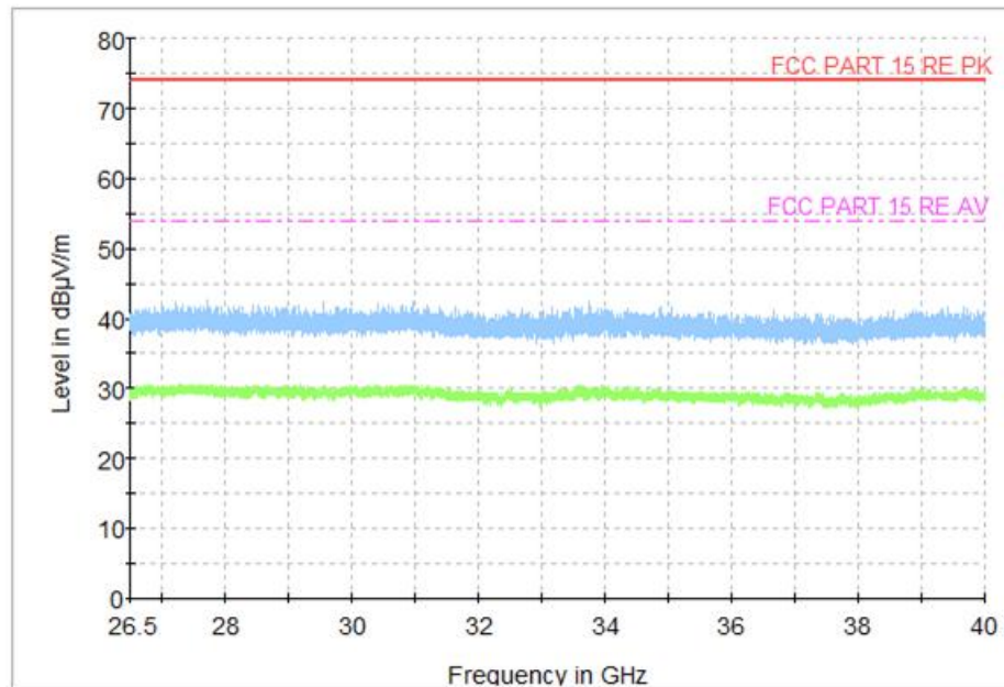
Fig. 70 Transmitter Spurious Emission (All channel, 26.5GHz~40GHz)
