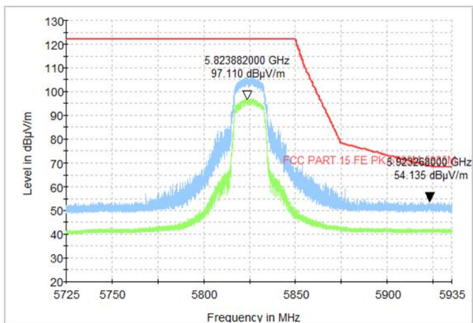
Fig. 40 Band Edges (802.11a, CH165 5825MHz)
