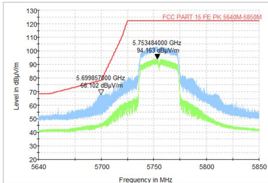
Fig. 43 Band Edges (802.11ac-VHT40, CH151 5755MHz)
