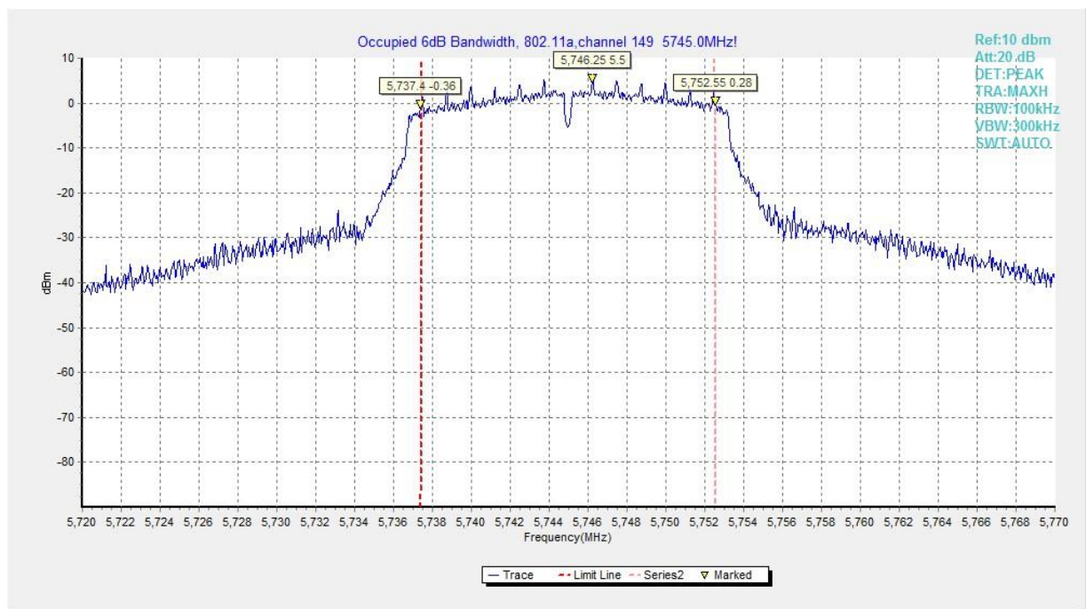
Fig. 13 Occupied 6dB Bandwidth (802.11a, 5745MHz)
