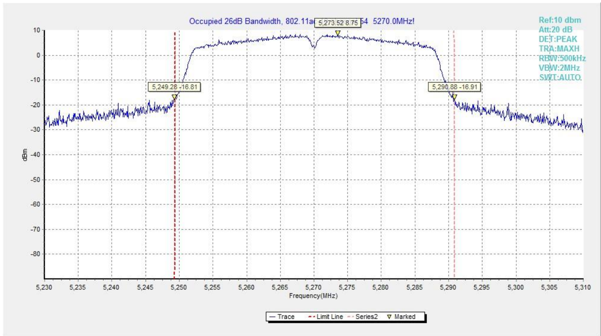
Fig. 9 Occupied 26dB Bandwidth (802. 11ac-VHT40, 5270MHz)
