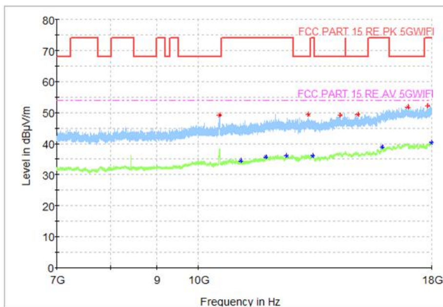
Fig. 59 Transmitter Spurious Emission (802. 11ac-VHT40, CH54 5270MHz)
