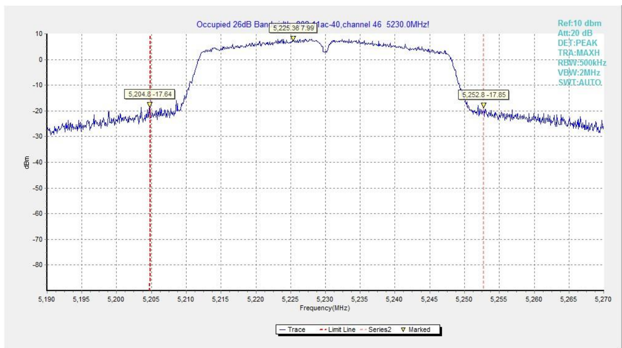
Fig. 8 Occupied 26dB Bandwidth (802.11ac-VHT40, 5230MHz)
