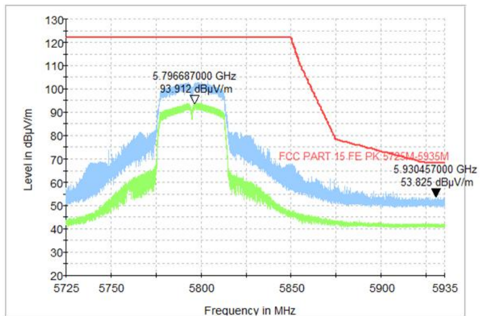
Fig. 44 Band Edges (802.11ac-VHT40, CH159 5795MHz)
