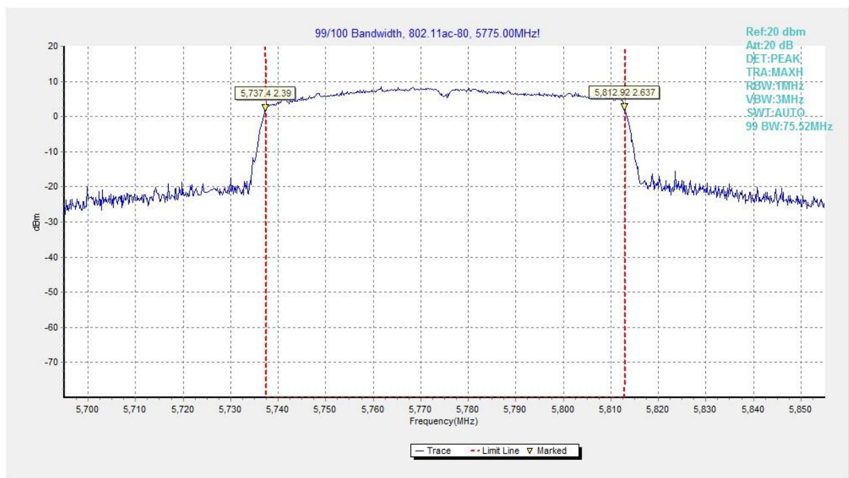
Fig. 36 99% Occupied Bandwidth (802.11ac-VHT80, 5775MHz)
