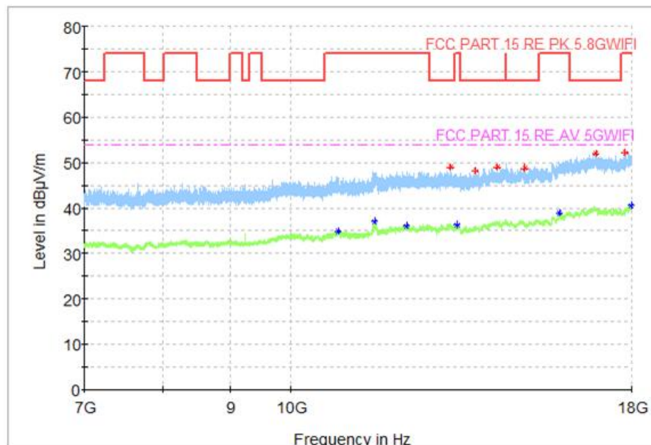
Fig. 65 Transmitter Spurious Emission (802. 11ac-VHT80, CH155 5775MHz)
