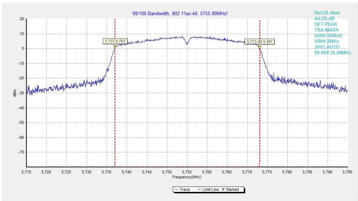
Fig. 32 99% Occupied Bandwidth (802. 11ac-VHT40, 5755MHz)
