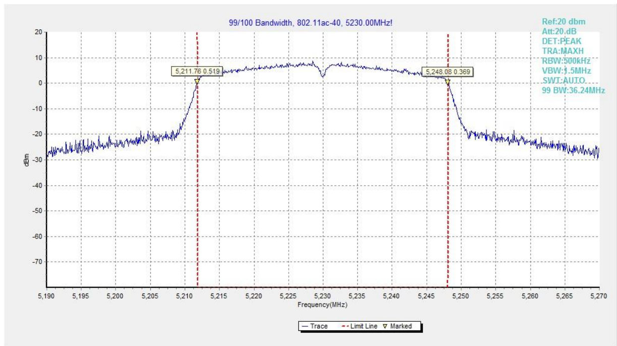
Fig. 29 99% Occupied Bandwidth (802.11ac-VHT40, 5230MHz)
