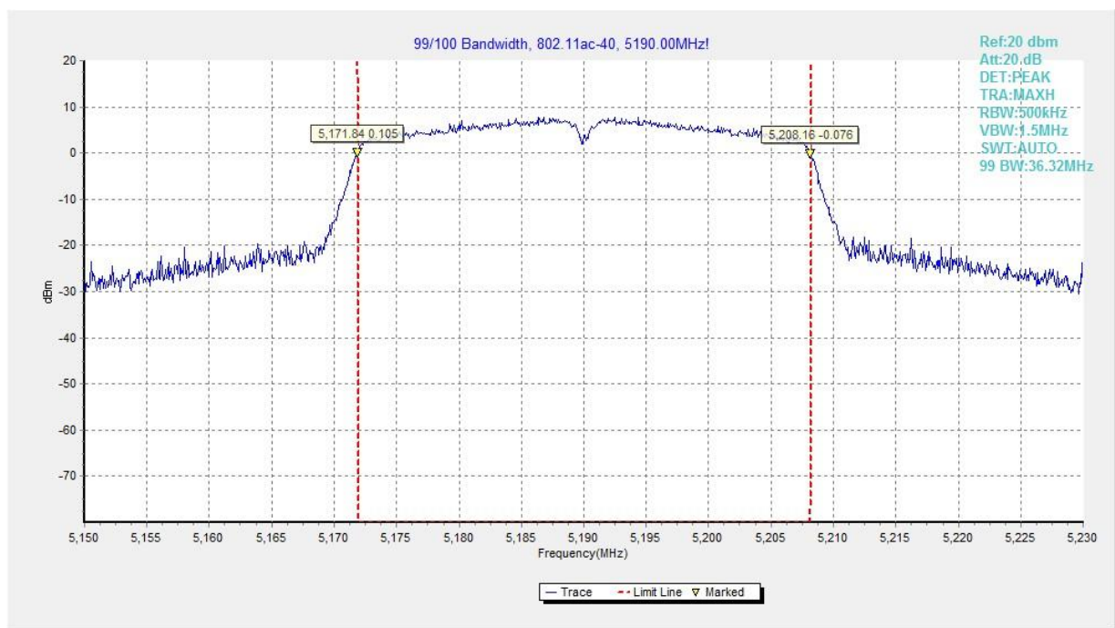
Fig. 28 99% Occupied Bandwidth (802.11ac-VHT40, 5190MHz)
