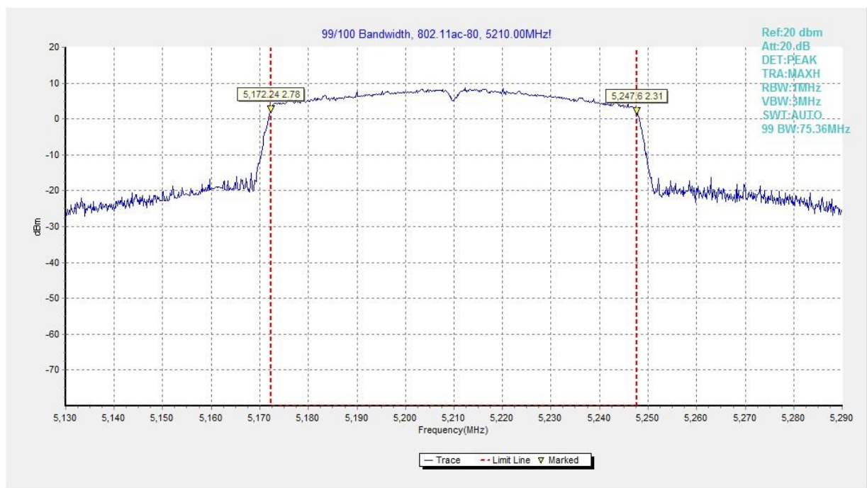
Fig. 34 99% Occupied Bandwidth (802. 11ac-VHT80, 5210MHz)
