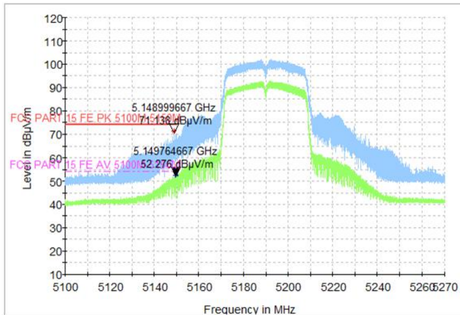
Fig. 41 Band Edges (802.11ac-VHT40, CH38 5190MHz)
