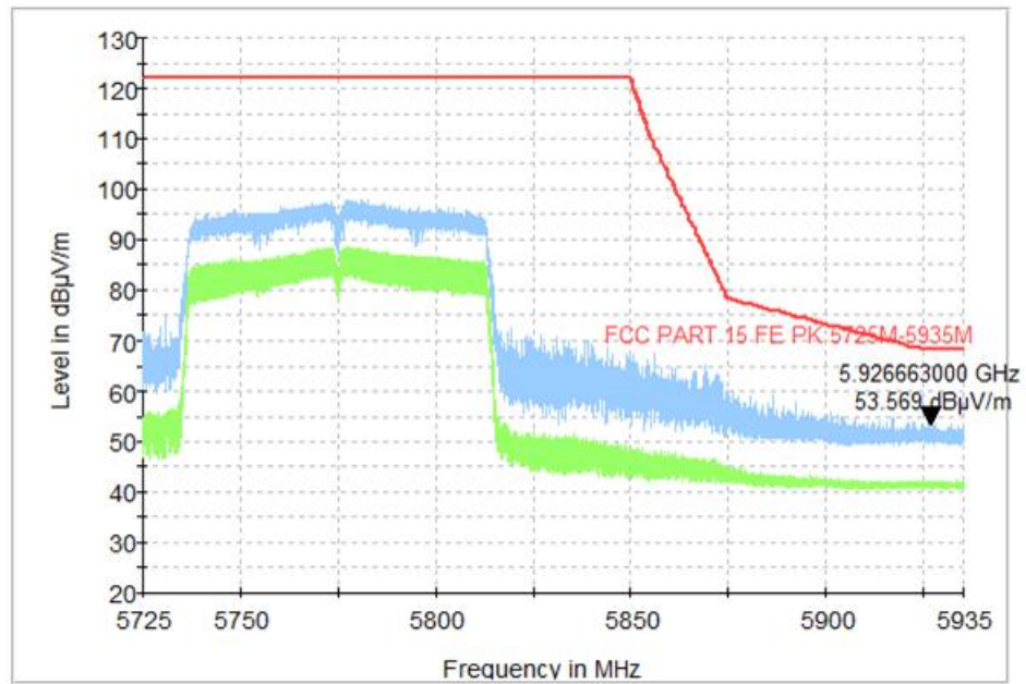
Fig. 47 Band Edges (802.11ac-VHT80, CH155 5775MHz)
