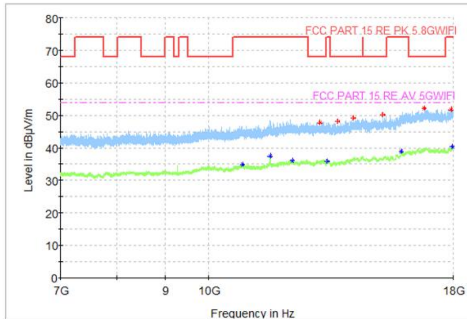
Fig. 62 Transmitter Spurious Emission (802. 11ac-VHT40, CH159 5795MHz)
