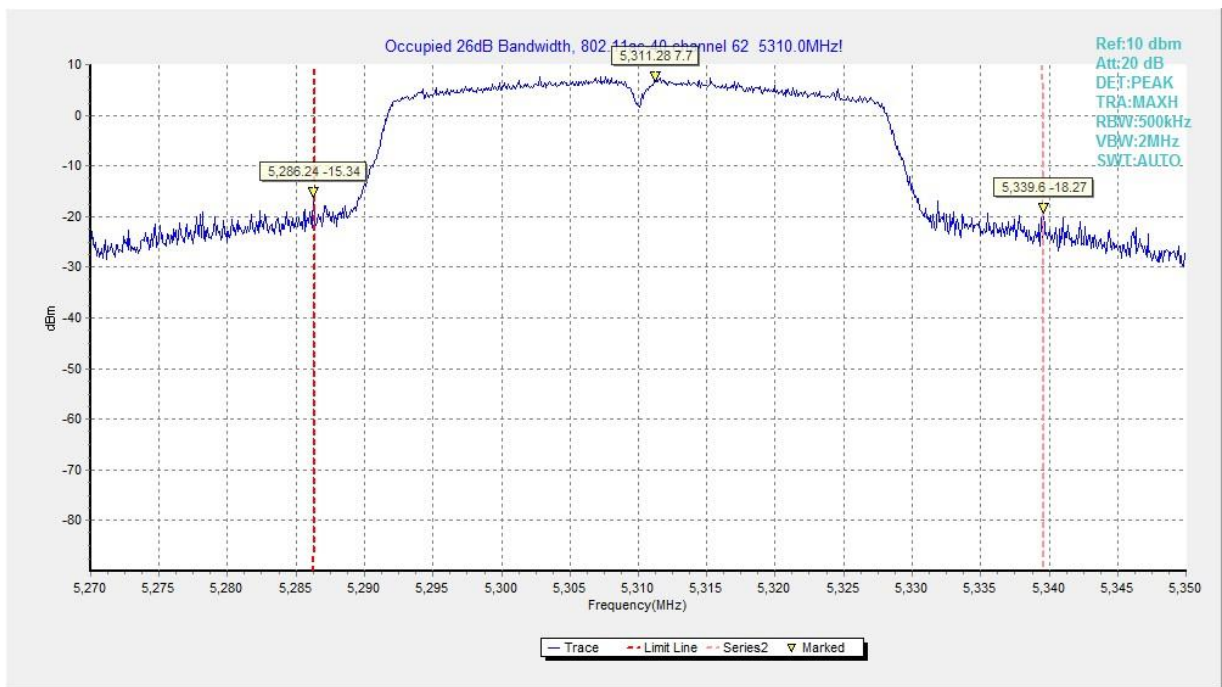
Fig. 10 Occupied 26dB Bandwidth (802. 11ac-VHT40, 5310MHz)
