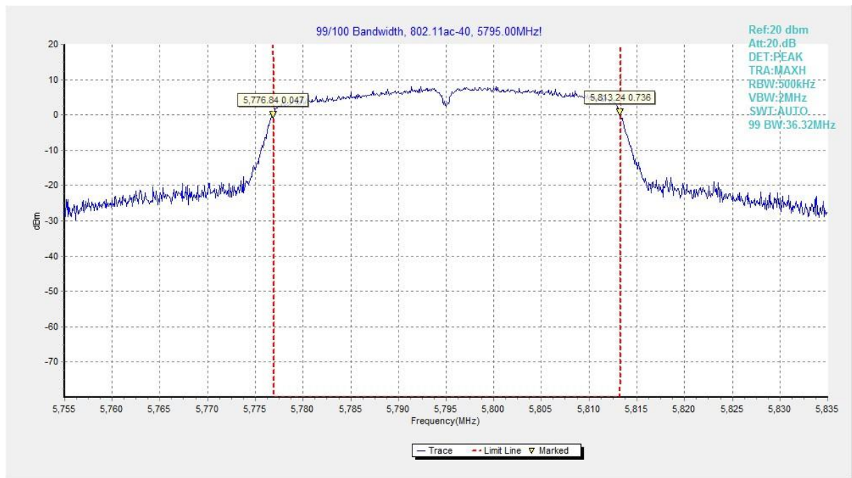
Fig. 33 99% Occupied Bandwidth (802. 11ac-VHT40, 5795MHz)
