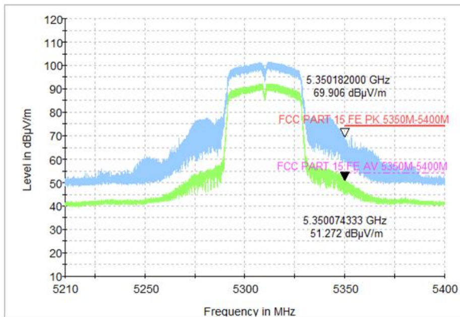
Fig. 42 Band Edges (802.11ac-VHT40, CH62 5310MHz)
