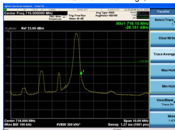
LTE Band 12 16QAM 3MHz CH-High, 1 RB 716MHz~717MHz
