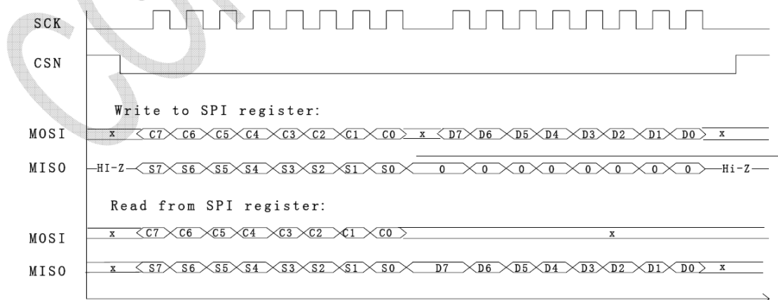
Figure 6 SPI timing
