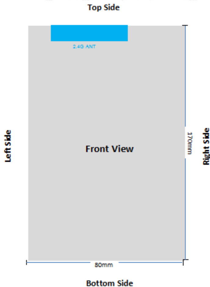
Distance of The Antenna vertical to the EUT surface and edge
