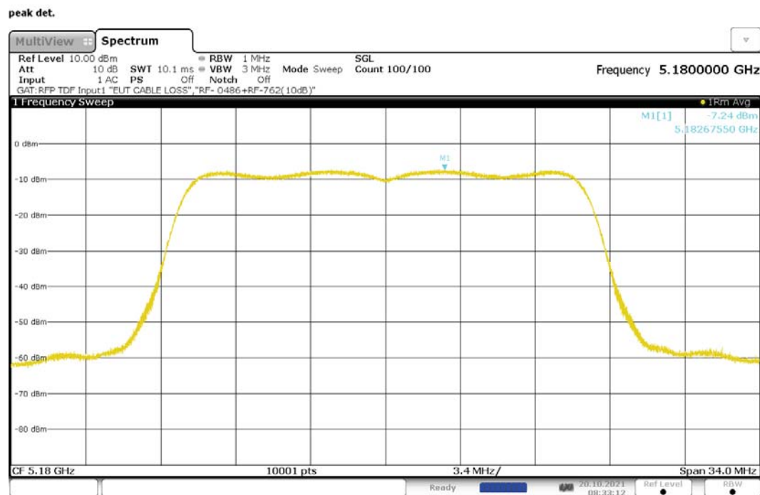
Figure 185: Maximum Power Spectral Density, 802.11ac-20, SISO, RF1, 5180MHz
