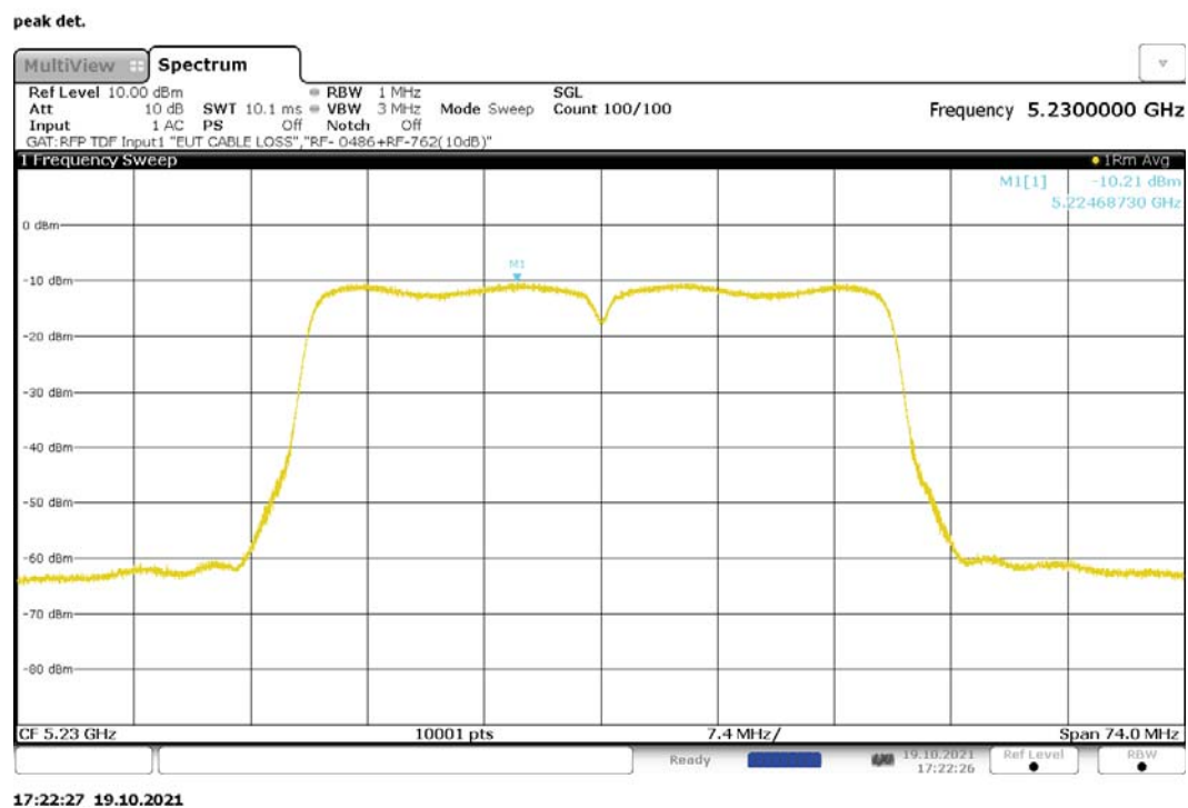
Figure 260: Maximum Power Spectral Density, 802.11ac-40, MIMO, RF1, 5230MHz
