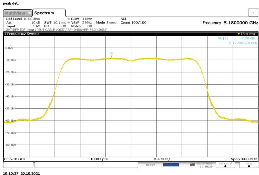
Figure 203: Maximum Power Spectral Density, 802.11ac-20, MIMO, RF0, 5180MHz
