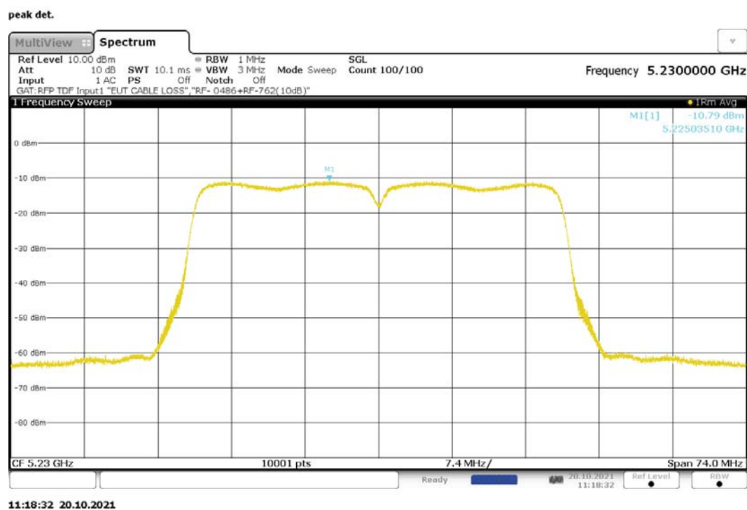
Figure 216: Maximum Power Spectral Density, 802.11n-40, SISO, RF0, 5230MHz
