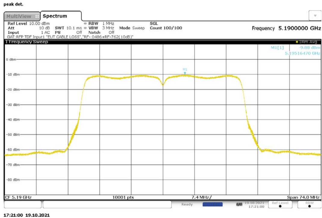
Figure 259: Maximum Power Spectral Density, 802.11ac-40, MIMO, RF1, 5190MHz
