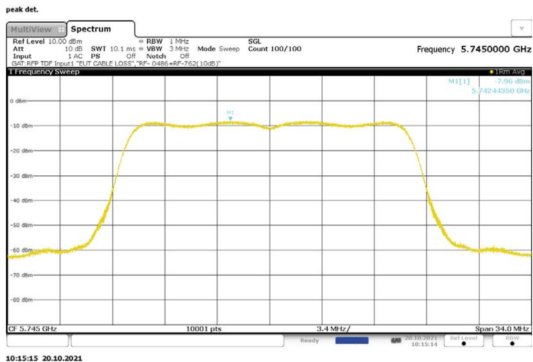
Figure 206: Maximum Power Spectral Density, 802.11ac-20, MIMO, RF0, 5745MHz
