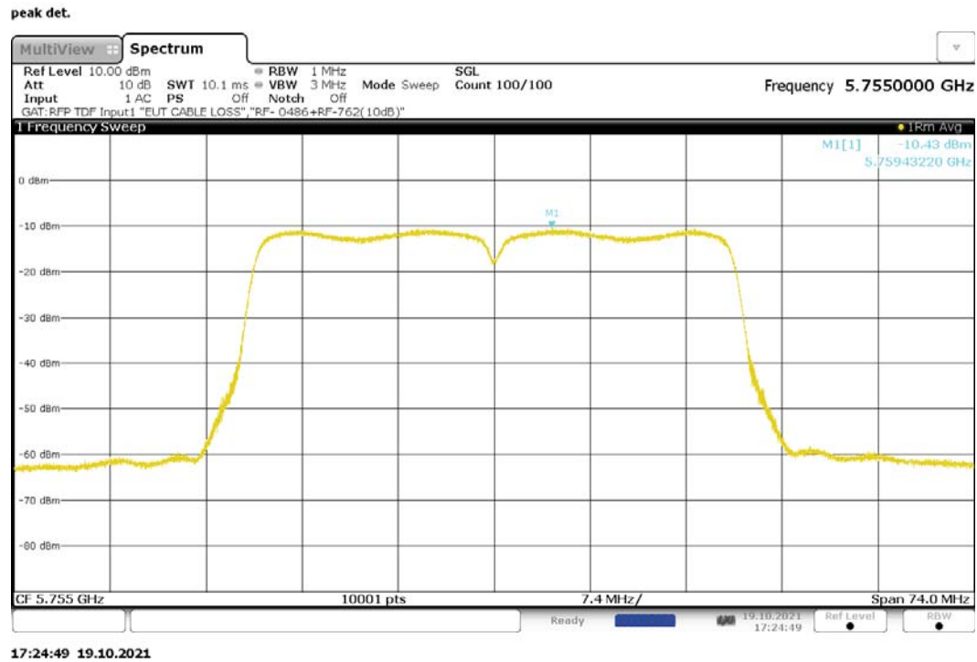
Figure 261: Maximum Power Spectral Density, 802.11ac-40, MIMO, RF1, 5755MHz
