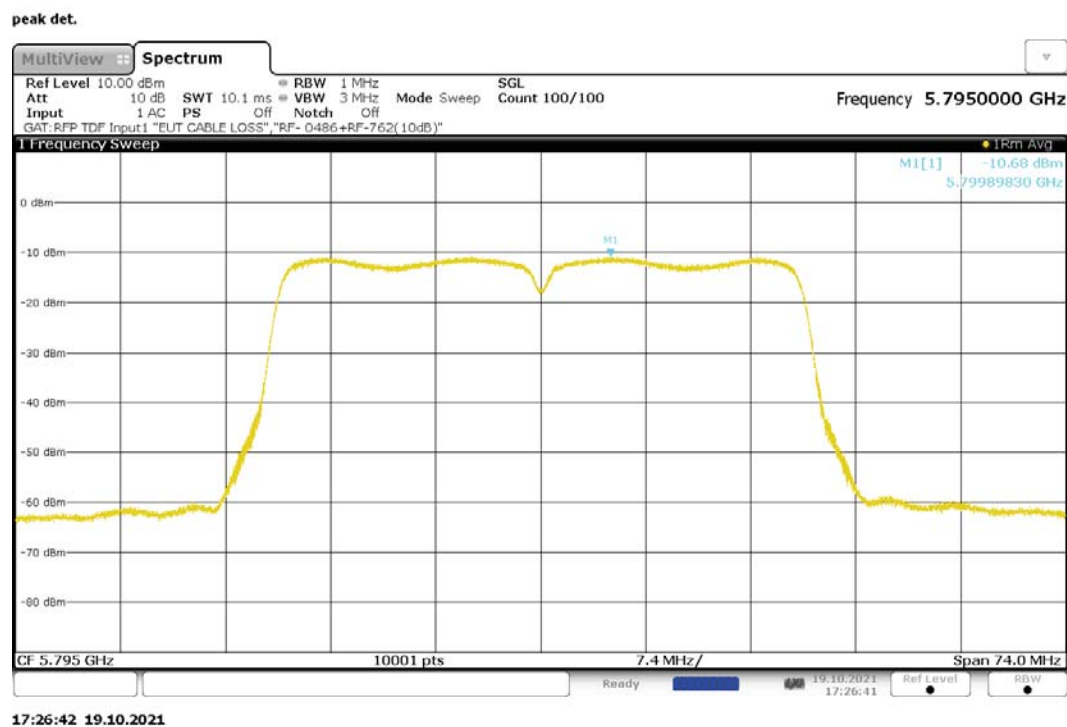
Figure 254: Maximum Power Spectral Density, 802.11ac-40, CDD, RF1, 5795MHz
