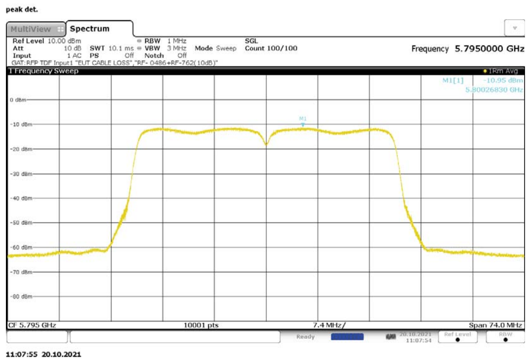
Figure 250: Maximum Power Spectral Density, 802.11ac-40, CDD, RF0, 5795MHz
