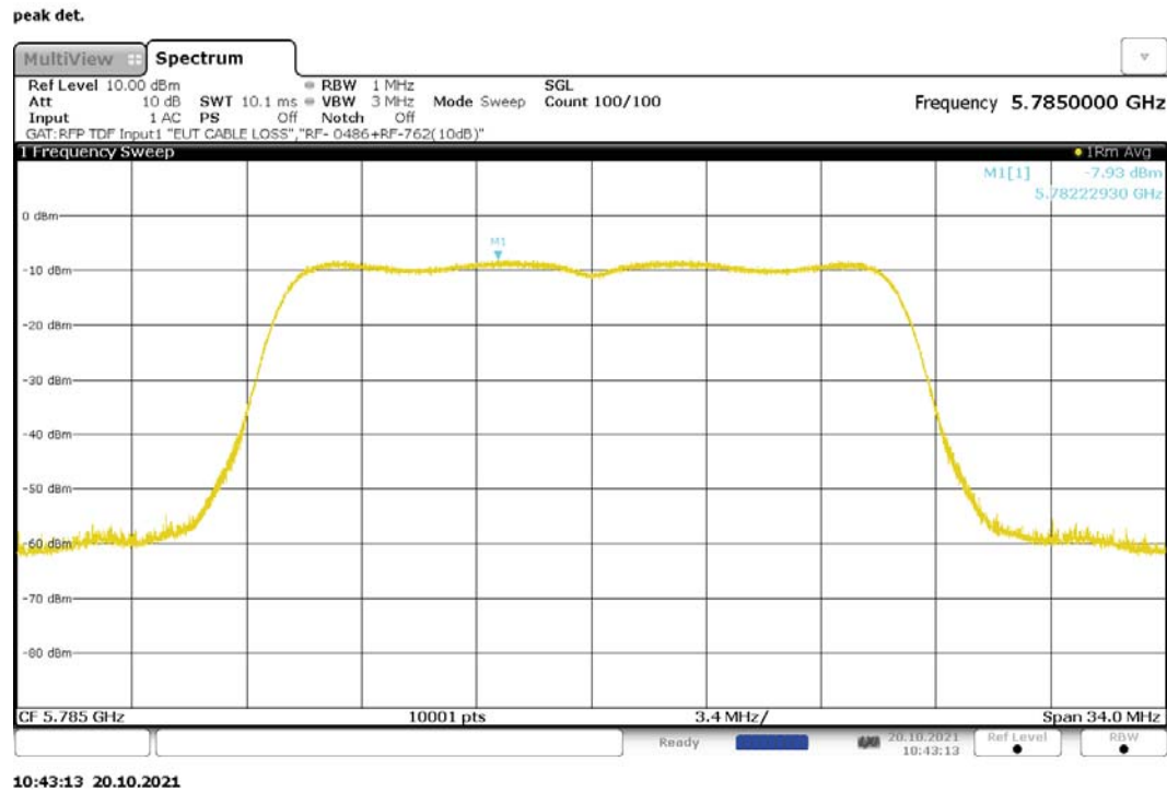
Figure 171: Maximum Power Spectral Density, 802.11n-20, MIMO, RF0, 5785MHz
