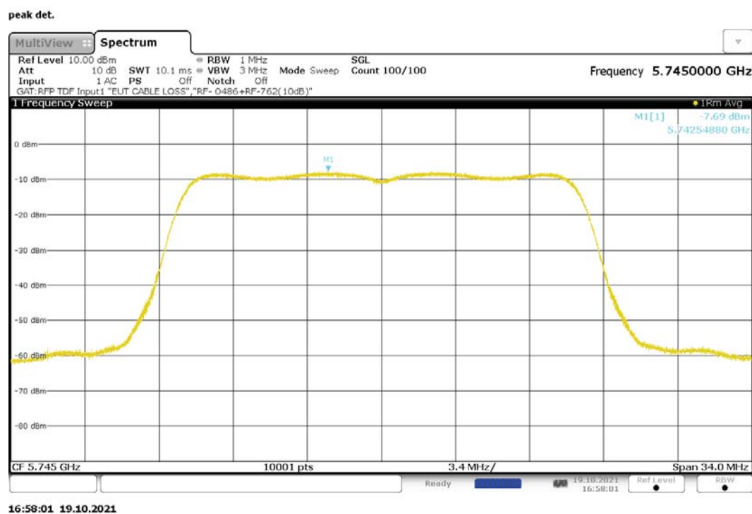
Figure 212: Maximum Power Spectral Density, 802.11ac-20, MIMO, RF1, 5745MHz
