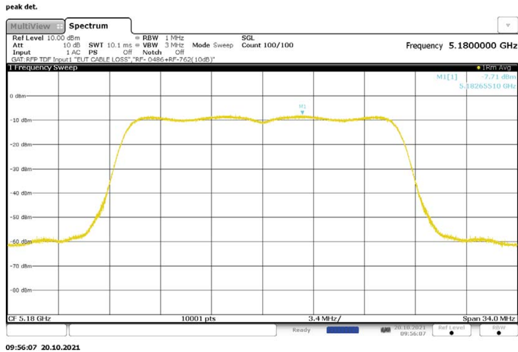
Figure 179: Maximum Power Spectral Density, 802.11ac-20, SISO, RF0, 5180MHz
