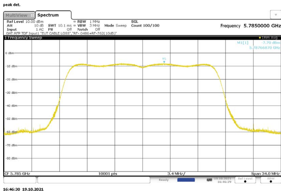
Figure 177: Maximum Power Spectral Density, 802.11n-20, MIMO, RF1, 5785MHz
