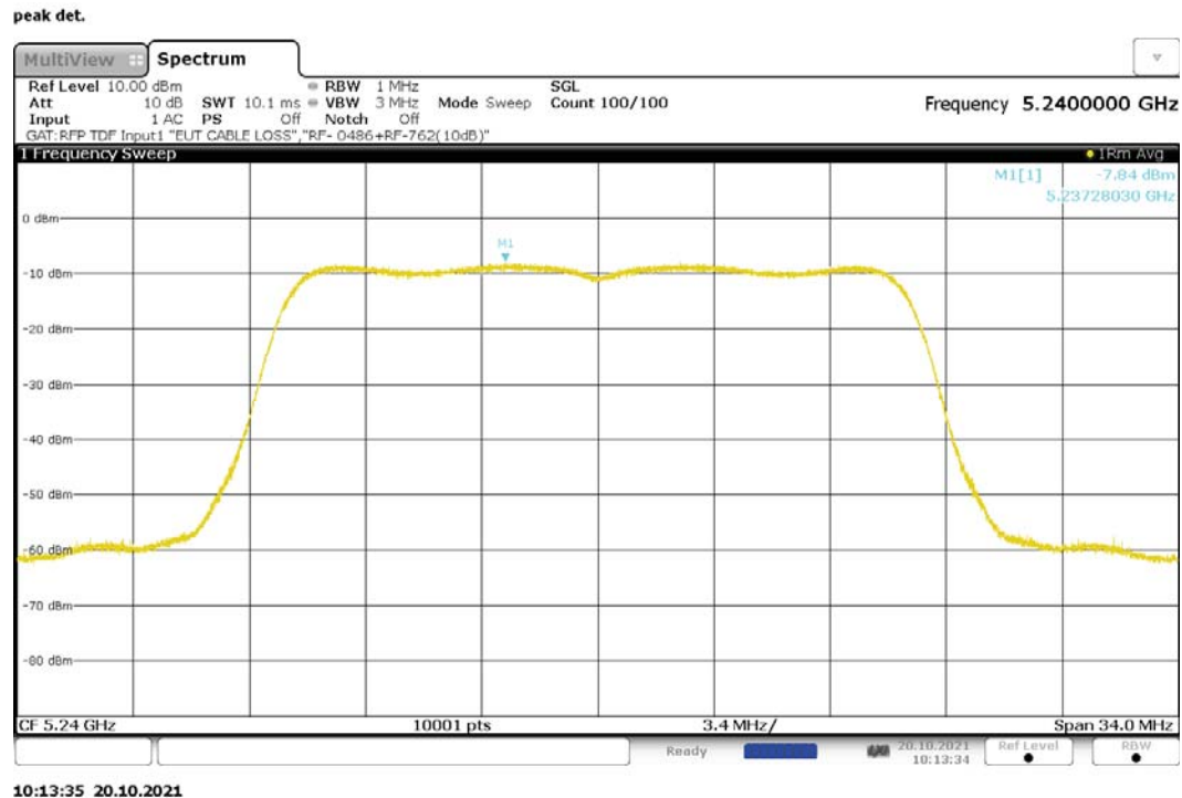
Figure 193: Maximum Power Spectral Density, 802.11ac-20, CDD, RF0, 5240MHz
