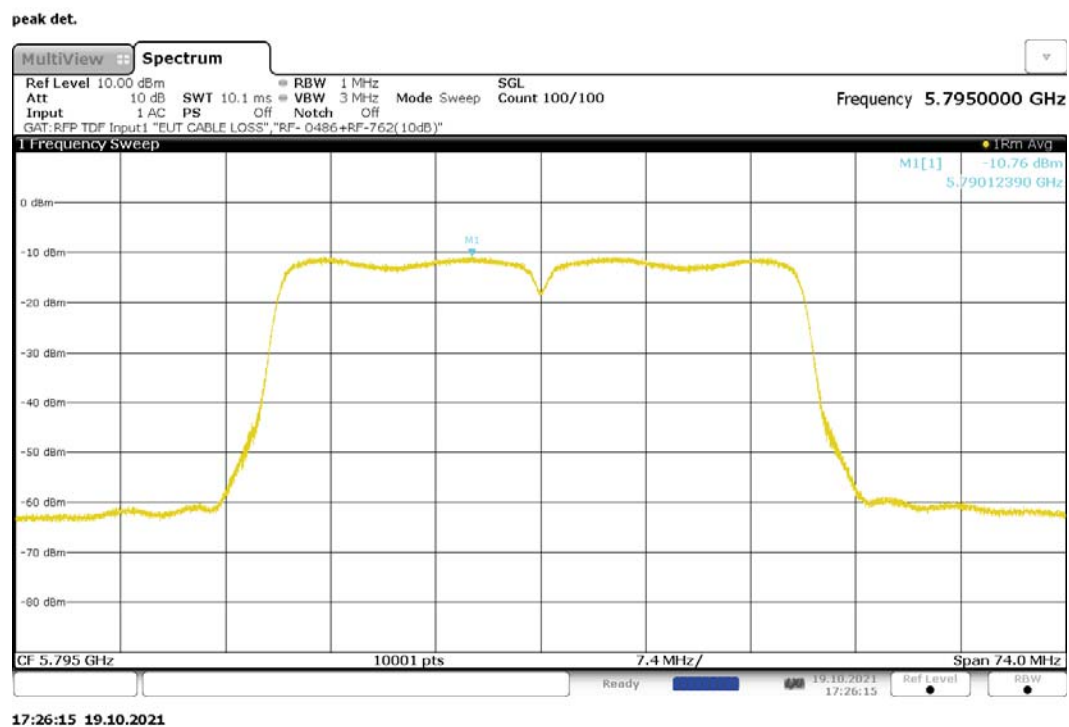
Figure 262: Maximum Power Spectral Density, 802.11ac-40, MIMO, RF1, 5795MHz
