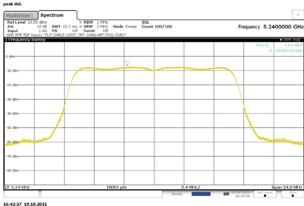
Figure 175: Maximum Power Spectral Density, 802.11n-20, MIMO, RF1, 5240MHz
