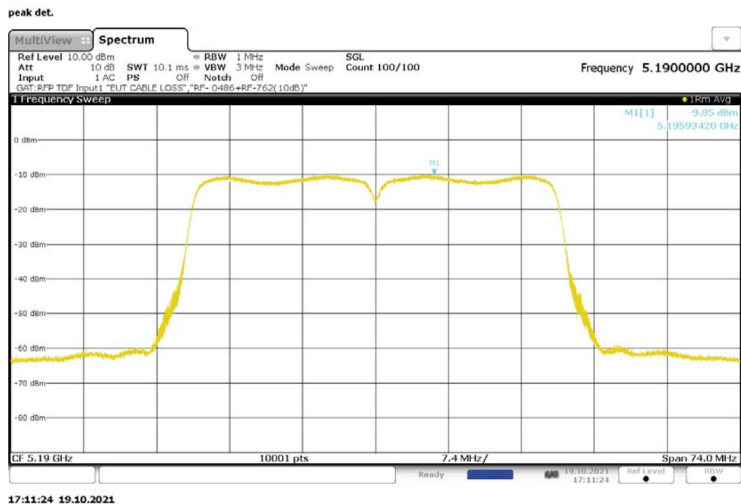
Figure 227: Maximum Power Spectral Density, 802.11n-40, CDD, RF1, 5190MHz
