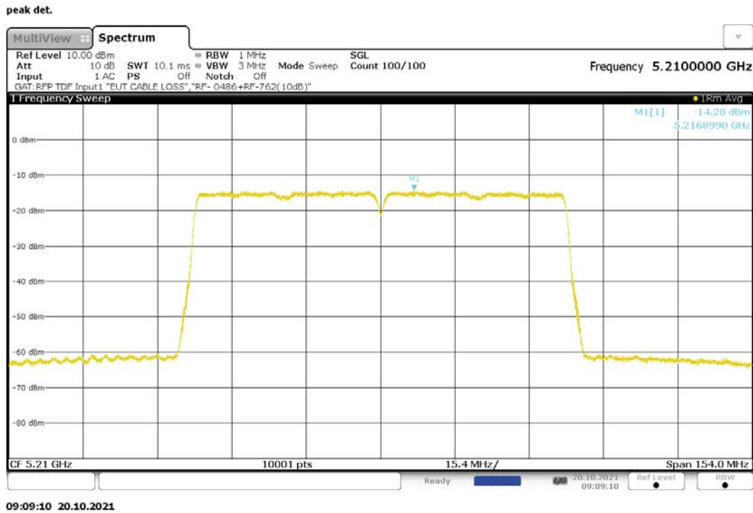
Figure 267: Maximum Power Spectral Density, 802.11ac-80, CDD, RF0, 5210MHz
