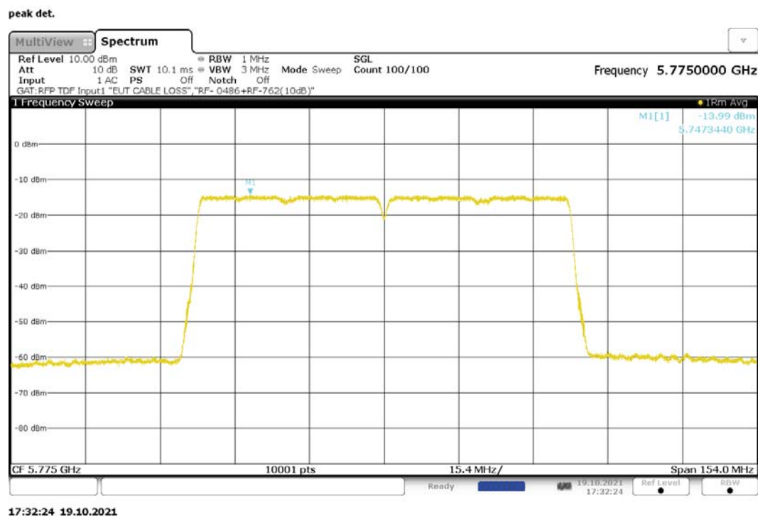
Figure 270: Maximum Power Spectral Density, 802.11ac-80, CDD, RF1, 5775MHz
