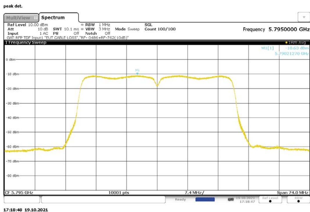
Figure 230: Maximum Power Spectral Density, 802.11n-40, CDD, RF1, 5795MHz
