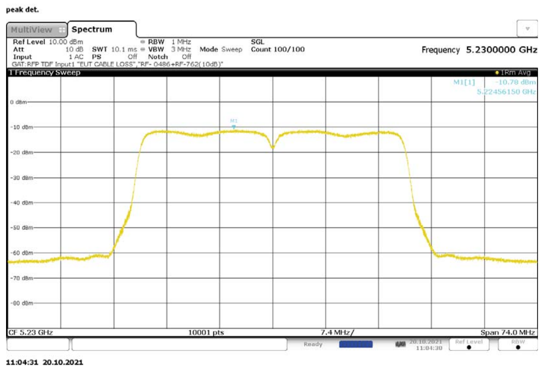
Figure 248: Maximum Power Spectral Density, 802.11ac-40, CDD, RF0, 5230MHz
