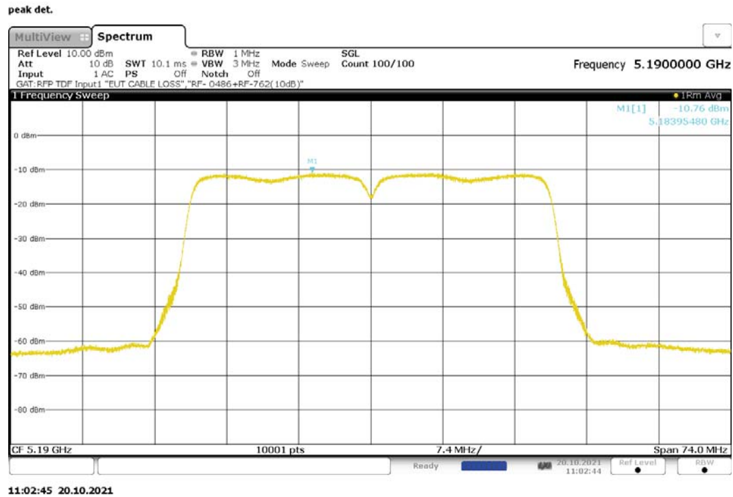
Figure 255: Maximum Power Spectral Density, 802.11ac-40, MIMO, RF0, 5190MHz
