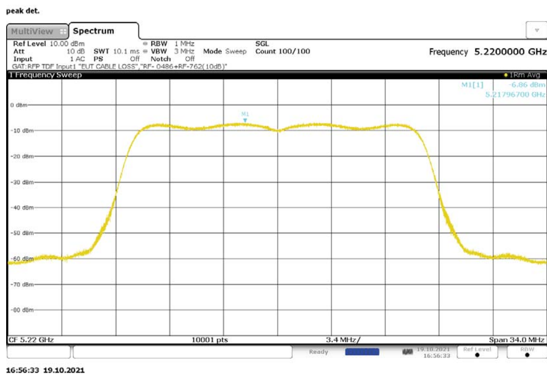
Figure 210: Maximum Power Spectral Density, 802.11ac-20, MIMO, RF1, 5220MHz
