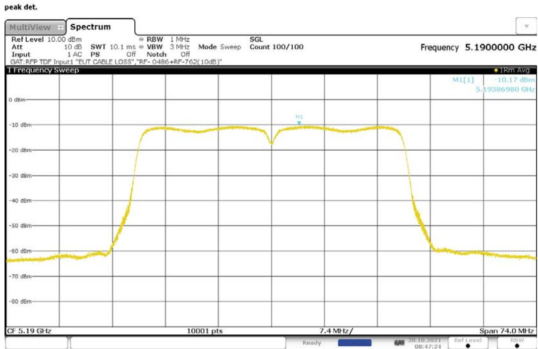
Figure 219: Maximum Power Spectral Density, 802.11n-40, SISO, RF1, 5190MHz
