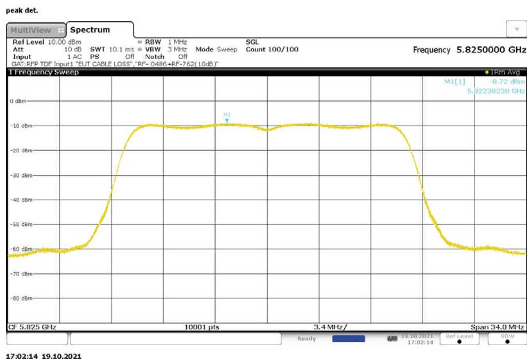
Figure 202: Maximum Power Spectral Density, 802.11ac-20, CDD, RF1, 5825MHz
