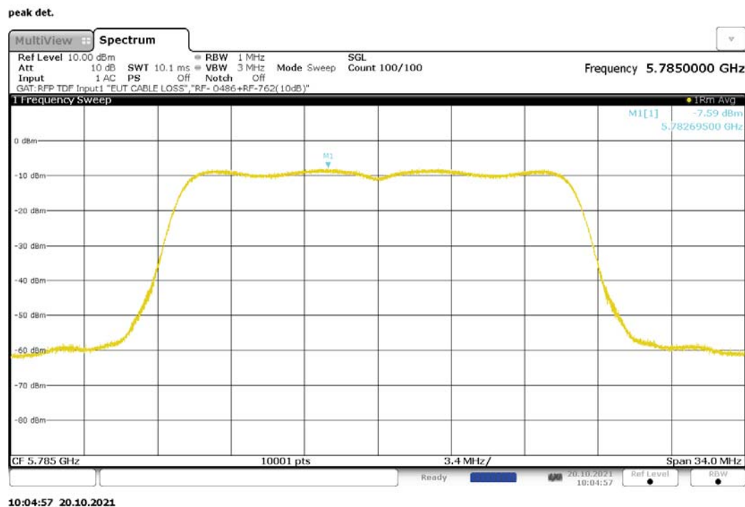
Figure 183: Maximum Power Spectral Density, 802.11ac-20, SISO, RF0, 5785MHz
