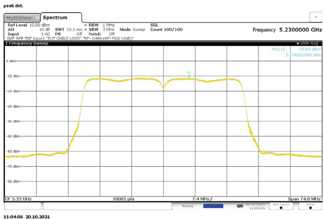
Figure 256: Maximum Power Spectral Density, 802.11ac-40, MIMO, RF0, 5230MHz
