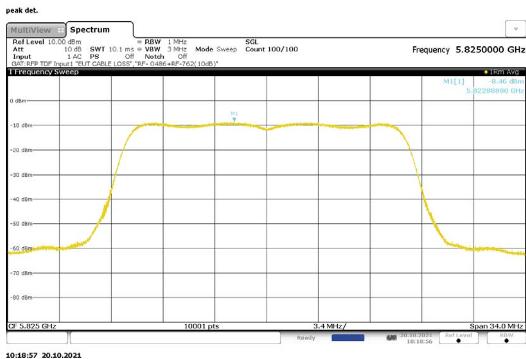
Figure 208: Maximum Power Spectral Density, 802.11ac-20, MIMO, RF0, 5825MHz
