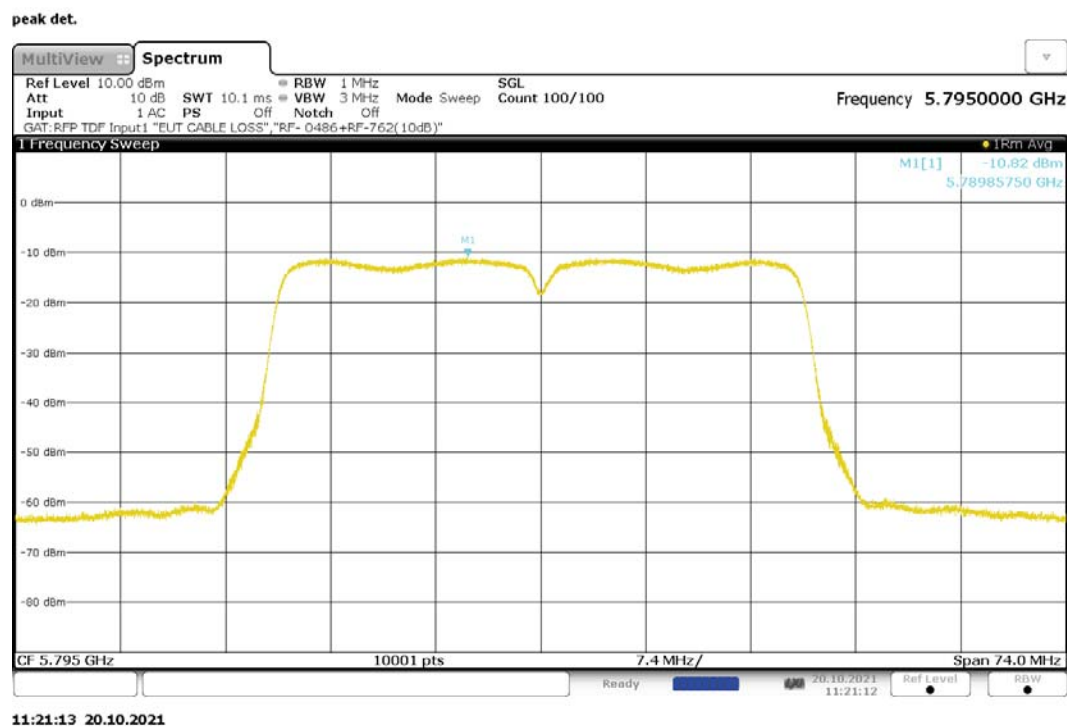
Figure 218: Maximum Power Spectral Density, 802.11n-40, SISO, RF0, 5795MHz
