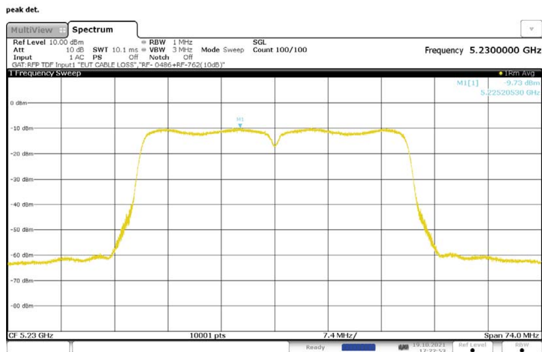
Figure 252: Maximum Power Spectral Density, 802.11ac-40, CDD, RF1, 5230MHz
