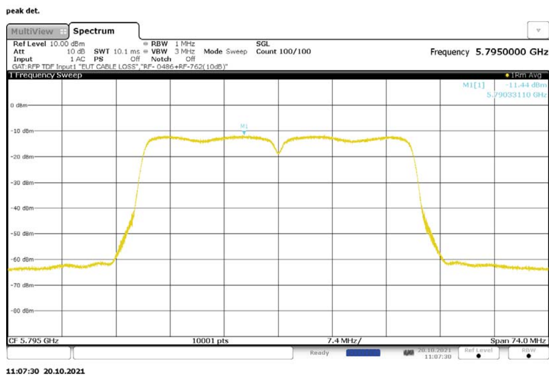
Figure 258: Maximum Power Spectral Density, 802.11ac-40, MIMO, RF0, 5795MHz
