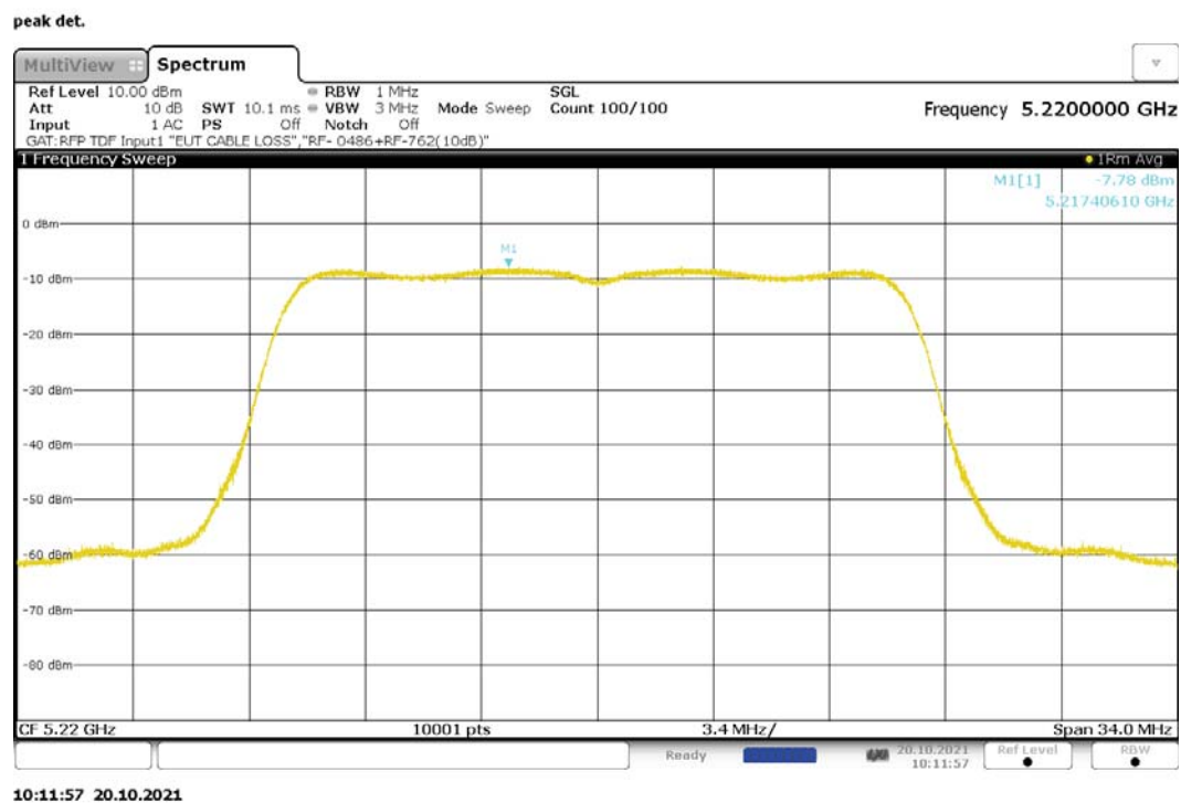
Figure 204: Maximum Power Spectral Density, 802.11ac-20, MIMO, RF0, 5220MHz
