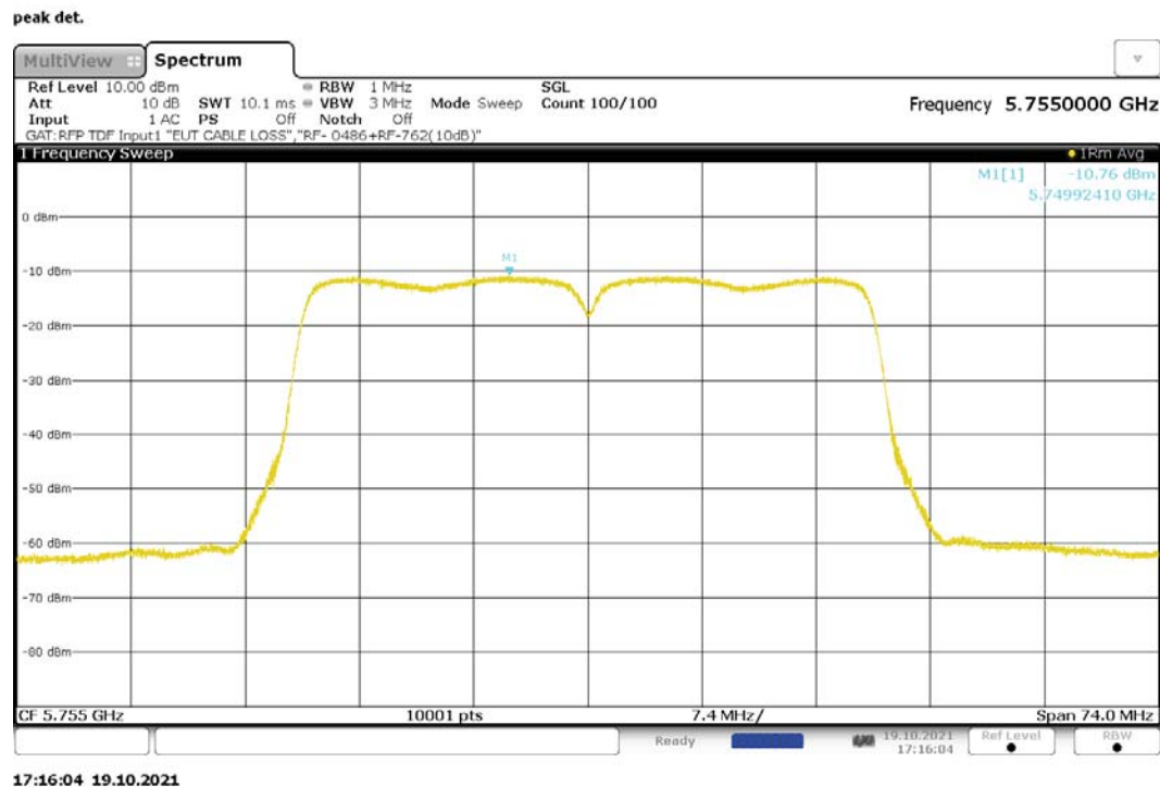
Figure 229: Maximum Power Spectral Density, 802.11n-40, CDD, RF1, 5755MHz
