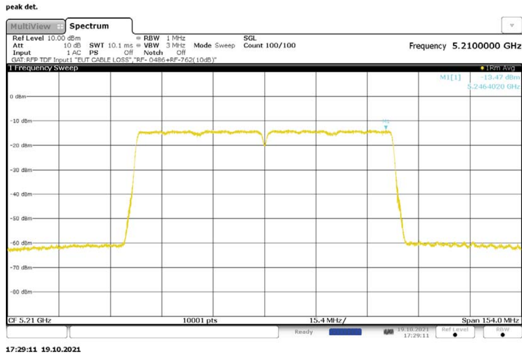
Figure 269: Maximum Power Spectral Density, 802.11ac-80, CDD, RF1, 5210MHz
