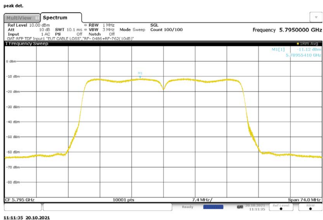
Figure 242: Maximum Power Spectral Density, 802.11ac-40, SISO, RF0, 5795MHz
