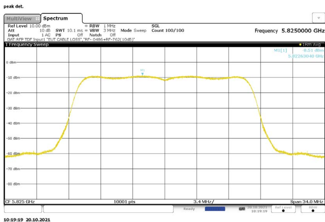
Figure 196: Maximum Power Spectral Density, 802.11ac-20, CDD, RF0, 5825MHz
