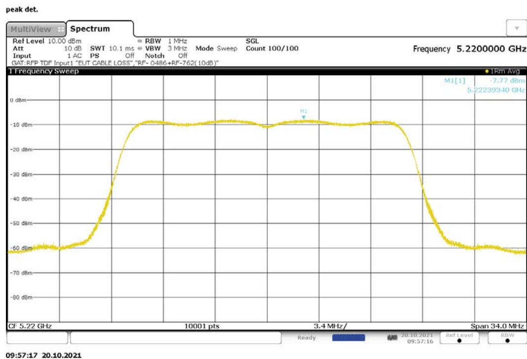
Figure 180: Maximum Power Spectral Density, 802.11ac-20, SISO, RF0, 5220MHz
