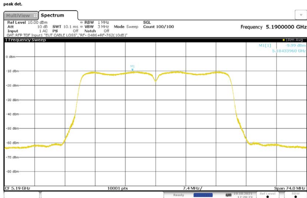
Figure 251: Maximum Power Spectral Density, 802.11ac-40, CDD, RF1, 5190MHz
