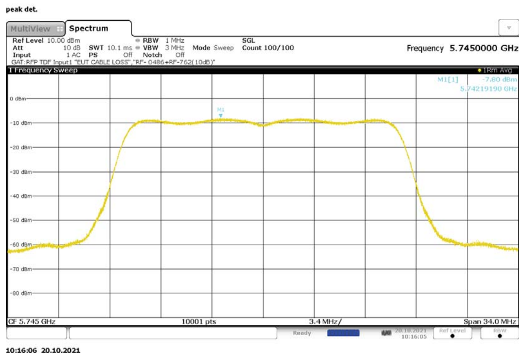
Figure 194: Maximum Power Spectral Density, 802.11ac-20, CDD, RF0, 5745MHz
