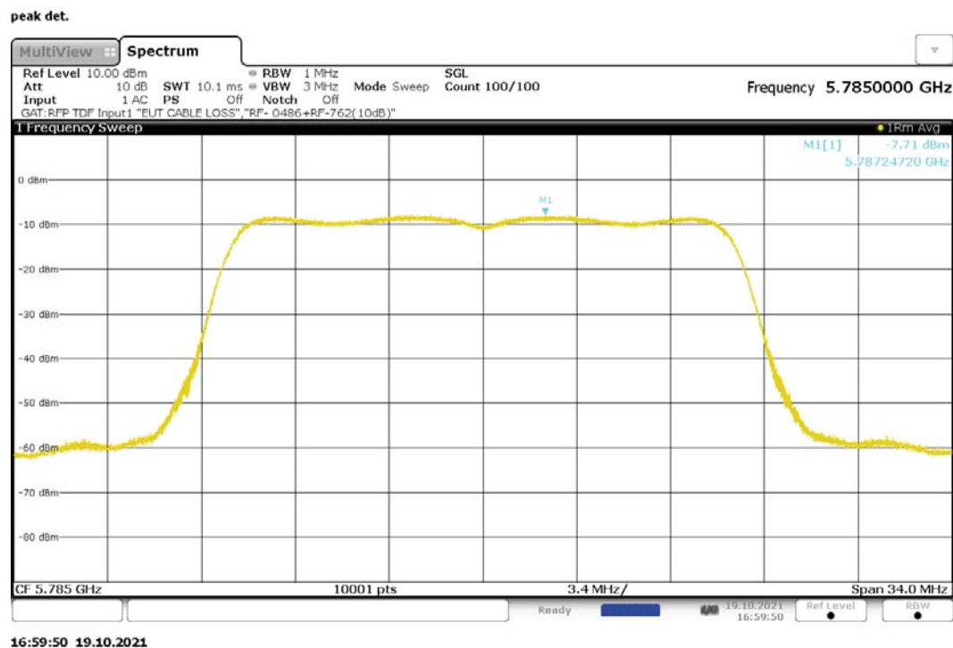
Figure 201: Maximum Power Spectral Density, 802.11ac-20, CDD, RF1, 5785MHz
