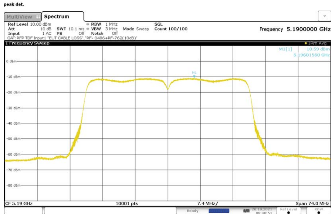
Figure 243: Maximum Power Spectral Density, 802.11ac-40, SISO, RF1, 5190MHz
