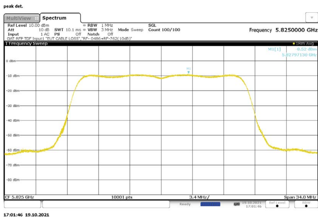
Figure 214: Maximum Power Spectral Density, 802.11ac-20, MIMO, RF1, 5825MHz
