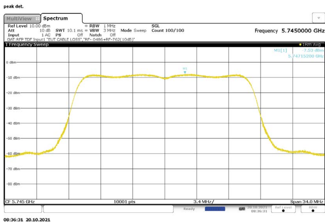
Figure 188: Maximum Power Spectral Density, 802.11ac-20, SISO, RF1, 5745MHz
