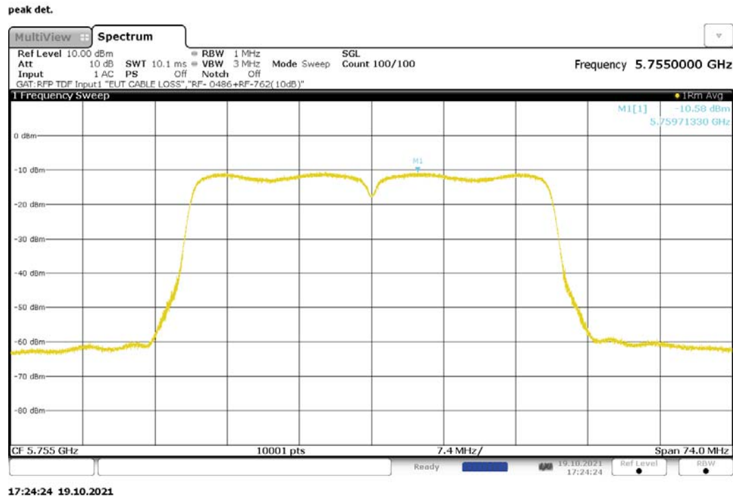
Figure 253: Maximum Power Spectral Density, 802.11ac-40, CDD, RF1, 5755MHz
