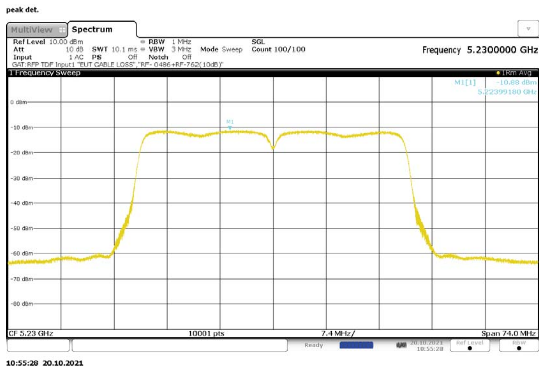
Figure 232: Maximum Power Spectral Density, 802.11n-40, MIMO, RF0, 5230MHz
