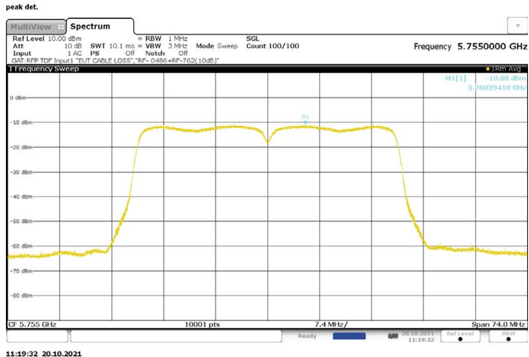
Figure 217: Maximum Power Spectral Density, 802.11n-40, SISO, RF0, 5755MHz
