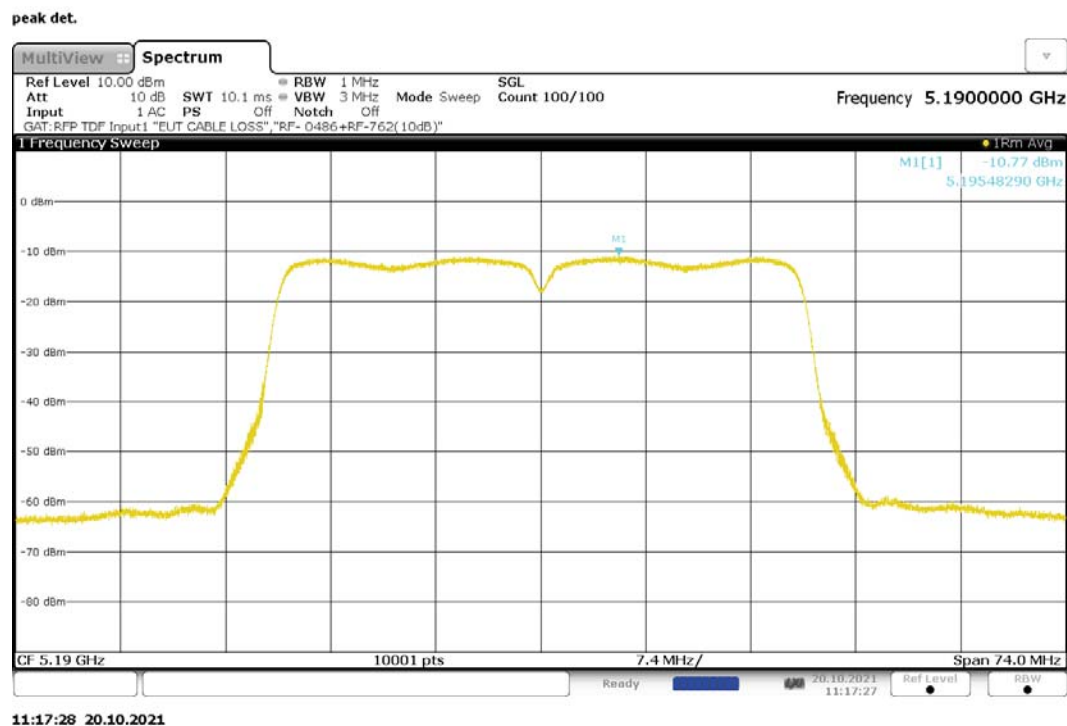
Figure 215: Maximum Power Spectral Density, 802.11n-40, SISO, RF0, 5190MHz
