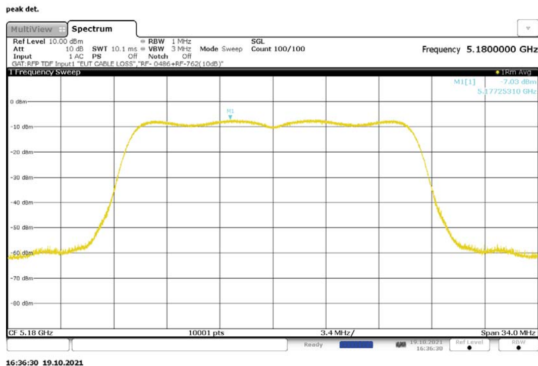
Figure 173: Maximum Power Spectral Density, 802.11n-20, MIMO, RF1, 5180MHz
