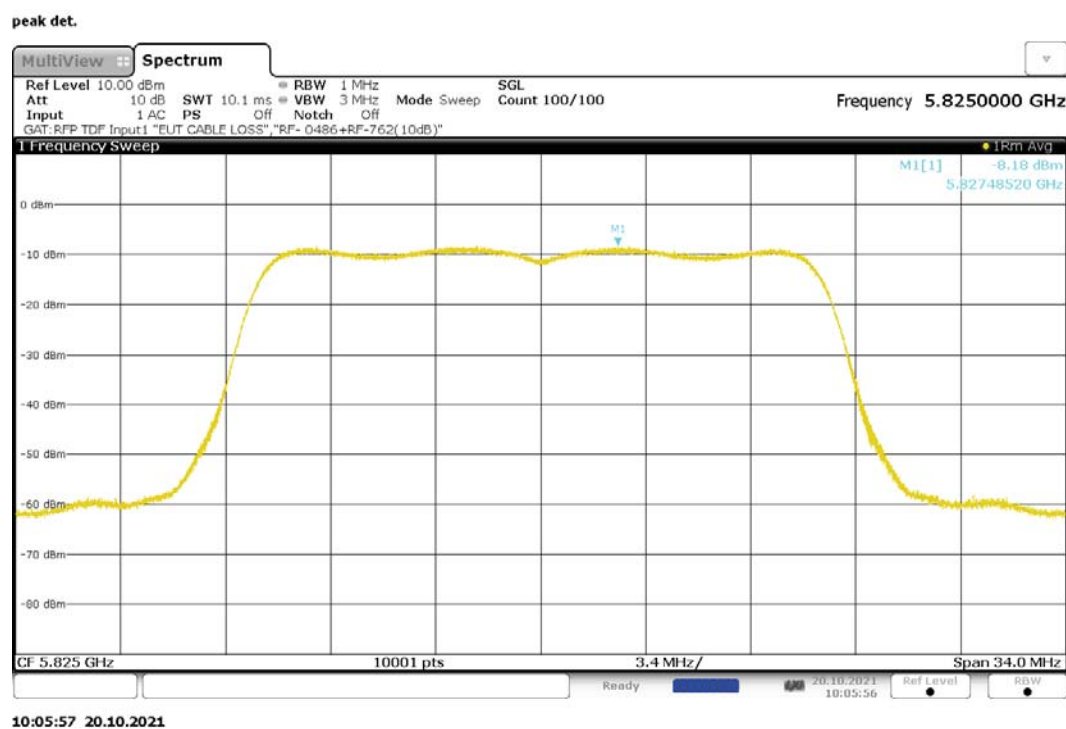
Figure 184: Maximum Power Spectral Density, 802.11ac-20, SISO, RF0, 5825MHz
