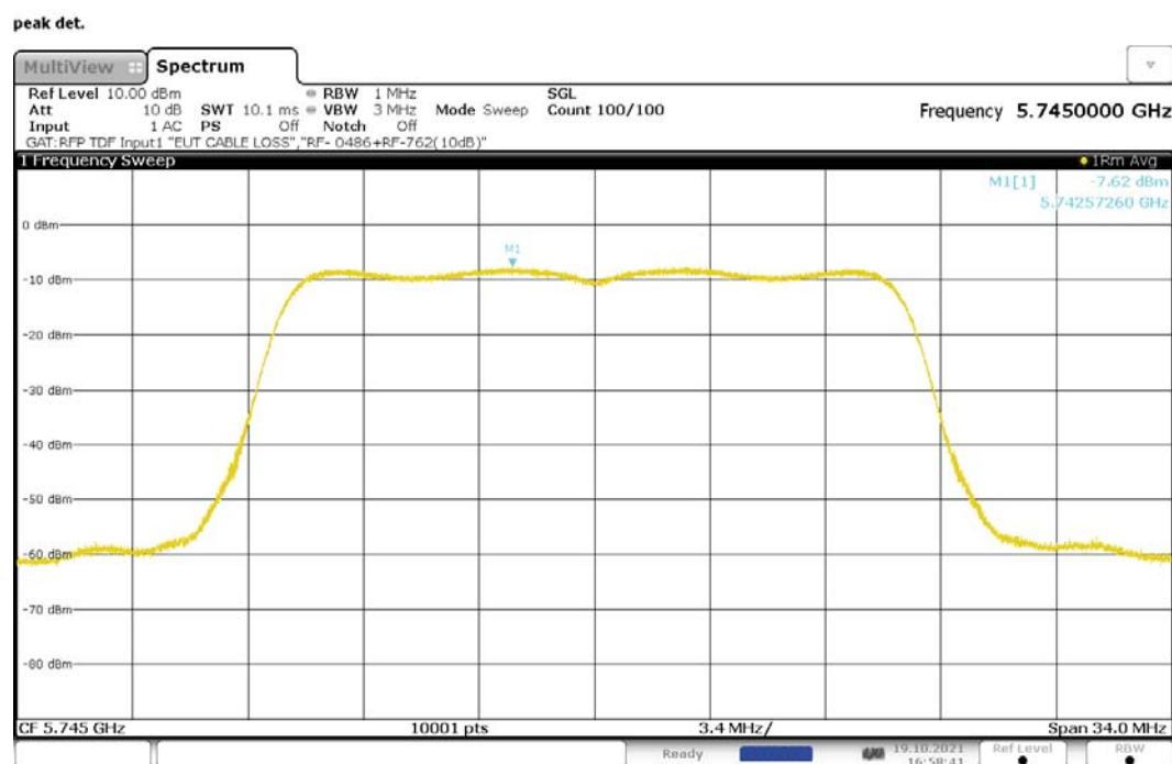
Figure 200: Maximum Power Spectral Density, 802.11ac-20, CDD, RF1, 5745MHz
