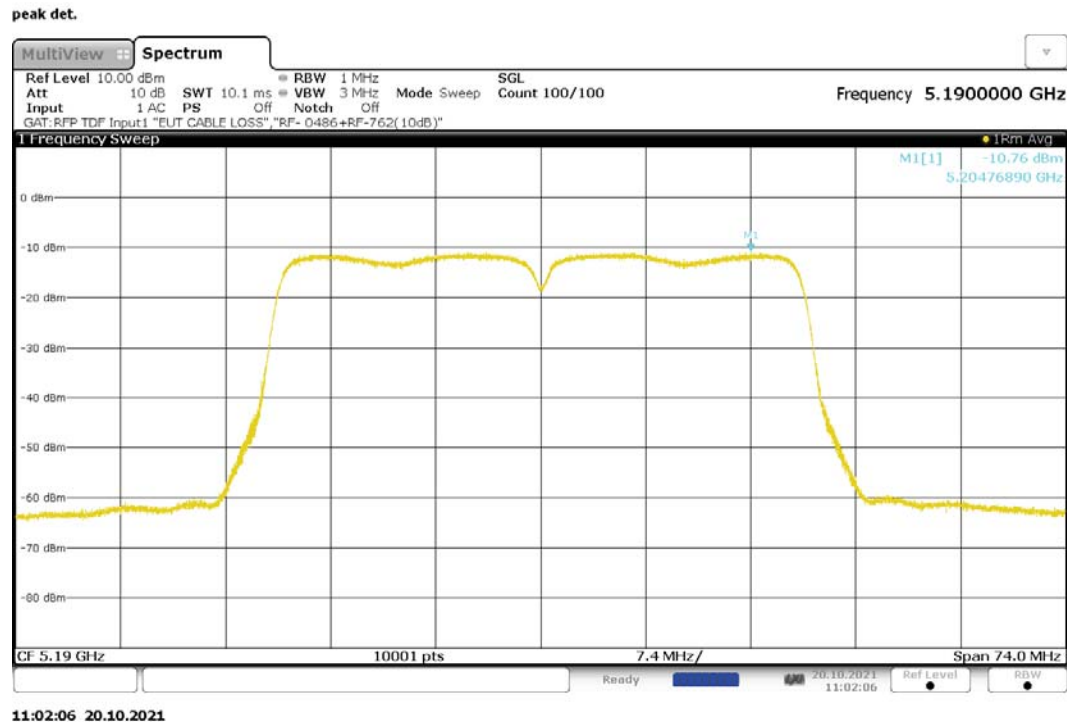
Figure 247: Maximum Power Spectral Density, 802.11ac-40, CDD, RF0, 5190MHz
