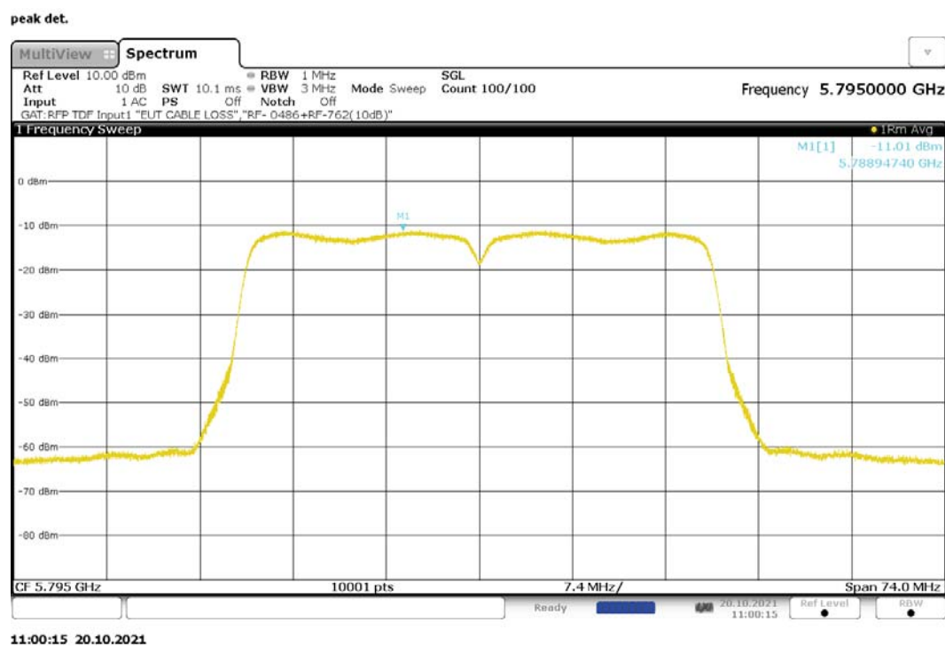
Figure 234: Maximum Power Spectral Density, 802.11n-40, MIMO, RF0, 5795MHz
