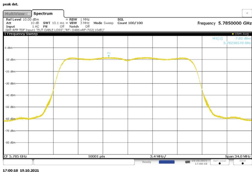
Figure 213: Maximum Power Spectral Density, 802.11ac-20, MIMO, RF1, 5785MHz
