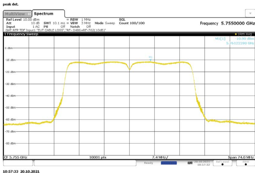
Figure 233: Maximum Power Spectral Density, 802.11n-40, MIMO, RF0, 5755MHz
