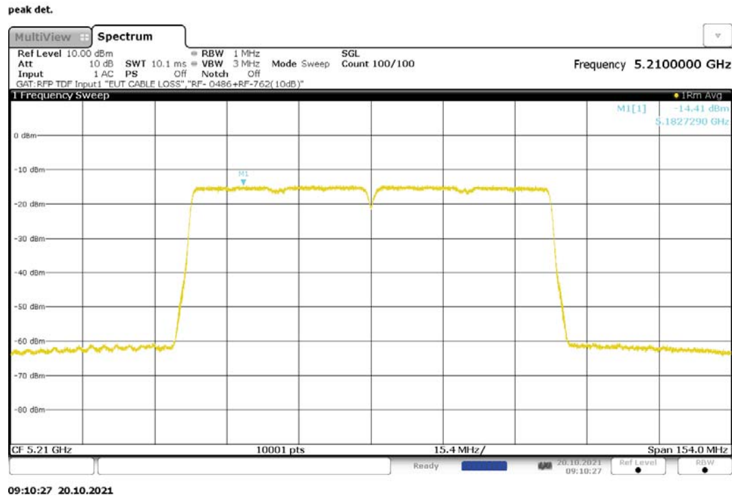
Figure 263: Maximum Power Spectral Density, 802.11ac-80, SISO, RF0, 5210MHz
