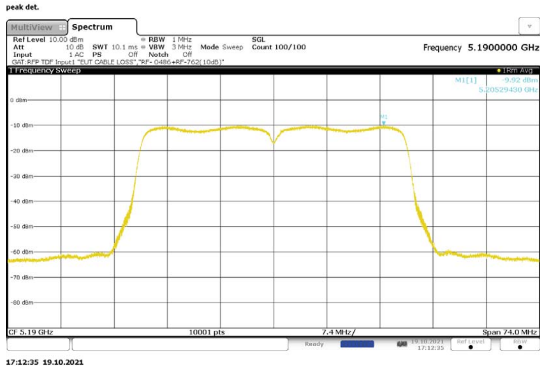
Figure 231: Maximum Power Spectral Density, 802.11n-40, MIMO, RF0, 5190MHz
