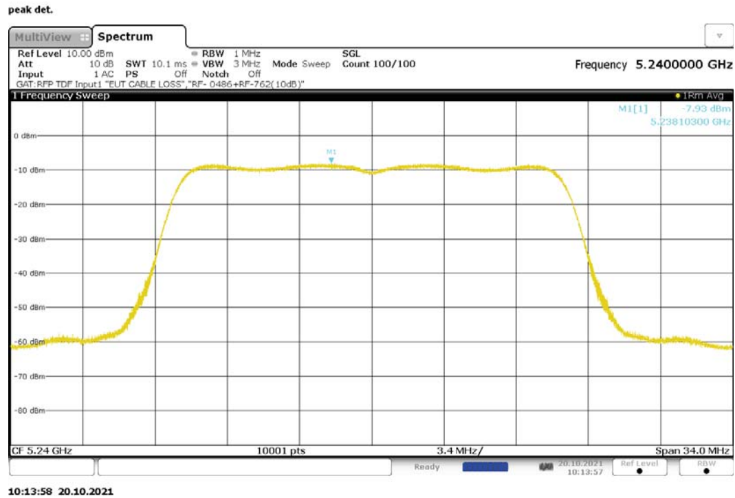
Figure 205: Maximum Power Spectral Density, 802.11ac-20, MIMO, RF0, 5240MHz
