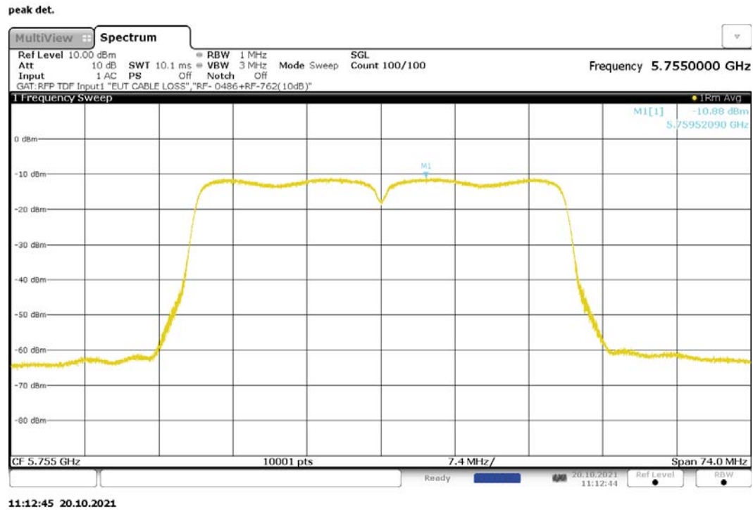
Figure 241: Maximum Power Spectral Density, 802.11ac-40, SISO, RF0, 5755MHz
