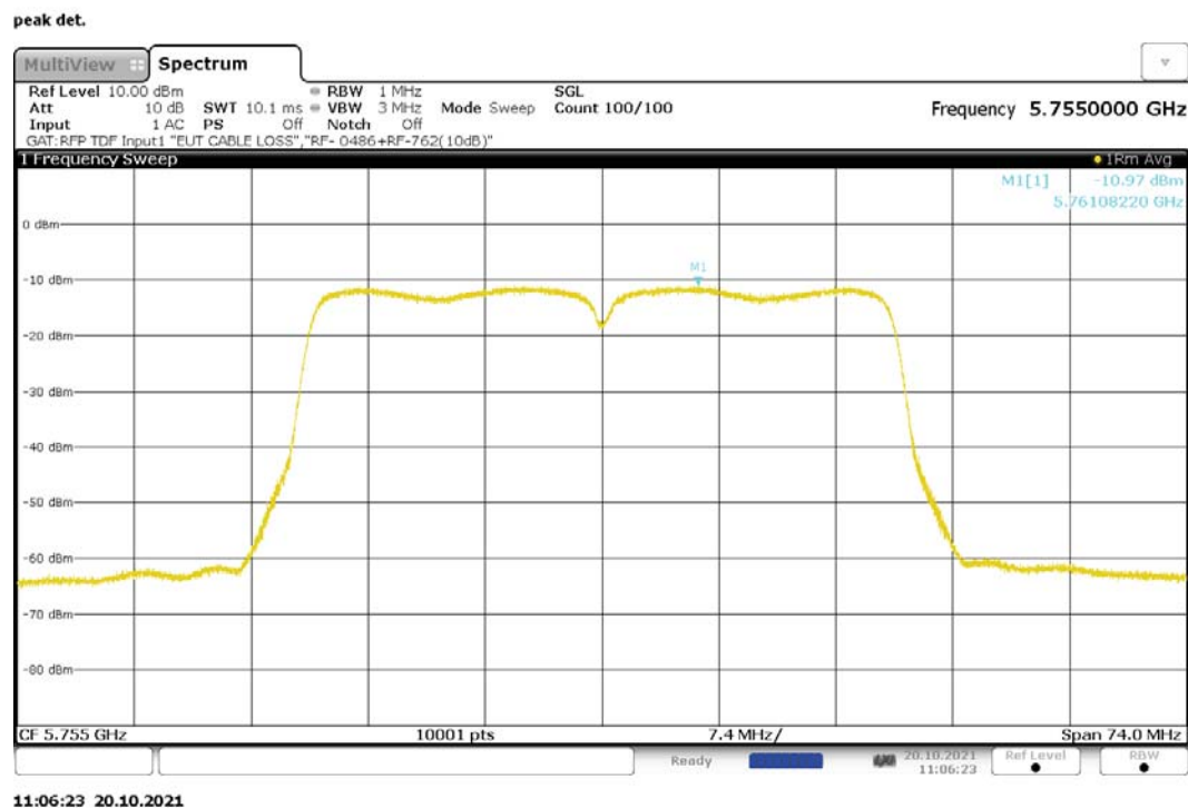
Figure 257: Maximum Power Spectral Density, 802.11ac-40, MIMO, RF0, 5755MHz
