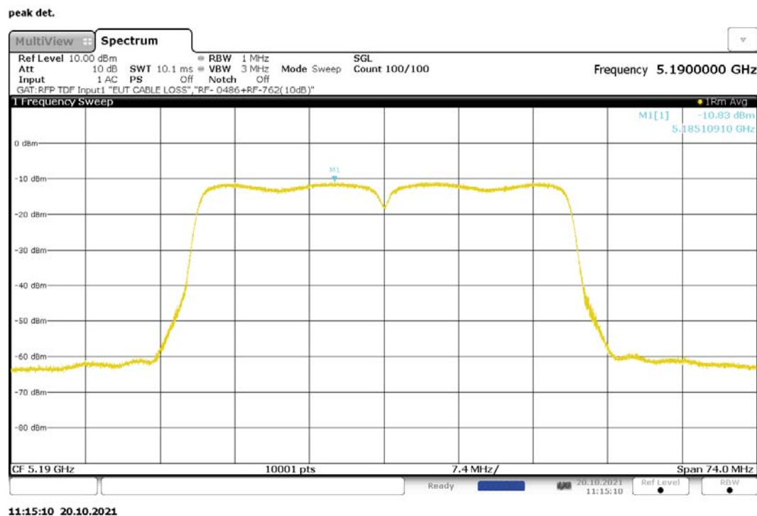
Figure 239: Maximum Power Spectral Density, 802.11ac-40, SISO, RF0, 5190MHz
