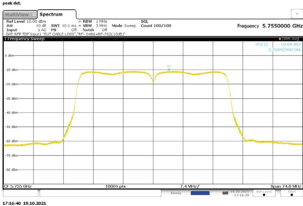
Figure 237: Maximum Power Spectral Density, 802.11n-40, MIMO, RF1, 5755MHz
