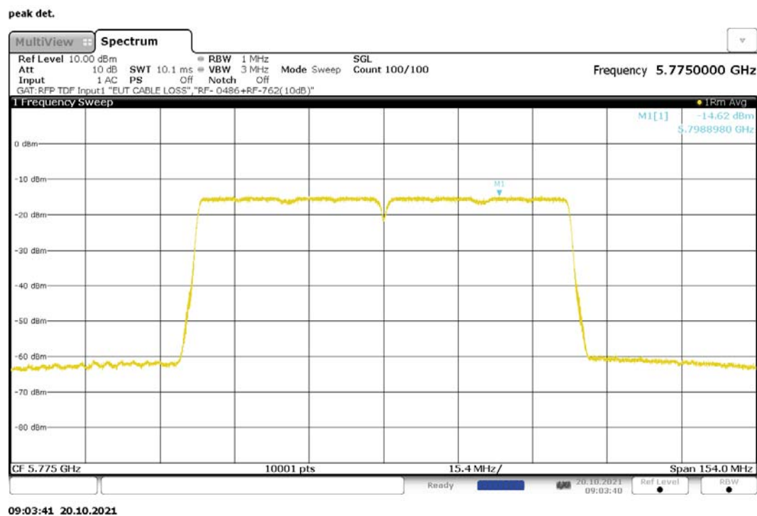
Figure 264: Maximum Power Spectral Density, 802.11ac-80, SISO, RF0, 5775MHz
