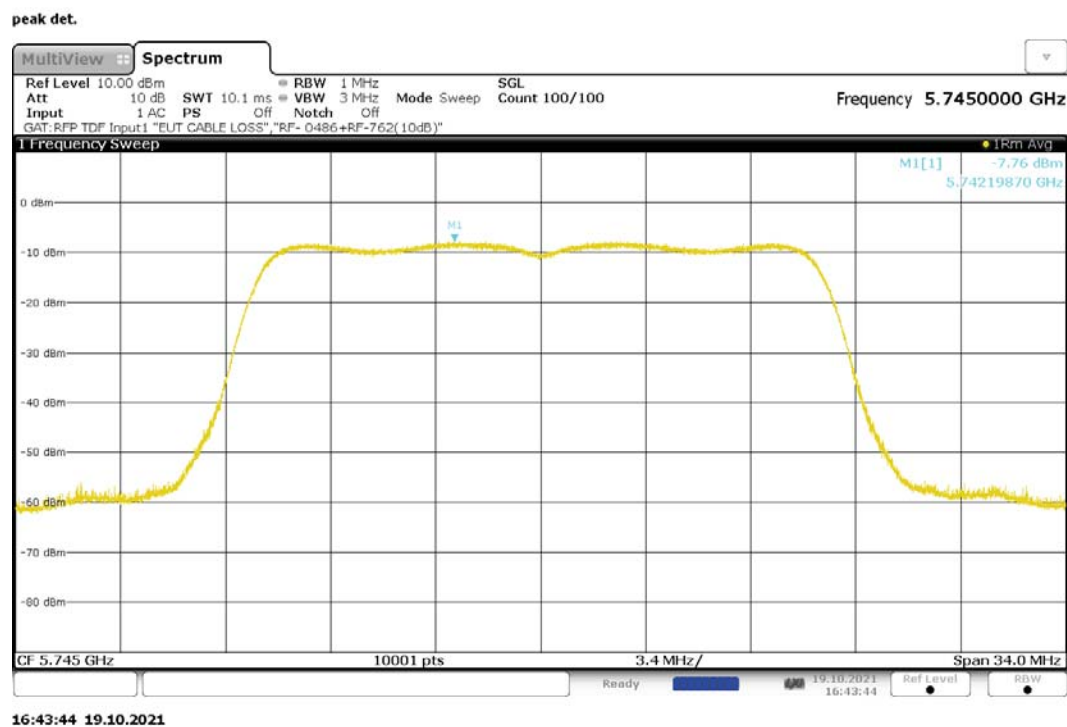
Figure 176: Maximum Power Spectral Density, 802.11n-20, MIMO, RF1, 5745MHz
