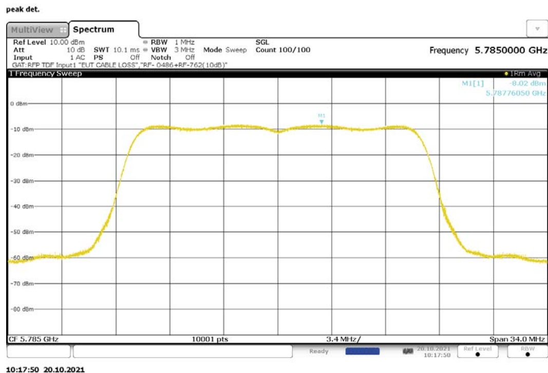
Figure 207: Maximum Power Spectral Density, 802.11ac-20, MIMO, RF0, 5785MHz
