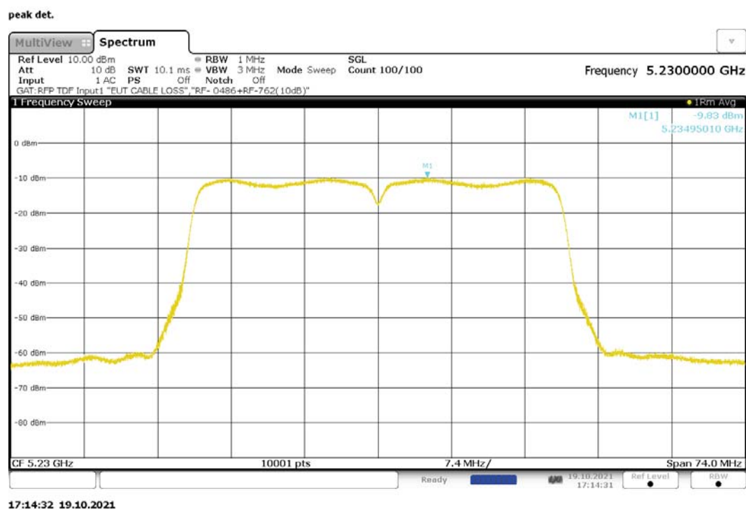
Figure 228: Maximum Power Spectral Density, 802.11n-40, CDD, RF1, 5230MHz
