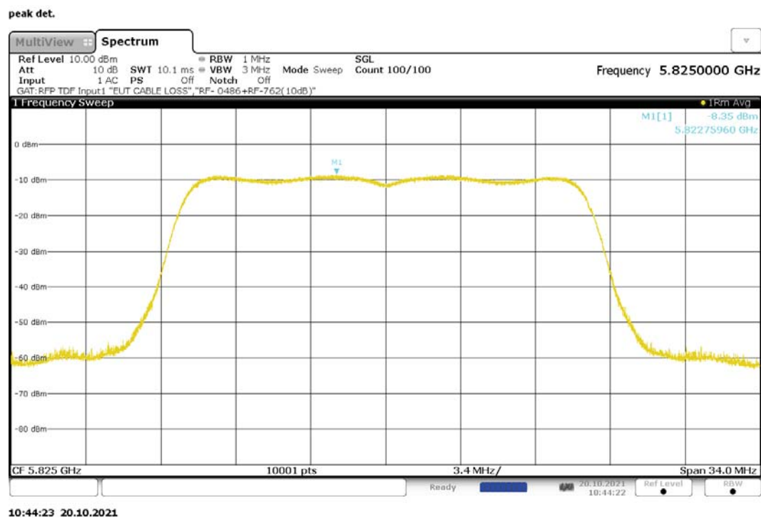
Figure 172: Maximum Power Spectral Density, 802.11n-20, MIMO, RF0, 5825MHz
