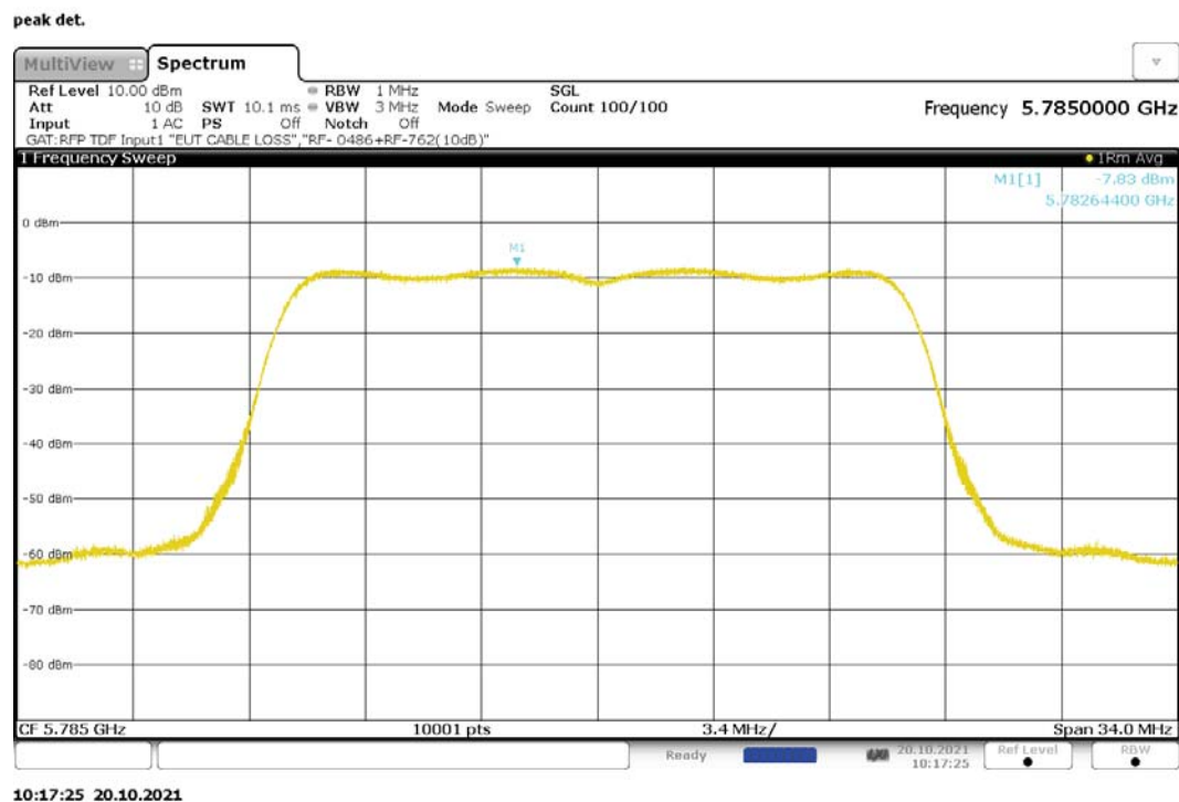
Figure 195: Maximum Power Spectral Density, 802.11ac-20, CDD, RF0, 5785MHz
