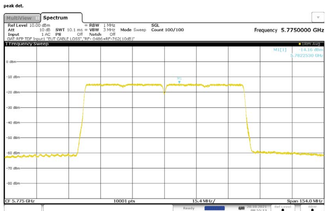
Figure 266: Maximum Power Spectral Density, 802.11ac-80, SISO, RF1, 5775MHz
