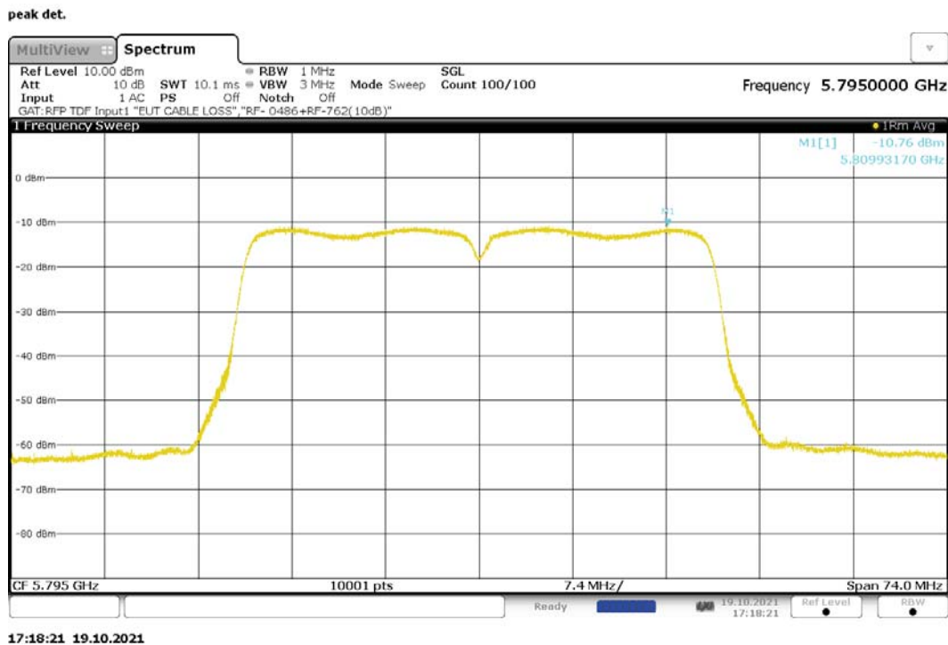
Figure 238: Maximum Power Spectral Density, 802.11n-40, MIMO, RF1, 5795MHz
