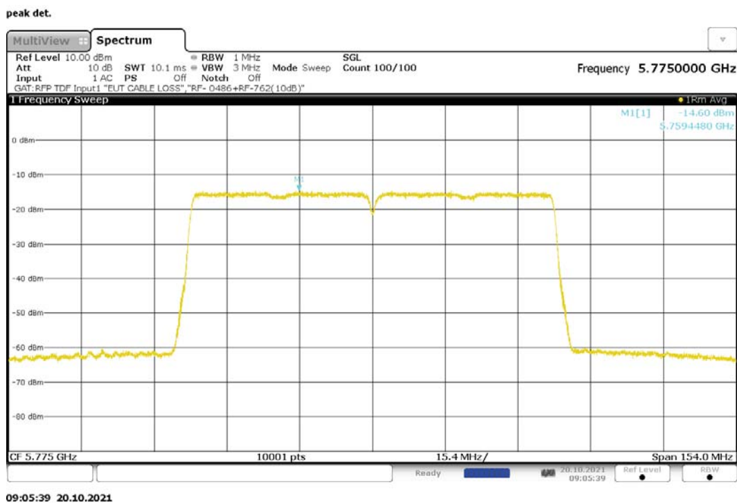
Figure 268: Maximum Power Spectral Density, 802.11ac-80, CDD, RF0, 5775MHz
