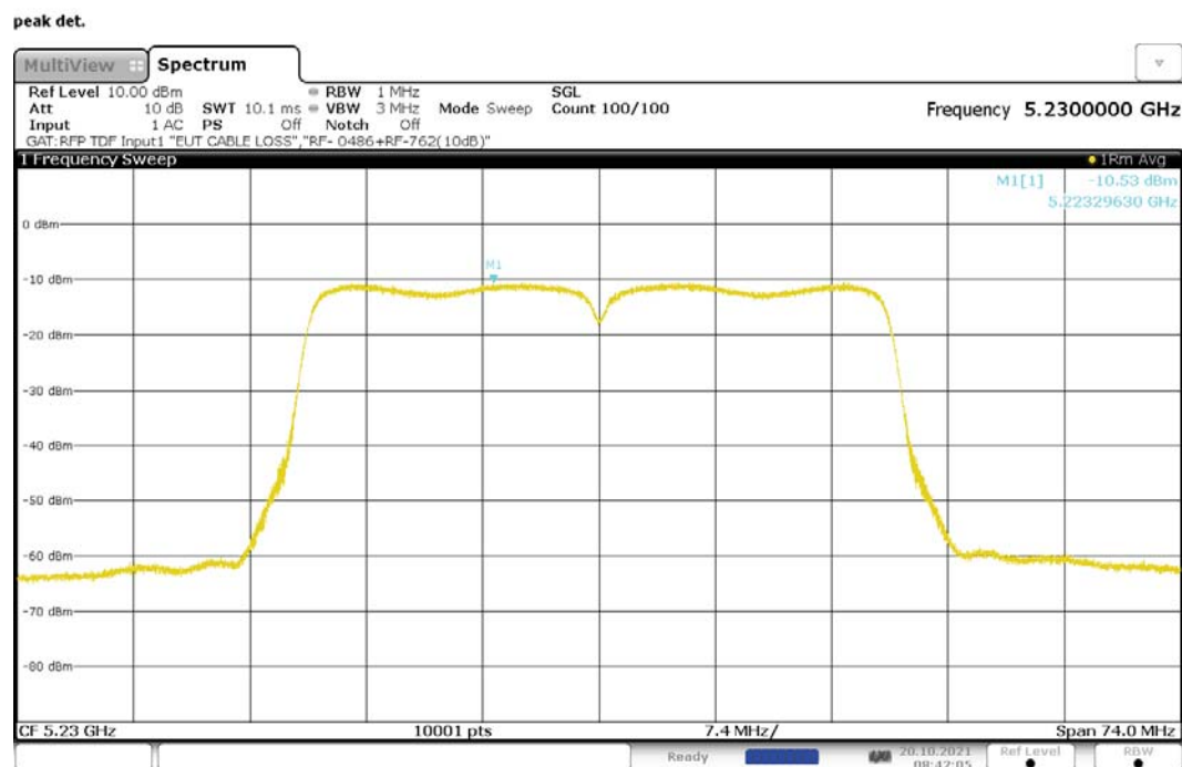
Figure 244: Maximum Power Spectral Density, 802.11ac-40, SISO, RF1, 5230MHz
