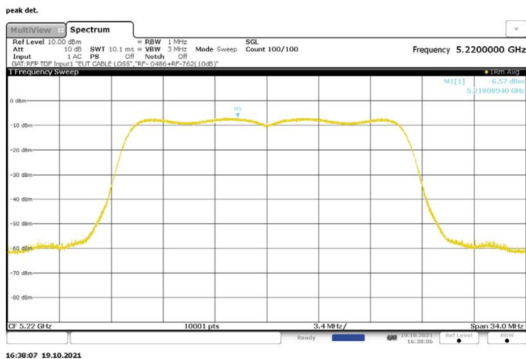
Figure 174: Maximum Power Spectral Density, 802.11n-20, MIMO, RF1, 5220MHz
