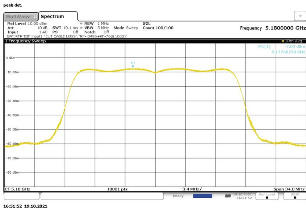
Figure 209: Maximum Power Spectral Density, 802.11ac-20, MIMO, RF1, 5180MHz
