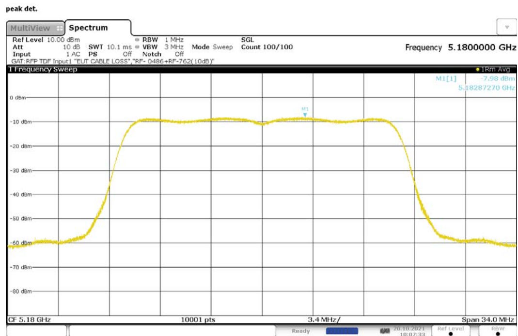
Figure 191: Maximum Power Spectral Density, 802.11ac-20, CDD, RF0, 5180MHz
