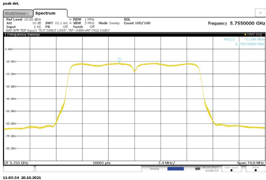
Figure 249: Maximum Power Spectral Density, 802.11ac-40, CDD, RF0, 5755MHz
