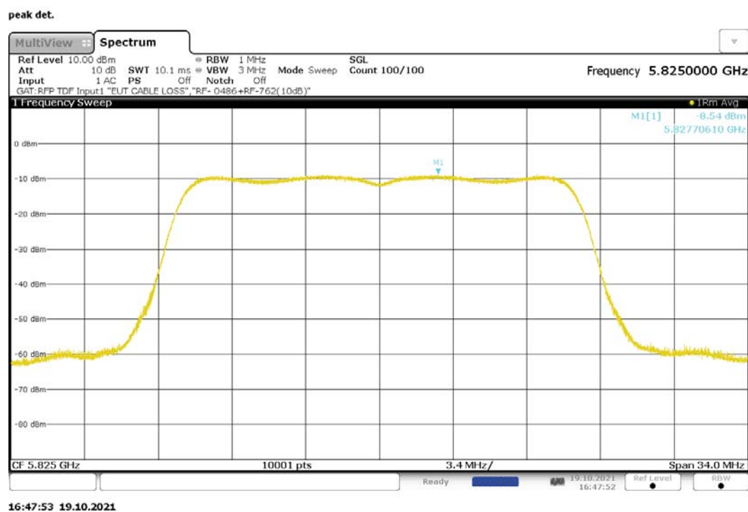
Figure 178: Maximum Power Spectral Density, 802.11n-20, MIMO, RF1, 5825MHz
