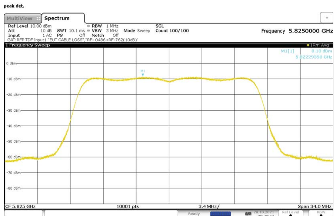
Figure 190: Maximum Power Spectral Density, 802.11ac-20, SISO, RF1, 5825MHz
