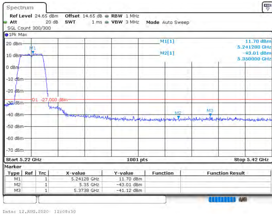
Band Edge NVNT 802.11ac20 5240MHz High Ant 1
