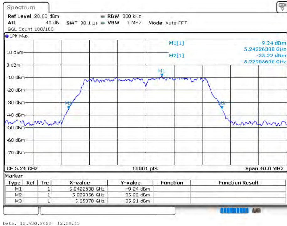
-26 dB BW NVNT 802.11ac20 5240MHz Ant 1
