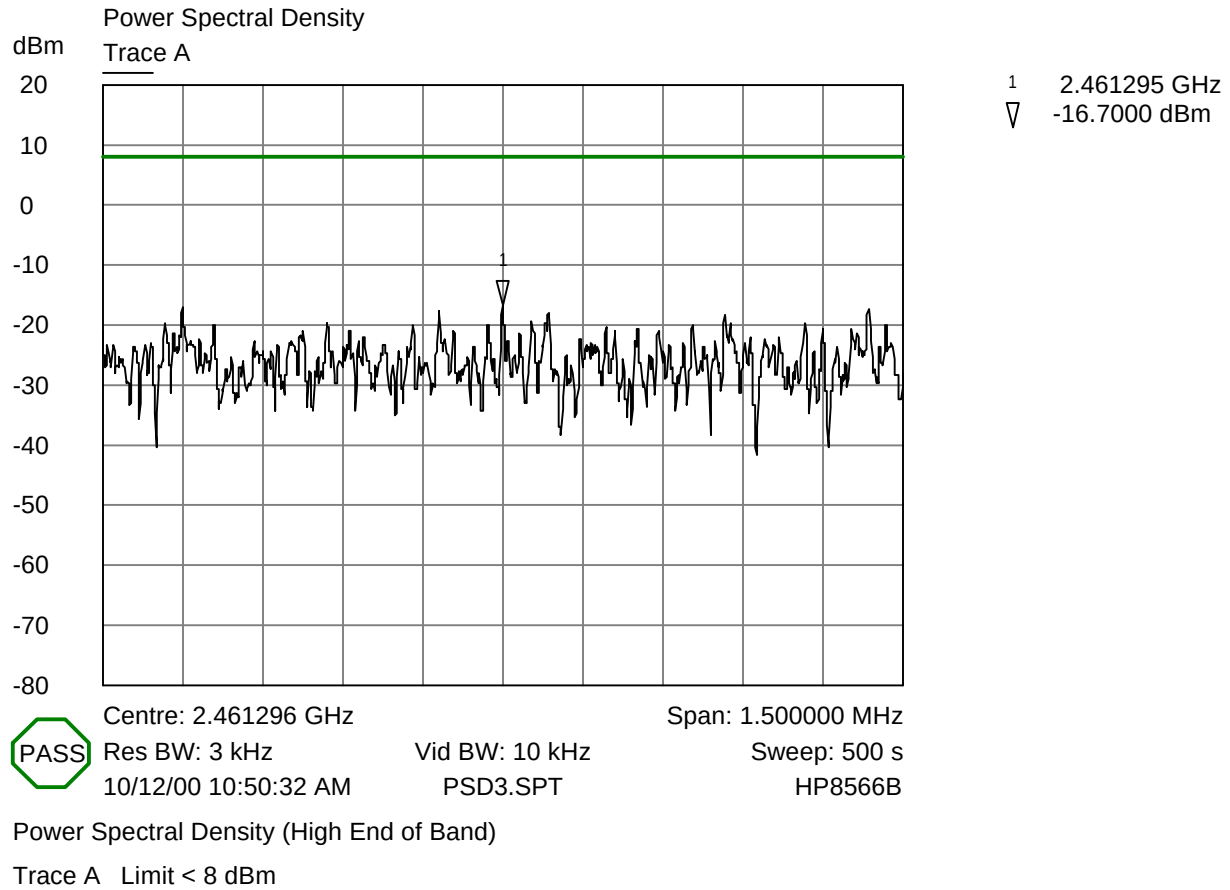
Power Spectral Density Plot (High Channel)
