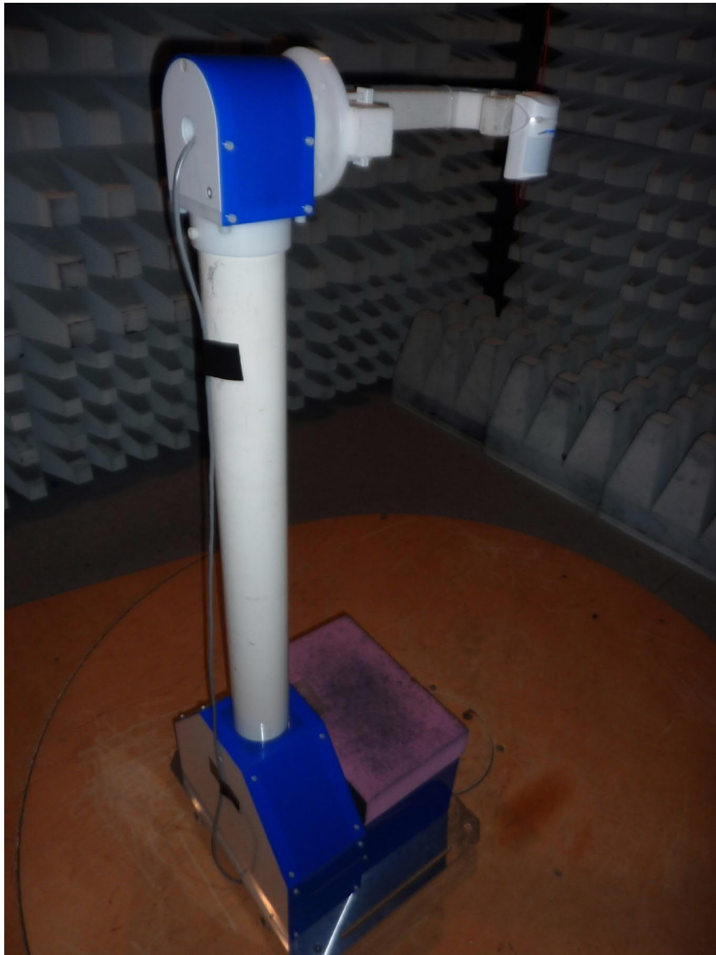
Test setup fully anechoic chamber
