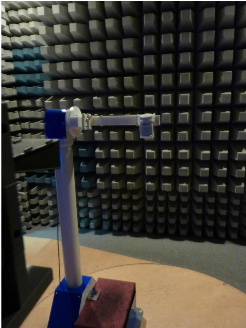
Test setup semi anechoic chamber (12 GHz to 40 GHz)
