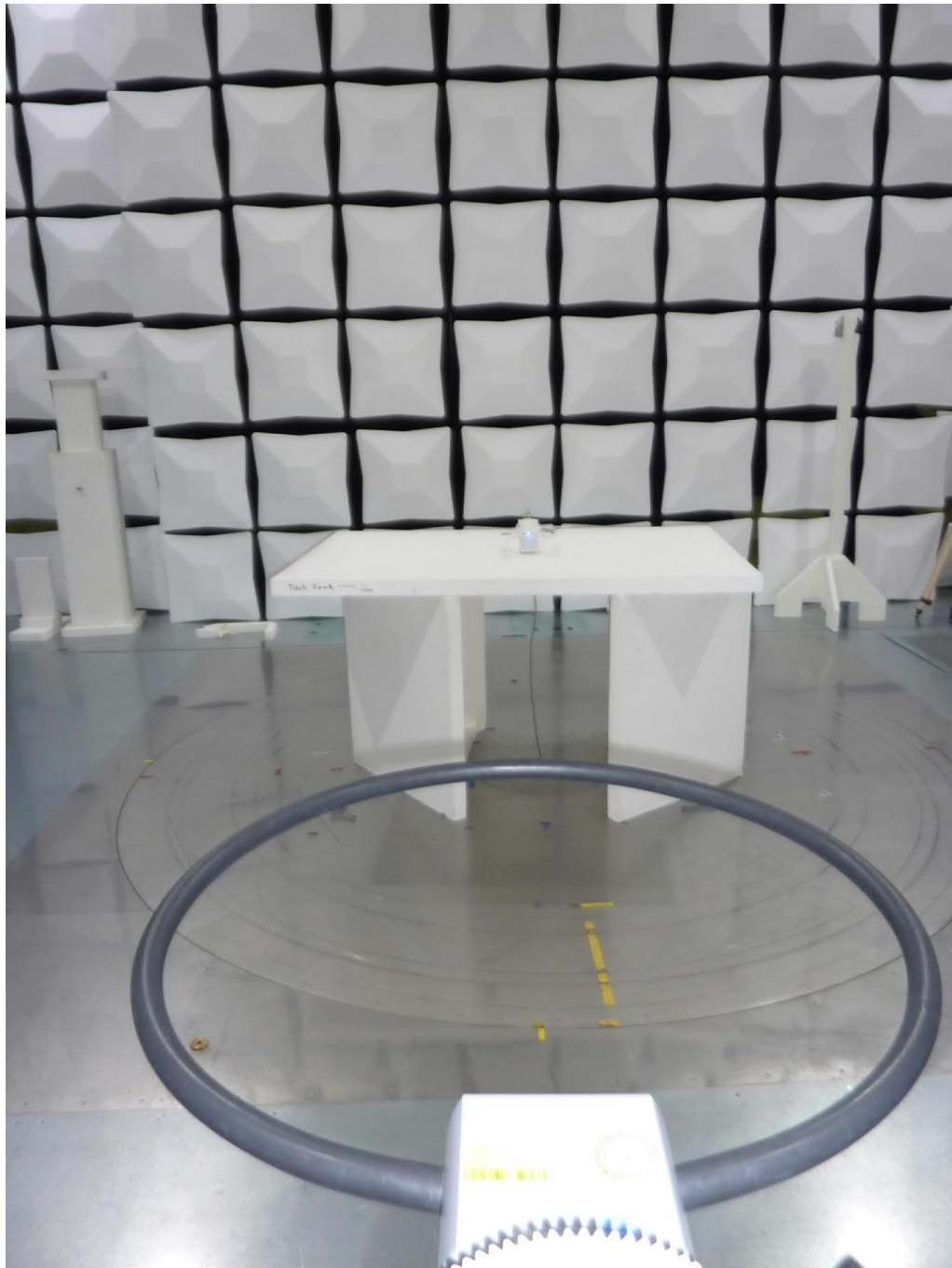
Test setup semi anechoic chamber (10 MHz to 30 MHz)
