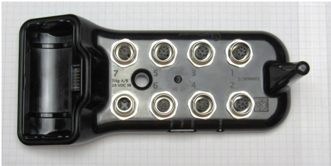
“HUB Top” with all internal parts installed. Grid pattern is 5mm.
