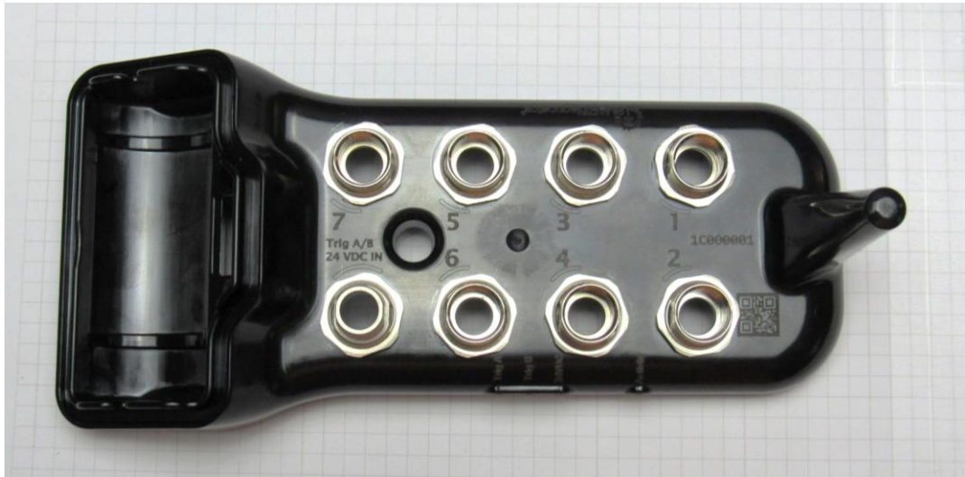
“HUB Top” without internal PCBs. Grid pattern is 5mm.
