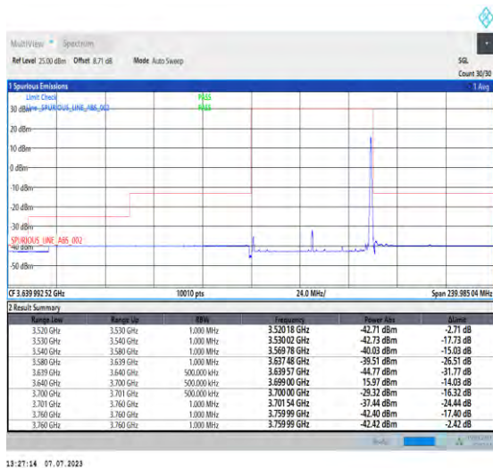
1-N48-PC3-30-60-H-2-DFT-PI2BPSK-Edge_1RB_Right-t-1@161-Ant3-1--PASS-see graph
