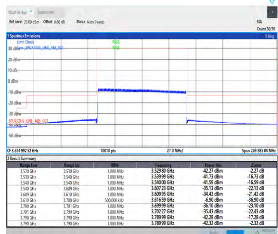
1-N48-PC3-30-90-H-6-CP-QPSK-Outer_Full-245@0-Ant3-1--PASS-see graph
