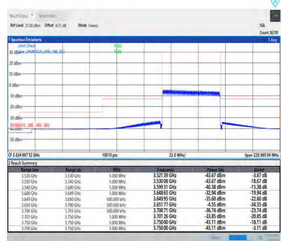
1-N48-PC3-30-50-H-6-CP-QPSK-Outer_Full-133@0-Ant3-1--PASS-see graph
