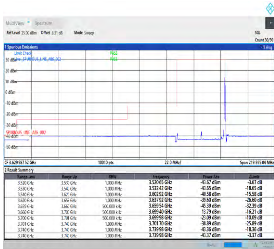
1-N48-PC3-30-40-H-2-DFT-PI2BPSK-Edge_1RB_Right-1@105-Ant3-1--PASS-see graph
