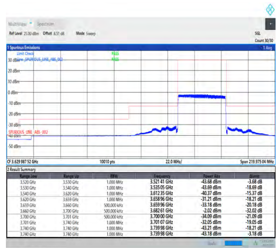
1-N48-PC3-30-40-H-3-DFT-PI2BPSK-Outer_Full-100@0-Ant3-1--PASS-see graph
