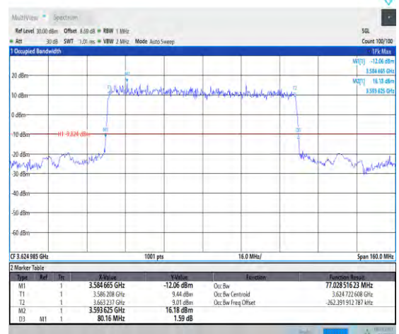
1-N48-PC3-30-80-M-2-DFT-PI2BPSK-Outer_Full-100 @0-Ant3-77.029-80.160-≤80-PASS
