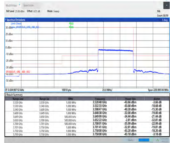
1-N48-PC3-30-50-H-3-DFT-PI2BPSK-Outer_Full-128@0-Ant3-1--PASS-see graph
