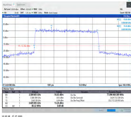
1-N48-PC3-30-80-M-3-DFT-16QAM-Outer_Full-100 @0-Ant3-77.096-80.320-≤80-PASS
