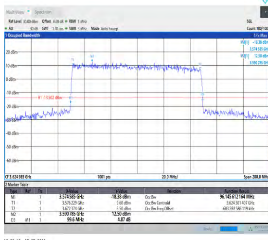
1-N48-PC3-30-100-M-3-DFT-16QAM-Outter_Full-51 @0-Ant3-96.146-99.600-≤100-PASS
