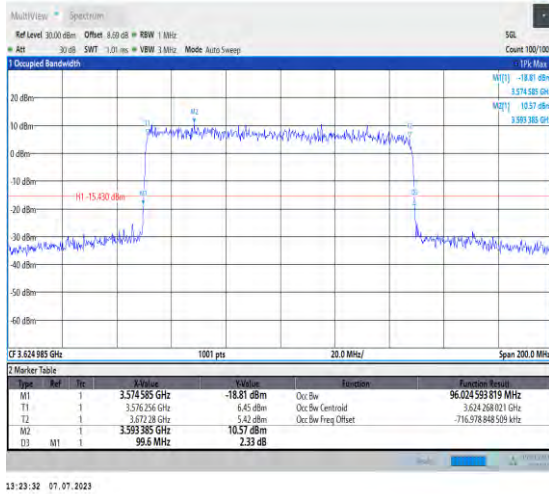
1-N48-PC3-30-100-M-5-DFT-256QAM-Outer_Full-51 @0-Ant3-96.025-99.600-≤100-PASS
