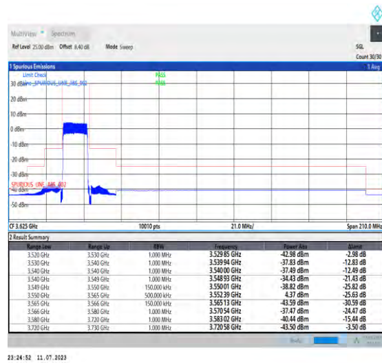
1-N48-PC3-30-15-L-3-DFT-PI2BPSK-Outer_Full-36@0Ant3-1--PASS-see graph
