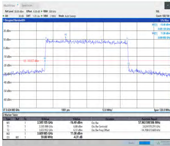
1-N48-PC3-30-60-M-4-DFT-64QAM-Outer_Full-162 @0-Ant3-57.964-59.880-≤60-PASS
