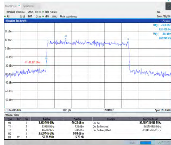
1-N48-PC3-30-60-M-3-DFT-16QAM-Outet_Full-162 @0-Ant3-57.739-59.760-≤60-PASS
