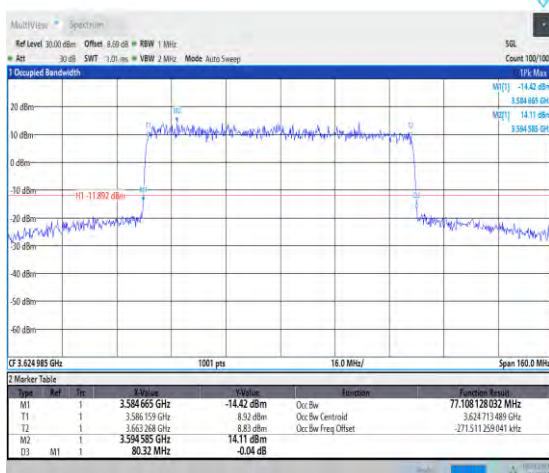
1-N48-PC3-30-80-M-1-DFT-QPSK-Outer_Full-100 @0-Ant3-77.108-80.320-≤80-PASS
