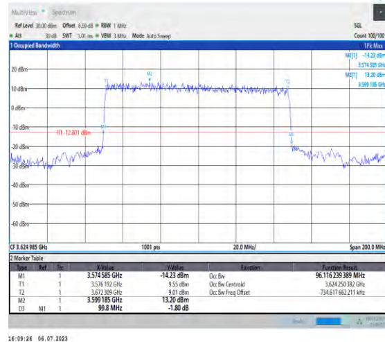
1-N48-PC3-30-100-M-2-DFT-PI2BPSK-Outter_Full-51 @0-Ant3-96.116-99.800-≤100-PASS
