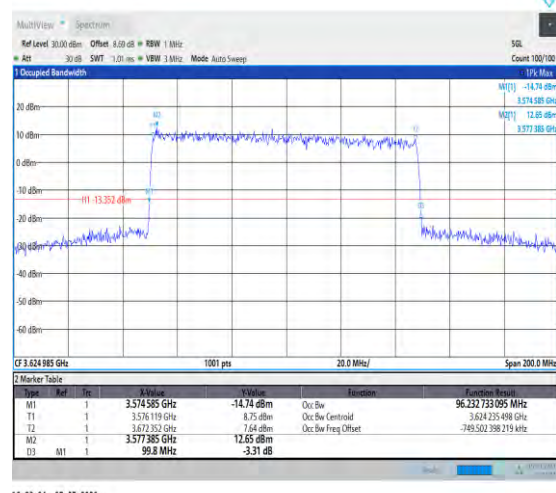
1-N48-PC3-30-100-M-4-DFT-64QAM-Outter_Full-51 @0-Ant3-96.233-99.800-≤100-PASS
