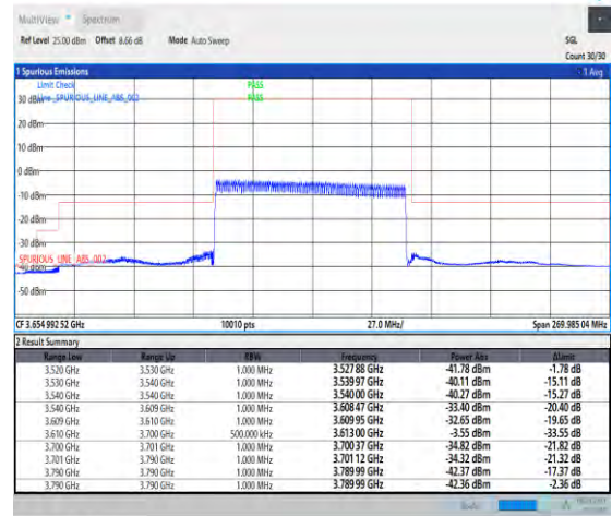
1-N48-PC3-30-90-H-3-DFT-PI2BPSK-Outer_Full-240@0-Ant3-1--PASS-see graph
