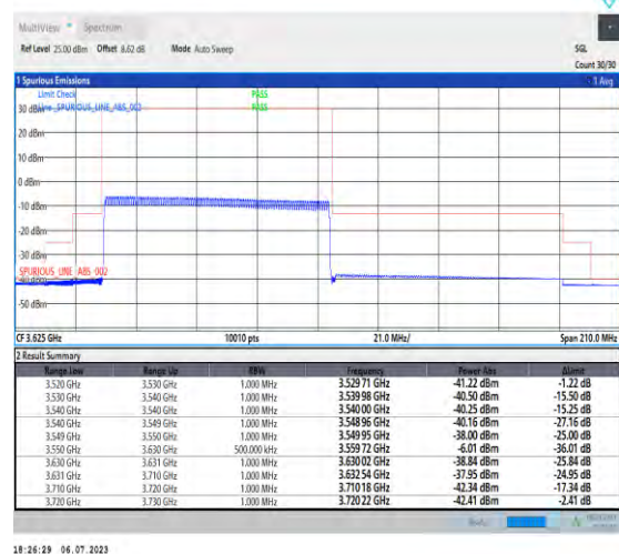
1-N48-PC3-30-80-L-6-CP-QPSK-Outer_Full-217@0-Ant3-1--PASS-see graph
