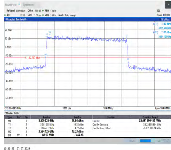
1-N48-PC3-30-90-M-3-DFT-16QAM-Out_240 @0-Ant3-85.682-88.920-≤90-PASS
