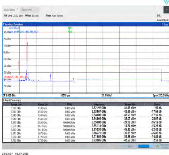
1-N48-PC3-30-60-L-4-CP-QPSK-Edge_1RB_Left-1@ 0-Ant3-1--PASS-see graph
