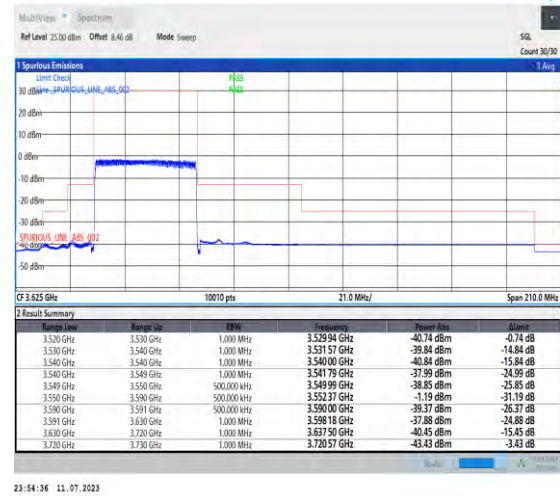
1-N48-PC3-30-40-L-3-DFT-PI2BPSK-Outer_Full-10 0@0-Ant3-1--PASS-see graph
