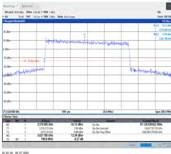
1-N48-PC3-30-100-M-7-CP-16QAM-Outer_Full-273 @0-Ant3-97.127-100.800-≤100-PASS
