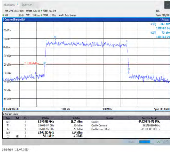
1-N48-PC3-30-50-M-9-CP-256QAM-Outet_Full-133 @0-Ant3-47.921-50.100-≤50-PASS
