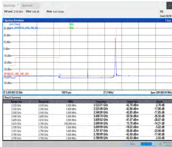
1-N48-PC3-30-90-H-2-DFT-PI2BPSK-Edge_1RB_Right-t-1@244-Ant3-1--PASS-see graph
