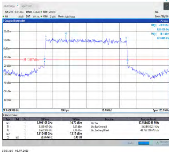
1-N48-PC3-30-60-M-2-DFT-PI2BPSK-Outet_Full-162 @0-Ant3-57.939-59.760-≤60-PASS
