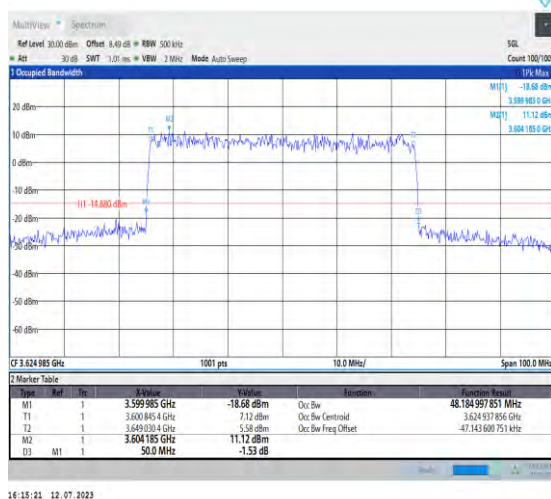
1-N48-PC3-30-50-M-3-DFT-16QAM-Outter_Full-128 @0-Ant3-48.185-50.000-≤50-PASS
