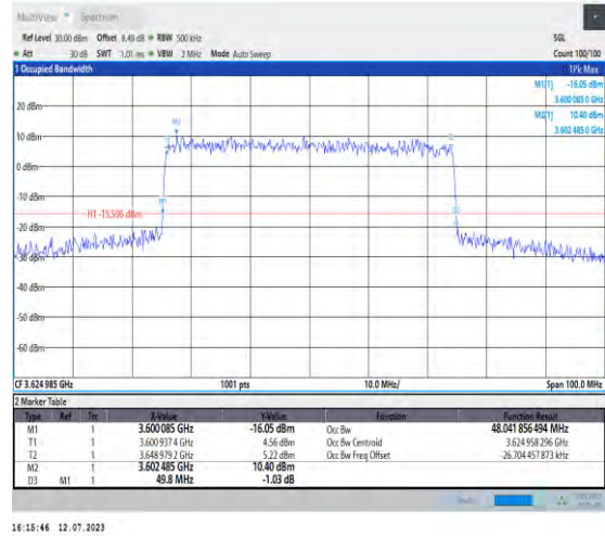
1-N48-PC3-30-50-M-6-CP-QPSK-Outer_Full-133@ 0-Ant3-48.042-49.800-≤50-PASS
