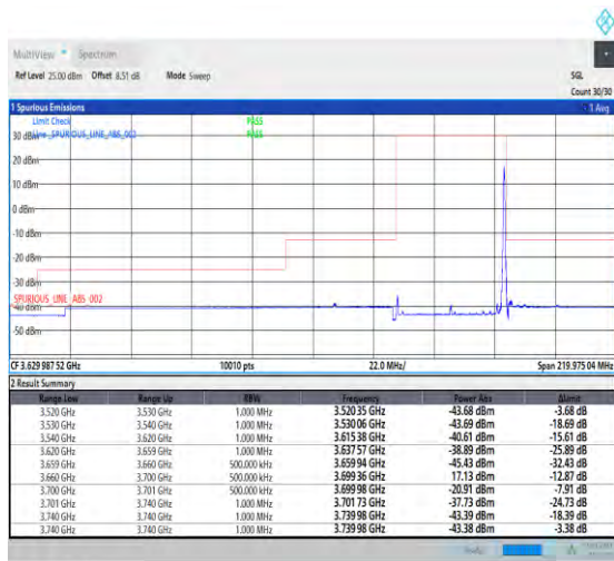
1-N48-PC3-30-40-H-2-DFT-PI2BPSK-Edge_1RB_Right-1@105-Ant3-1--PASS-see graph
