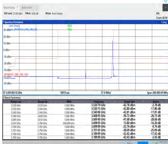
1-N48-PC3-30-90-H-5-CP-QPSK-Edge_1RB_Right-1@244-Ant3-1--PASS-see graph
