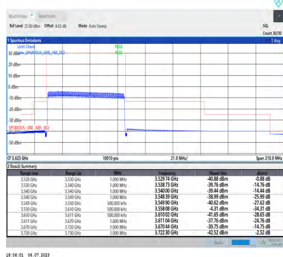
1-N48-PC3-30-60-L-6-CP-QPSK-Outer_Full-162@0 -Ant3-1--PASS-see graph
