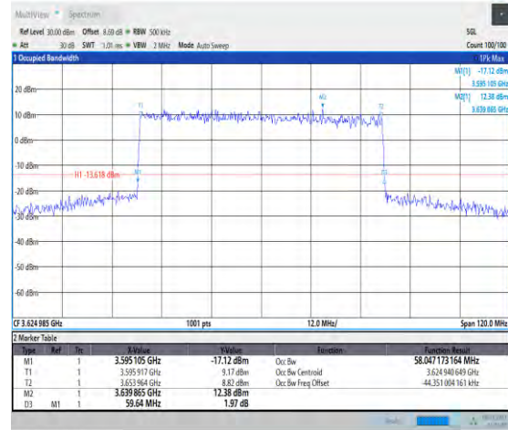
1-N48-PC3-30-60-M-1-DFT-QPSK-Outet_Full-162@ 0-Ant3-58.047-59.640-≤60-PASS
