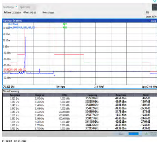
1-N48-PC3-30-40-L-4-CP-QPSK-Edge_1RB_Left-1@ 0-Ant3-1--PASS-see graph
