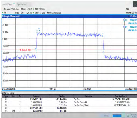
1-N48-PC3-30-60-M-8-CP-64QAM-Outer_Full-162 @0-Ant3-57.726-59.640-≤60-PASS
