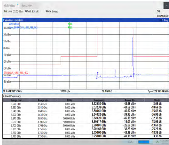
1-N48-PC3-30-50-H-2-DFT-PI2BPSK-Edge_1RB_Right-t-1@132-Ant3-1--PASS-see graph
