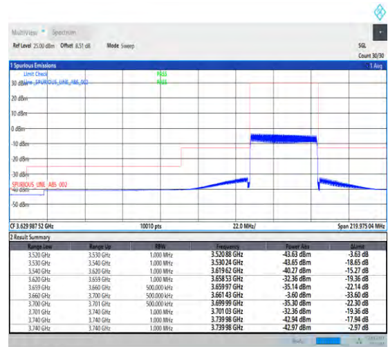
1-N48-PC3-30-40-H-3-DFT-PI2BPSK-Outer_Full-100@0-Ant3-1--PASS-see graph
