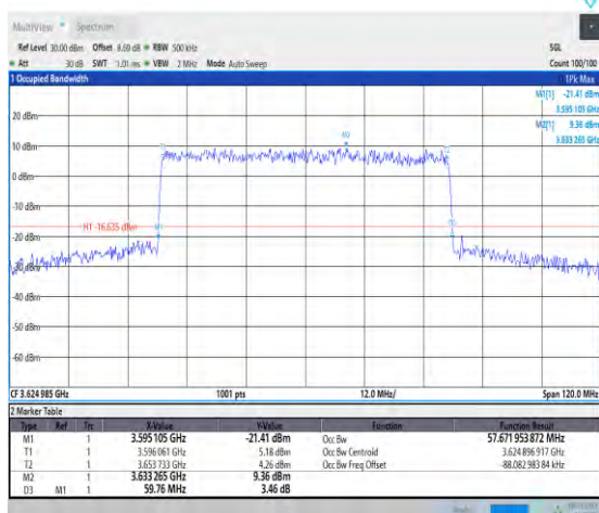
1-N48-PC3-30-60-M-6-CP-QPSK-Outer_Full-162@0 -Ant3-57.672-59.760-≤60-PASS
