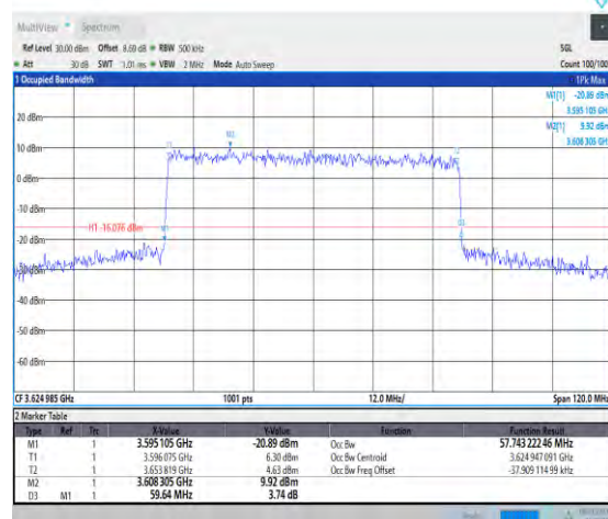
1-N48-PC3-30-60-M-7-CP-16QAM-Outer_Full-162@ 0-Ant3-57.743-59.640-≤60-PASS
