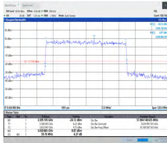
1-N48-PC3-30-60-M-5-DFT-256QAM-Outer_Full-162 @0-Ant3-57.904-59.760-≤60-PASS
