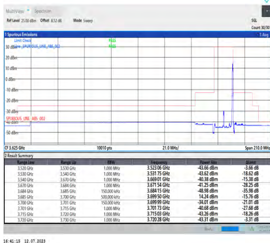
1-N48-PC3-30-15-H-5-CP-QPSK-Edge_1RB_Right-1@37-Ant3-1--PASS-see graph
