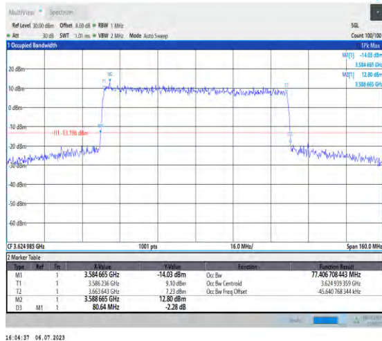
1-N48-PC3-30-80-M-7-CP-16QAM-Outer_Full-217@ 0-Ant3-77.407-80.640-≤80-PASS
