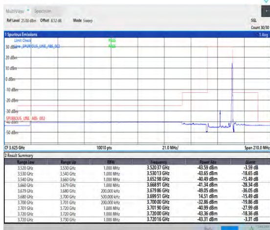
1-N48-PC3-30-20-H-5-CP-QPSK-Edge_1RB_Right-1@50-Ant3-1--PASS-see graph
