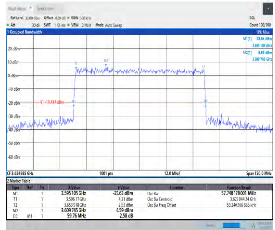
1-N48-PC3-30-60-M-9-CP-256QAM-Outer_Full-162 @0-Ant3-57.748-59.760-≤60-PASS
