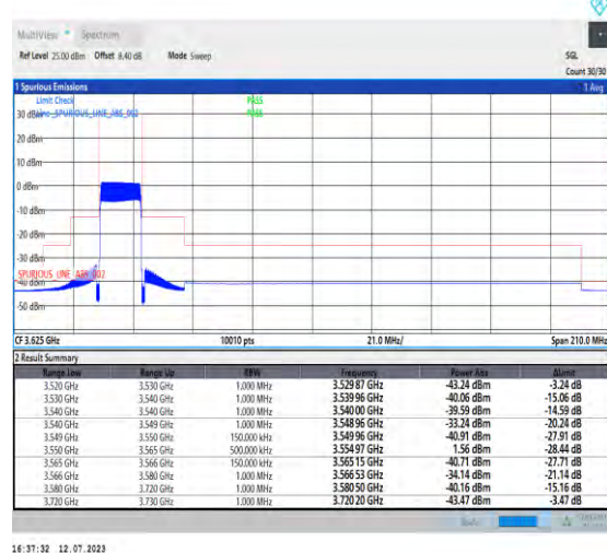
1-N48-PC3-30-15-L-6-CP-QPSK-Outer_Full-38@0-Ant3-1--PASS-see graph
