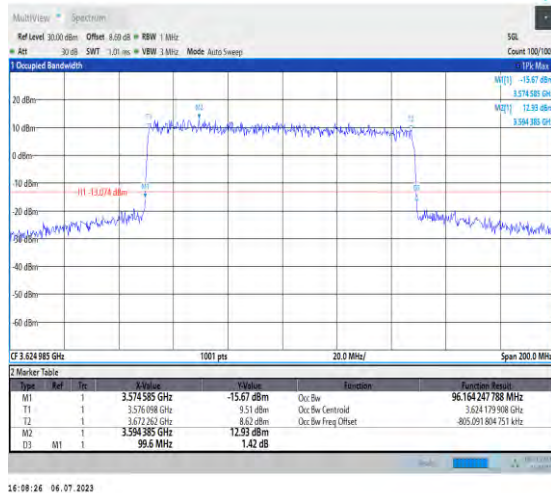
1-N48-PC3-30-100-M-1-DFT-QPSK-Outter_Full-51@ 0-Ant3-96.164-99.600-≤100-PASS
