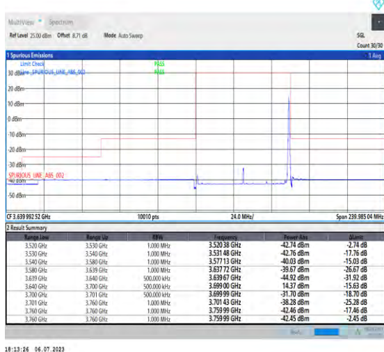
1-N48-PC3-30-60-H-5-CP-QPSK-Edge_1RB_Right-1@161-Ant3-1--PASS-see graph
