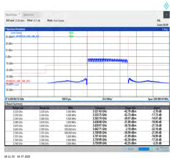
1-N48-PC3-30-60-H-3-DFT-PI2BPSK-Outer_Full-162@0-Ant3-1--PASS-see graph
