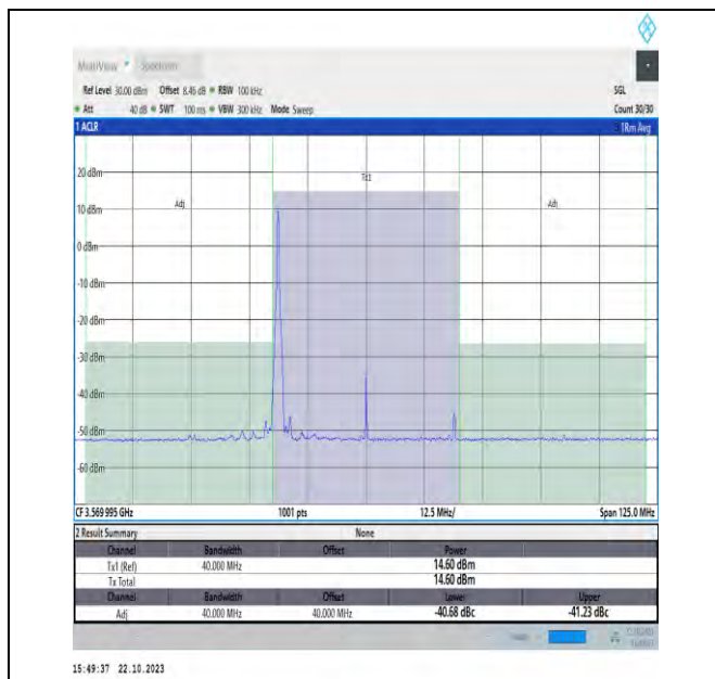
NTNV_N48_PC3_30_40_L_TID17_#1_-40_40
