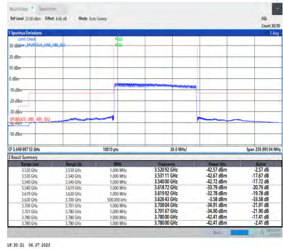
1-N48-PC3-30-80-H-3-DFT-PI2BPSK-Outer_Full-100@0-Ant3-1--PASS-see graph
