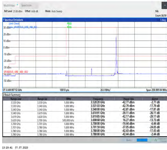
1-N48-PC3-30-80-H-2-DFT-PI2BPSK-Edge_1RB_Right-t-1@216-Ant3-1--PASS-see graph
