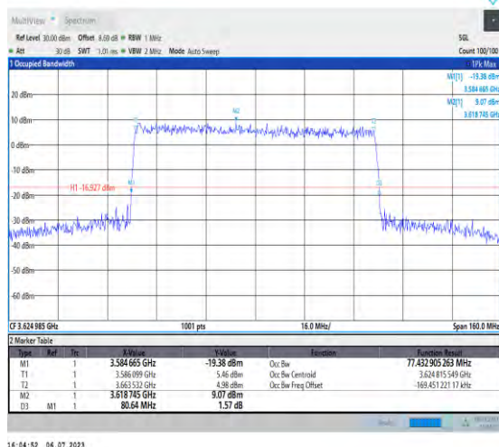
1-N48-PC3-30-80-M-9-CP-256QAM-Outer_Full-217@ 0-Ant3-77.433-80.640-≤80-PASS
