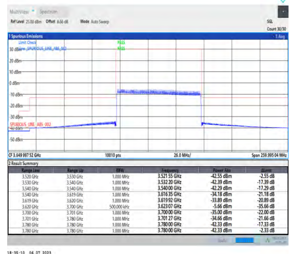
1-N48-PC3-30-80-H-6-CP-QPSK-Outer_Full-217@0-Ant3-1--PASS-see graph
