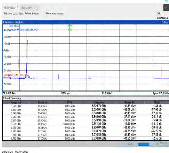
1-N48-PC3-30-80-L-4-CP-QPSK-Edge_1RB_Left-1@0-Ant3-1--PASS-see graph
