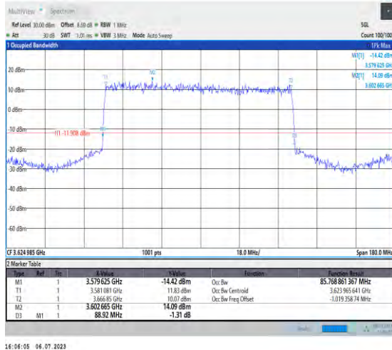
1-N48-PC3-30-90-M-2-DFT-PI2BPSK-Out_24 @0-Ant3-85.769-88.920-≤90-PASS
