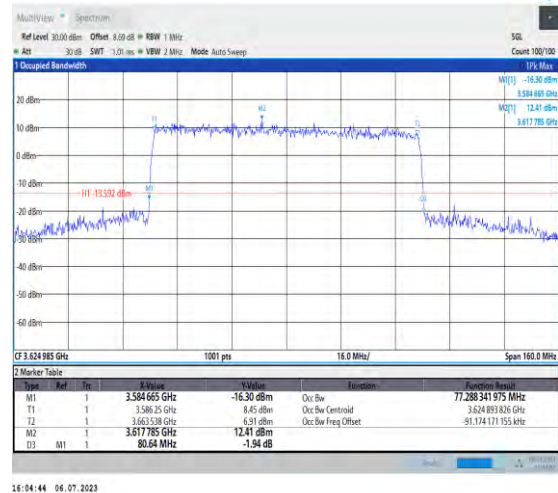
1-N48-PC3-30-80-M-8-CP-64QAM-Outer_Full-217@ 0-Ant3-77.288-80.640-≤80-PASS
