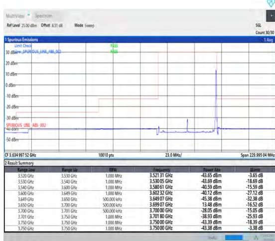
1-N48-PC3-30-50-H-5-CP-QPSK-Edge_1RB_Right-1@132-Ant3-1--PASS-see graph
