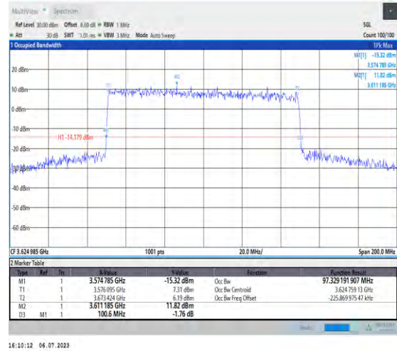
1-N48-PC3-30-100-M-6-CP-QPSK-Outer_Full-273@ 0-Ant3-97.329-100.600-≤100-PASS
