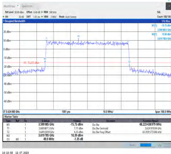
1-N48-PC3-30-50-M-7-CP-16QAM-Outer_Full-133@ 0-Ant3-48.223-49.900-≤50-PASS
