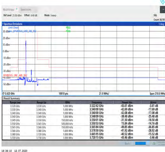
1-N48-PC3-30-15-L-4-CP-QPSK-Edge_1RB_Left-1@0-Ant3-1--PASS-see graph
