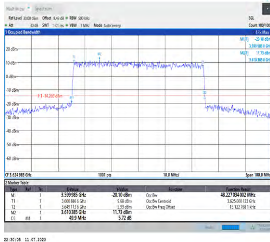
1-N48-PC3-30-50-M-1-DFT-QPSK-Outter_Full-128@ 0-Ant3-48.227-49.900-≤50-PASS
