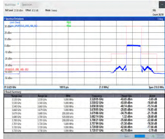
1-N48-PC3-30-20-H-3-DFT-PI2BPSK-Outer_Full-50@0-Ant3-1--PASS-see graph
