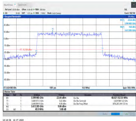
1-N48-PC3-30-50-M-8-CP-64QAM-Outer_Full-133 @0-Ant3-48.022-49.900-≤50-PASS
