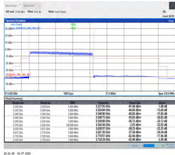
1-N48-PC3-30-80-L-3-DFT-PI2BPSK-Outer_Full-100@0-Ant3-1--PASS-see graph
