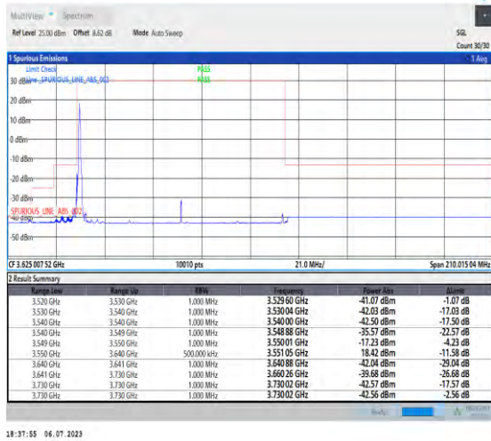
1-N48-PC3-30-90-L-1-DFT-PI2BPSK-Edge_1RB_Left-1@0-Ant3-1--PASS-see graph
