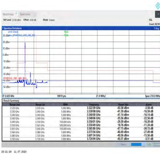
1-N48-PC3-30-15-L-1-DFT-PI2BPSK-Edge_1RB_Left-1@0-Ant3-1--PASS-see graph
