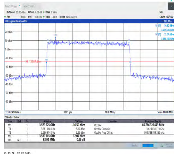
1-N48-PC3-30-90-M-5-DFT-256QAM-Out_240 @0-Ant3-85.766-88.920-≤90-PASS
