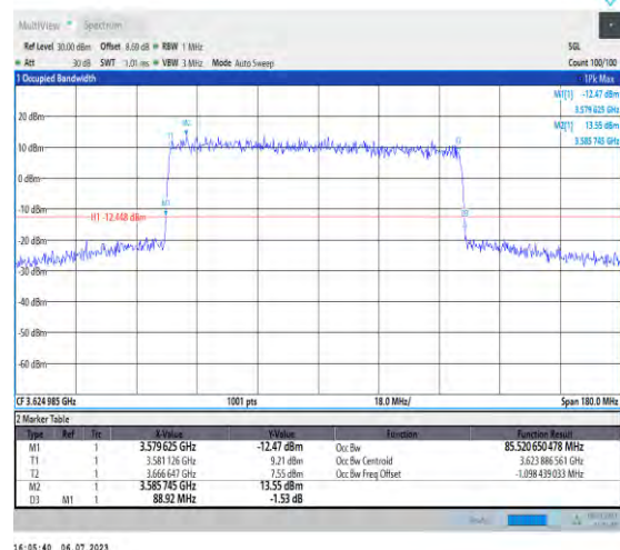
1-N48-PC3-30-90-M-1-DFT-QPSK-Outer_Full-240@ 0-Ant3-85.521-88.920-≤90-PASS
