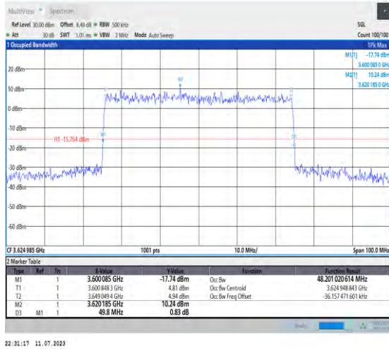
1-N48-PC3-30-50-M-5-DFT-256QAM-Outer_Full-128 @0-Ant3-48.201-49.800-≤50-PASS
