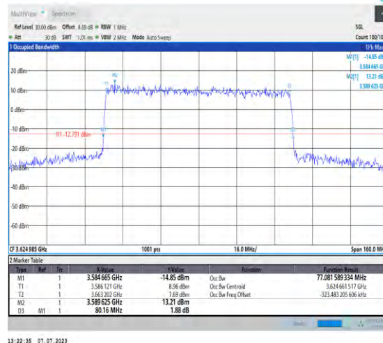
1-N48-PC3-30-80-M-4-DFT-64QAM-Outer_Full-100 @0-Ant3-77.082-80.160-≤80-PASS
