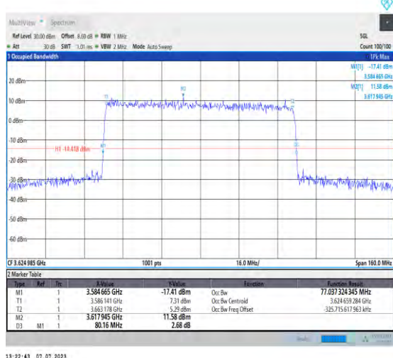
1-N48-PC3-30-80-M-5-DFT-256QAM-Outer_Full-100 @0-Ant3-77.037-80.160-≤80-PASS
