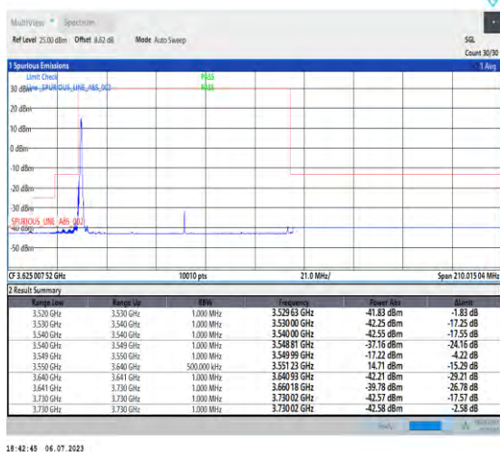
1-N48-PC3-30-90-L-4-CP-QPSK-Edge_1RB_Left-1@0-Ant3-1--PASS-see graph
