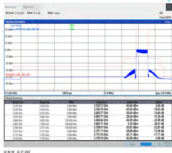
1-N48-PC3-30-15-H-6-CP-QPSK-Outer_Full-38@0-Ant3-1--PASS-see graph
