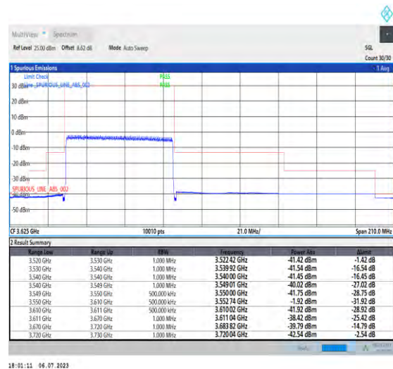
1-N48-PC3-30-60-L-3-DFT-PI2BPSK-Outer_Full-16 2@0-Ant3-1--PASS-see graph
