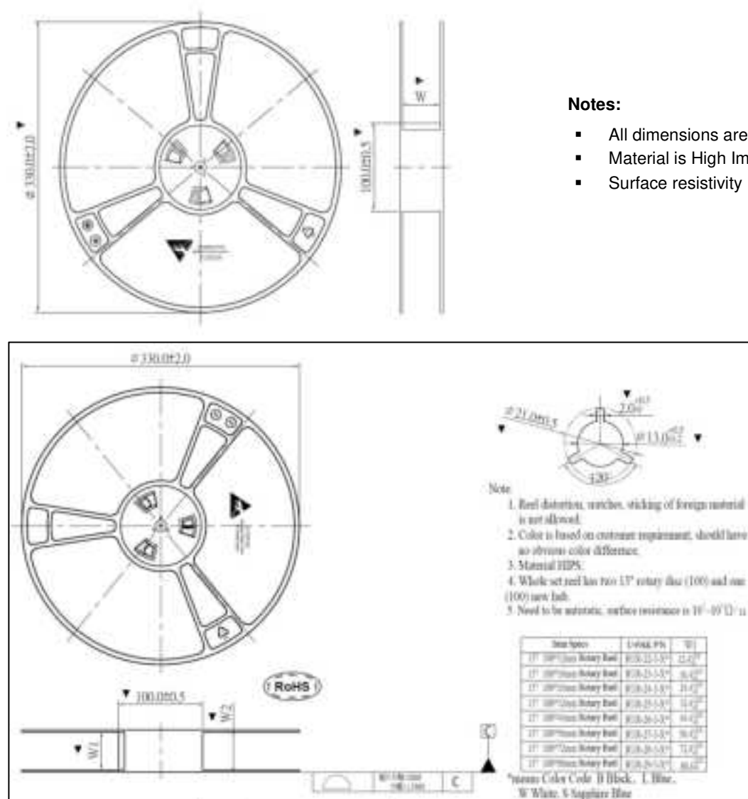
Figure 13: Reel specifications
