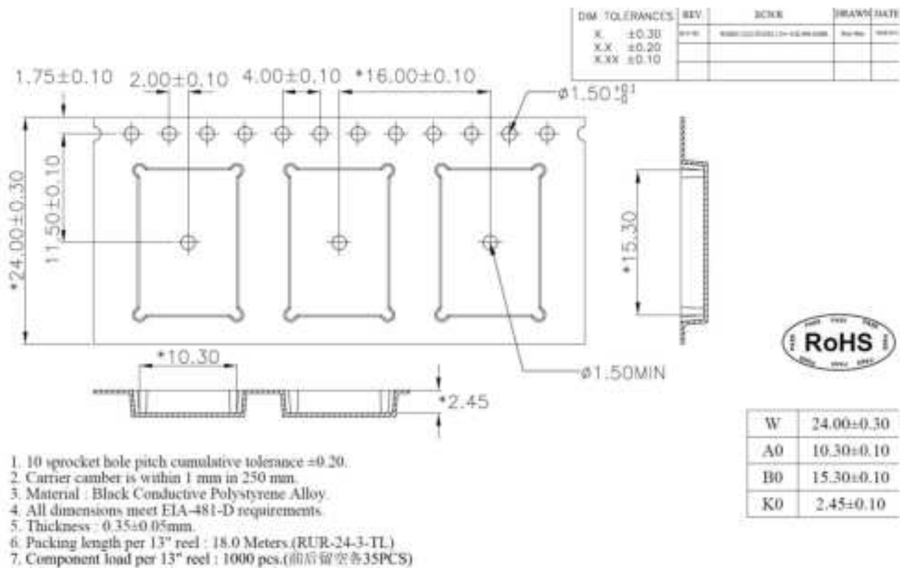
Figure 14: Tape specifications
