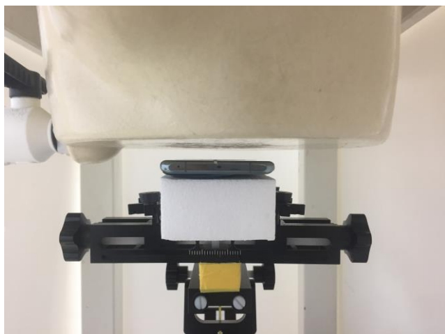
Front, Test Separation 11 mm
