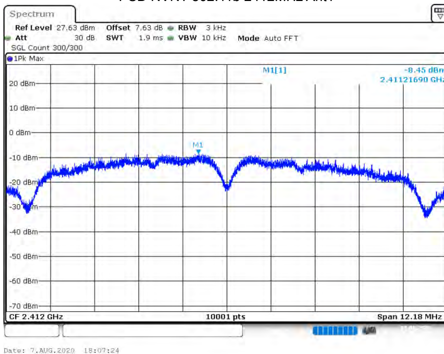
PSD NVNT 802.11b 2412MHz Ant1
