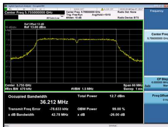
Channel 151 (5755MHz)
