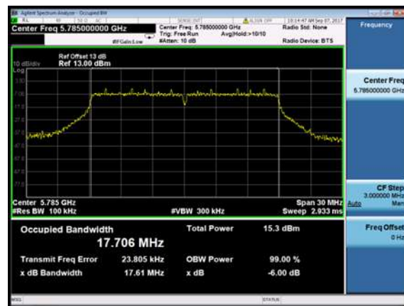
Channel 157 (5785MHz)
