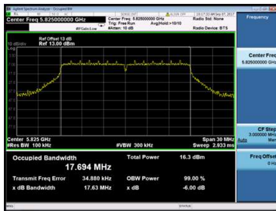
Channel 165 (5825MHz)
