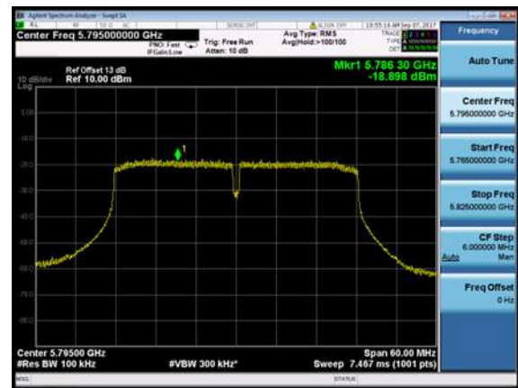
Channel 159 (5795MHz)
