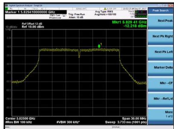
Channel 165 (5825MHz)
