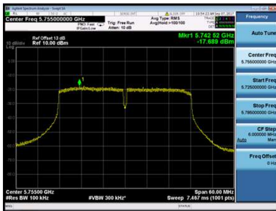
Channel 155 (5755MHz)
