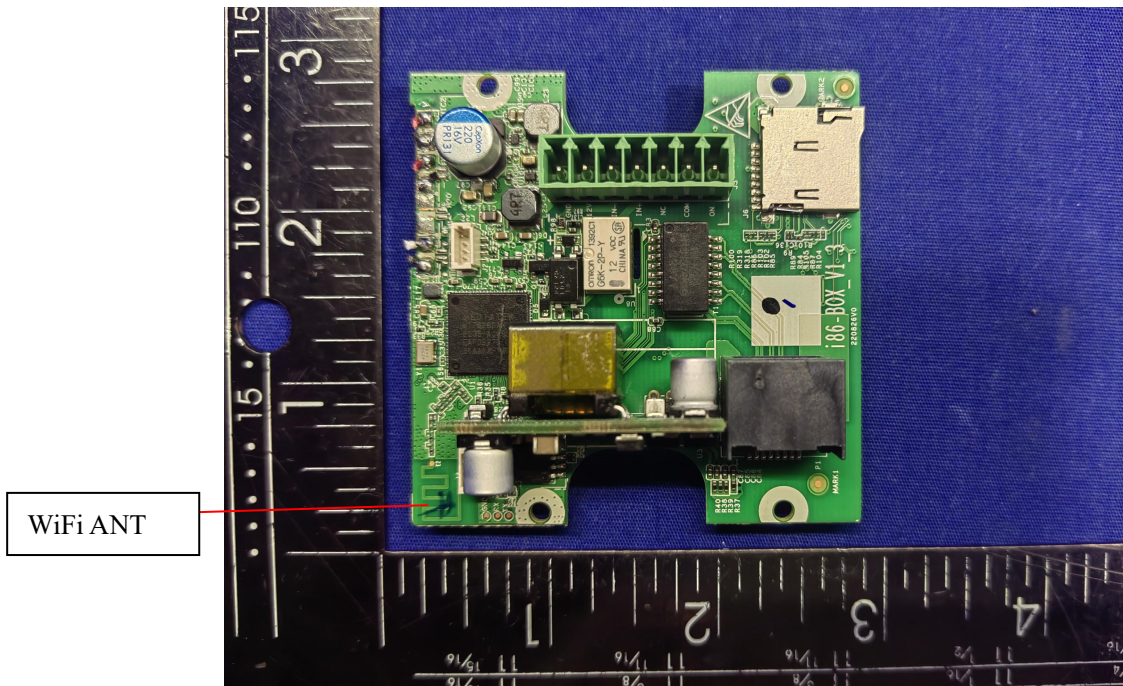
EUT View 7
