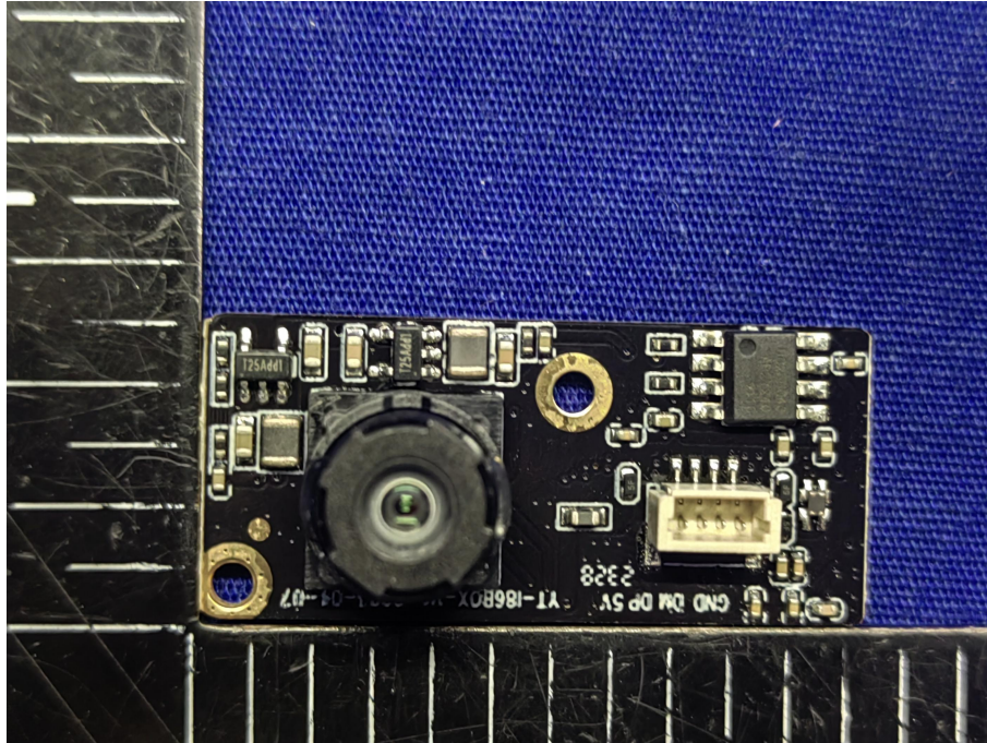
EUT View 11
