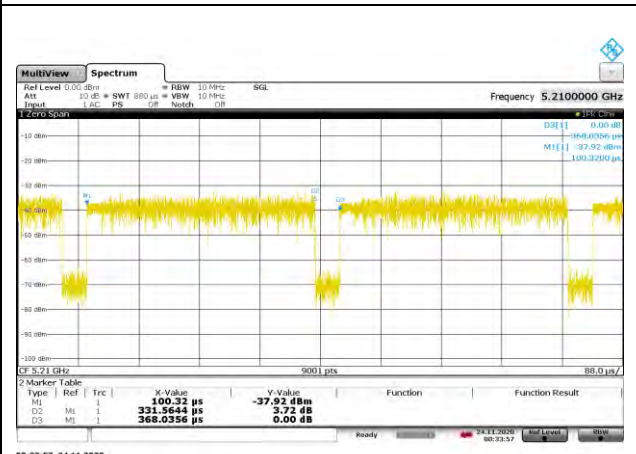
DUTY CYCLE 802.11ac VHT80
