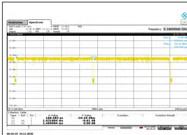
DUTY CYCLE 802.11a
