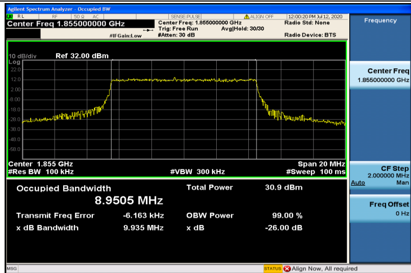
Band2-10MHz-16QAM-18650-50RB#0-8.9505
