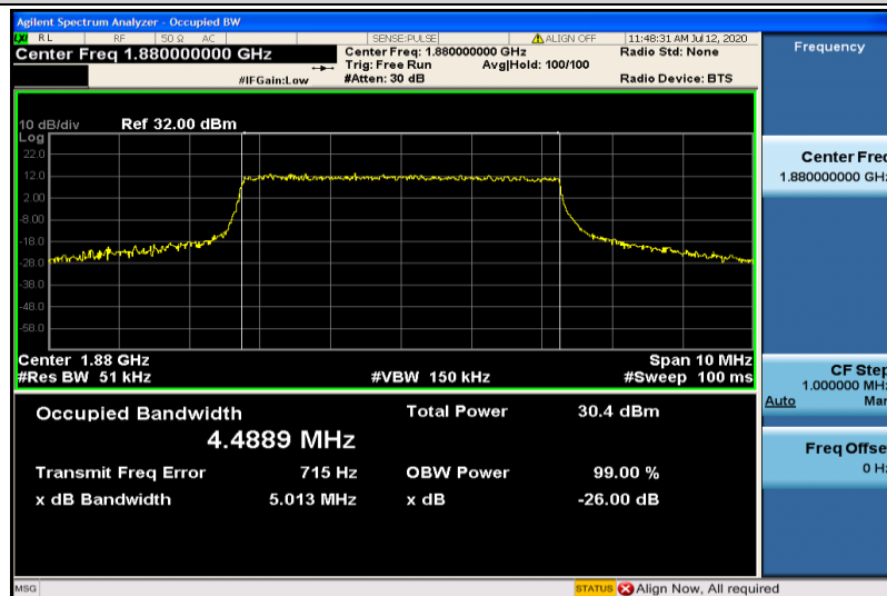
Band2-5MHz-16QAM-18900-25RB#0-4.4889
