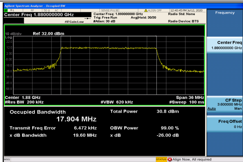
Band2-20MHz-16QAM-18900-100RB#0-17.904
