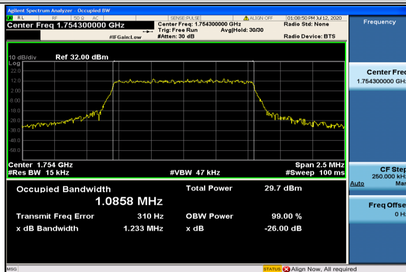
Band4-1.4MHz-16QAM-20393-6RB#0-1.0858
