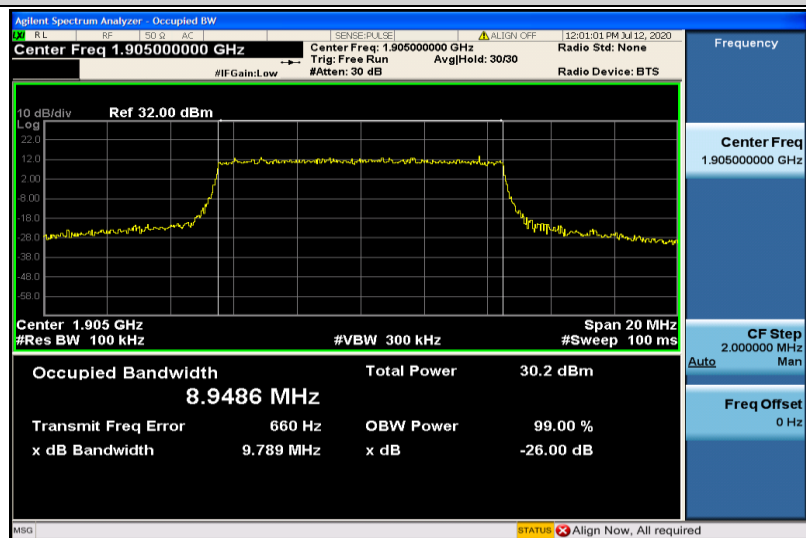
Band2-10MHz-16QAM-19150-50RB#0-8.9486
