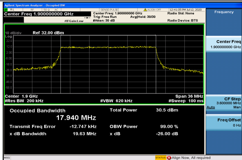
Band2-20MHz-16QAM-19100-100RB#0-17.940
