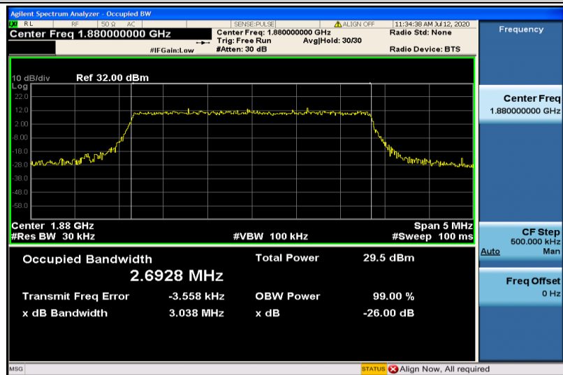
Band2-3MHz-16QAM-18900-15RB#0-2.6928
