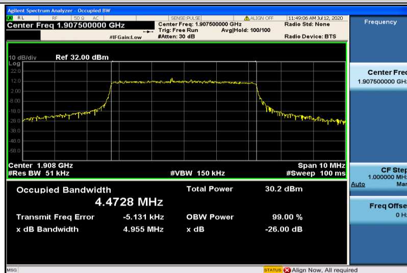
Band2-5MHz-16QAM-19175-25RB#0-4.4728
