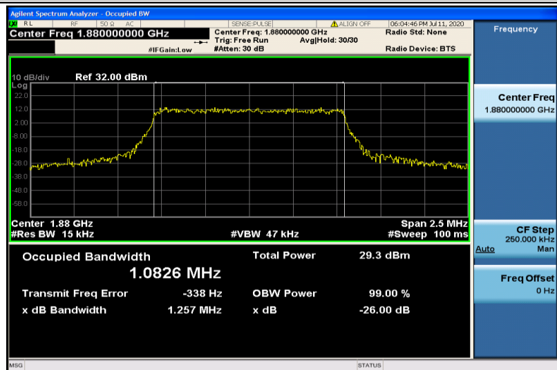
Band2-1.4MHz-16QAM-18900-6RB#0-1.0826
