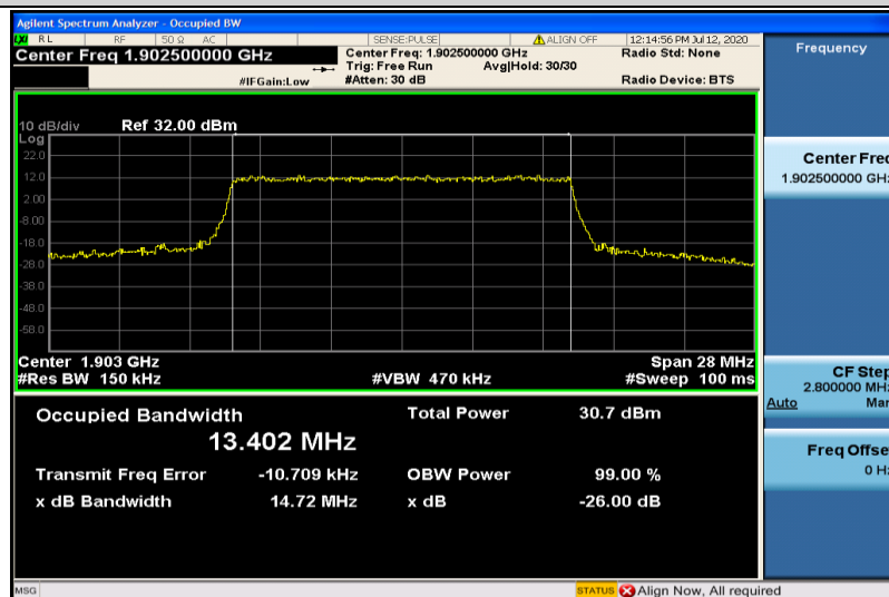
Band2-15MHz-16QAM-19125-75RB#0-13.402
