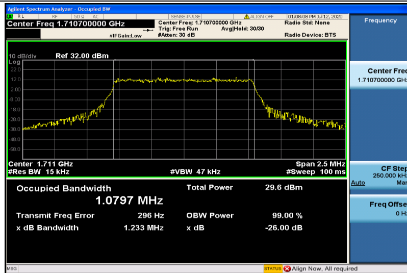
Band4-1.4MHz-16QAM-19957-6RB#0-1.0797
