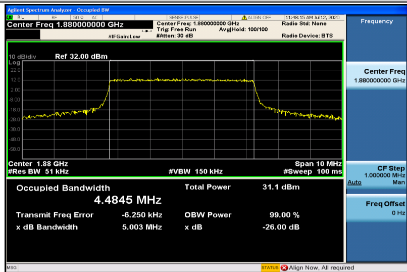
Band2-5MHz-QPSK-18900-25RB#0-4.4845
