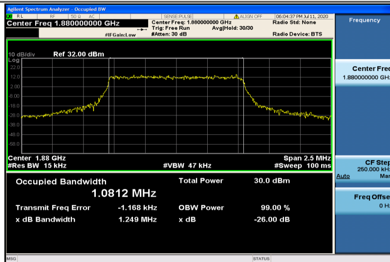
Band2-1.4MHz-QPSK-18900-6RB#0-1.0812
