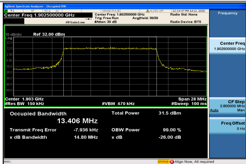
Band2-15MHz-QPSK-19125-75RB#0-13.406
