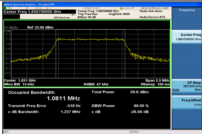
Band2-1.4MHz-16QAM-18607-6RB#0-1.0811
