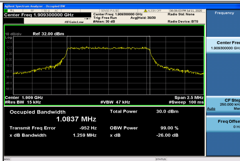
Band2-1.4MHz-QPSK-19193-6RB#0-1.0837
