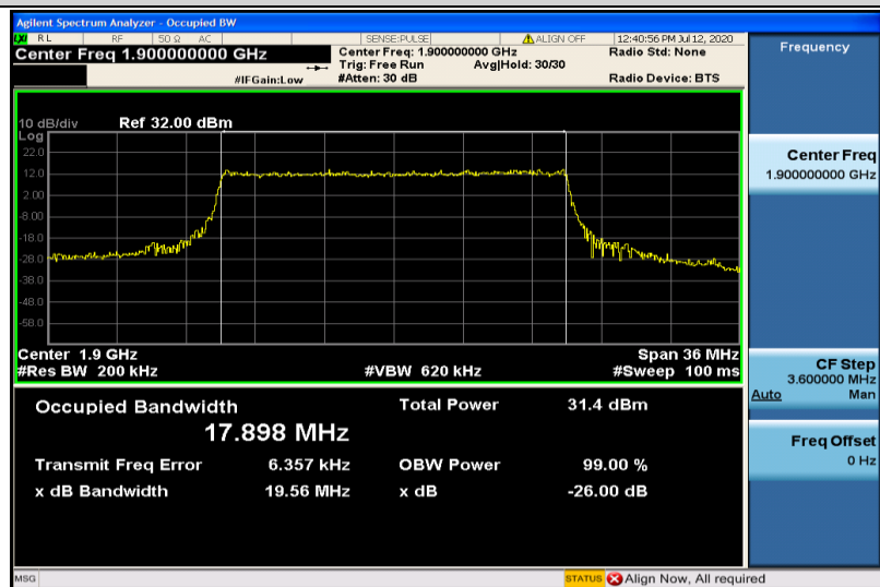
Band2-20MHz-QPSK-19100-100RB#0-17.898
