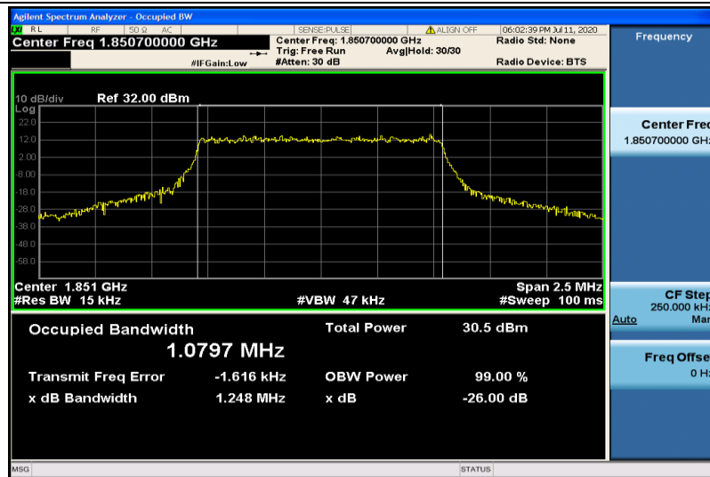
Band2-1.4MHz-QPSK-18607-6RB#0-1.0797
