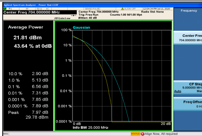
Band12-10MHz-16QAM-23060-50RB#0
