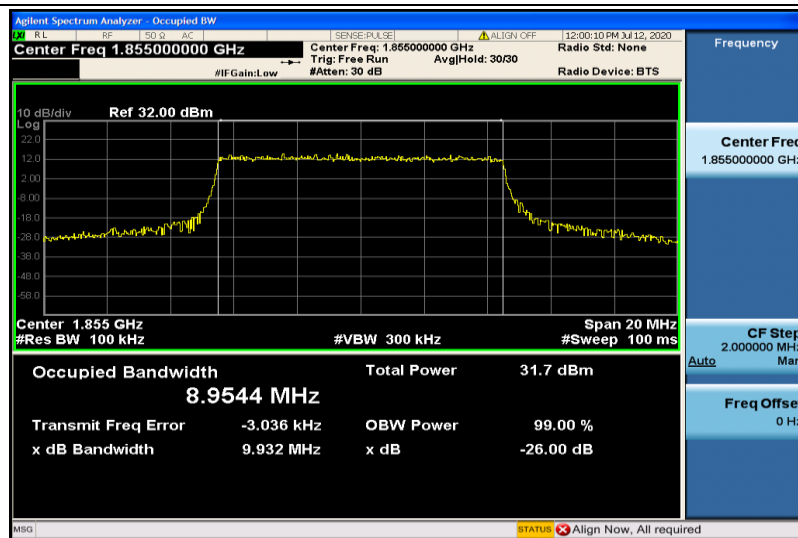
Band2-10MHz-QPSK-18650-50RB#0-8.9544
