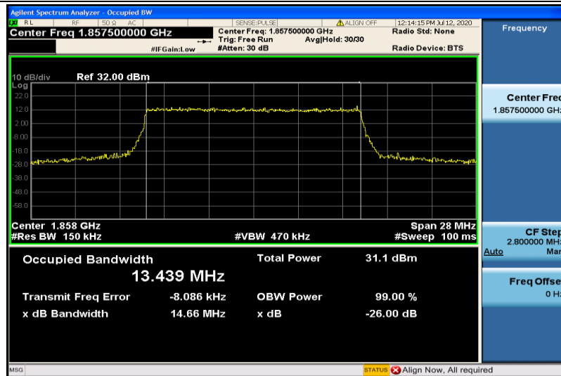
Band2-15MHz-16QAM-18675-75RB#0-13.439
