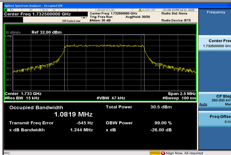
Band4-1.4MHz-QPSK-20175-6RB#0-1.0819
