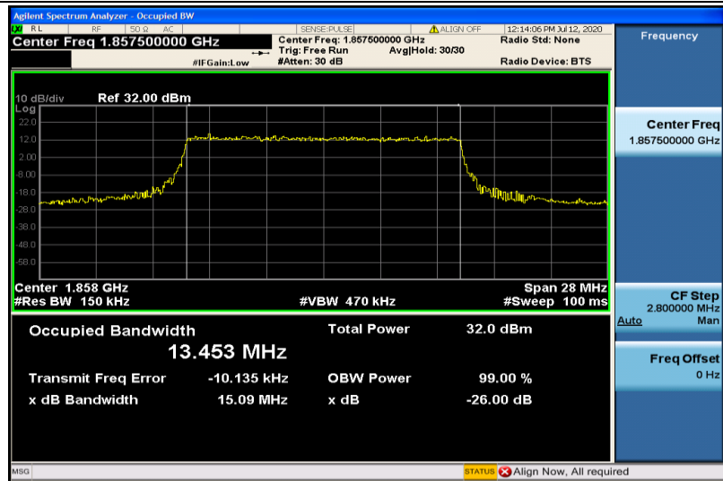
Band2-15MHz-QPSK-18675-75RB#0-13.453
