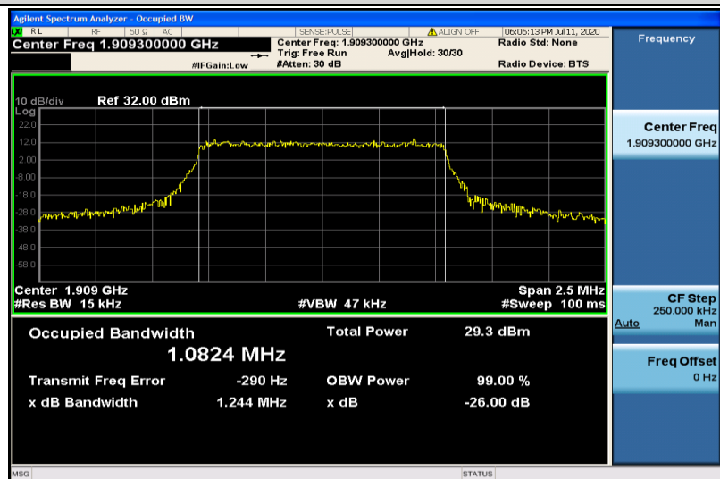
Band2-1.4MHz-16QAM-19193-6RB#0-1.0824
