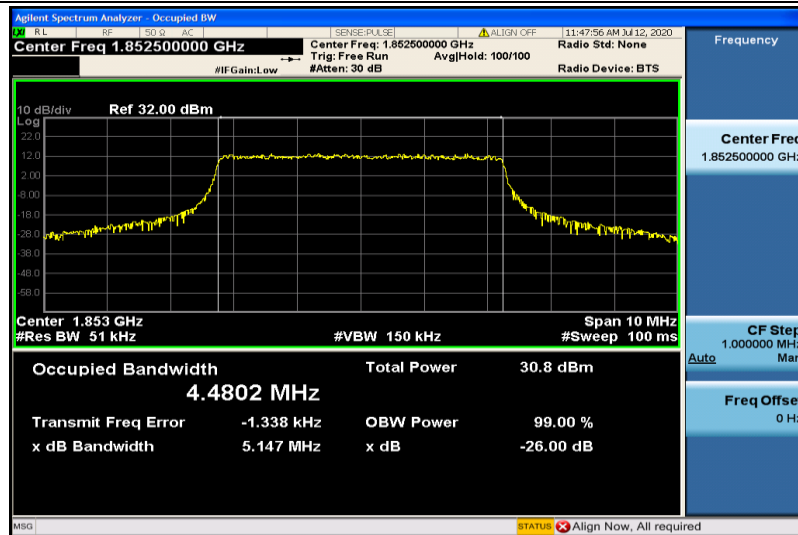
Band2-5MHz-16QAM-18625-25RB#0-4.4802
