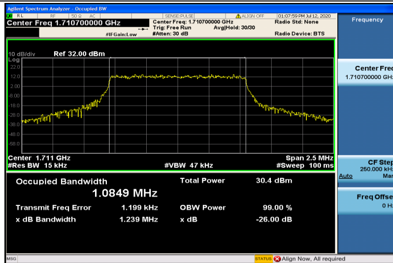
Band4-1.4MHz-QPSK-19957-6RB#0-1.0849
