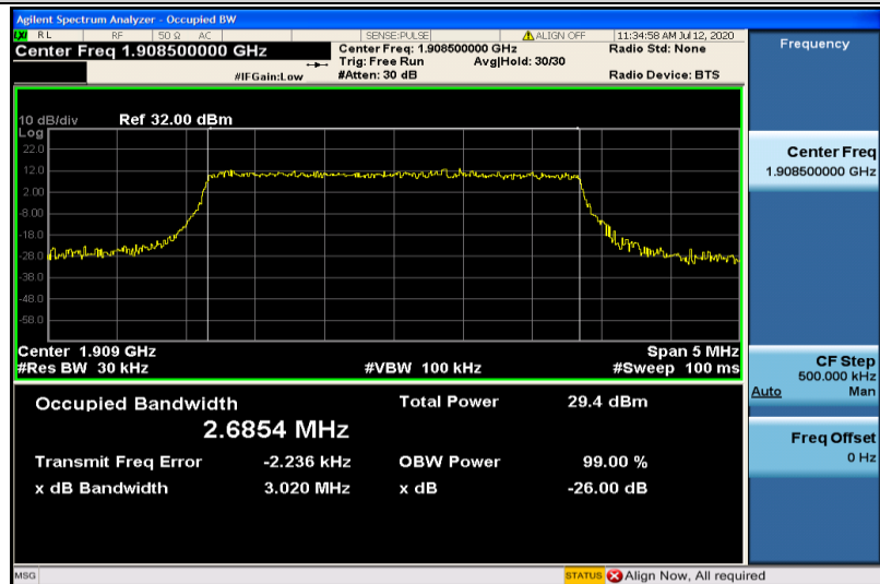
Band2-3MHz-16QAM-19185-15RB#0-2.6854
