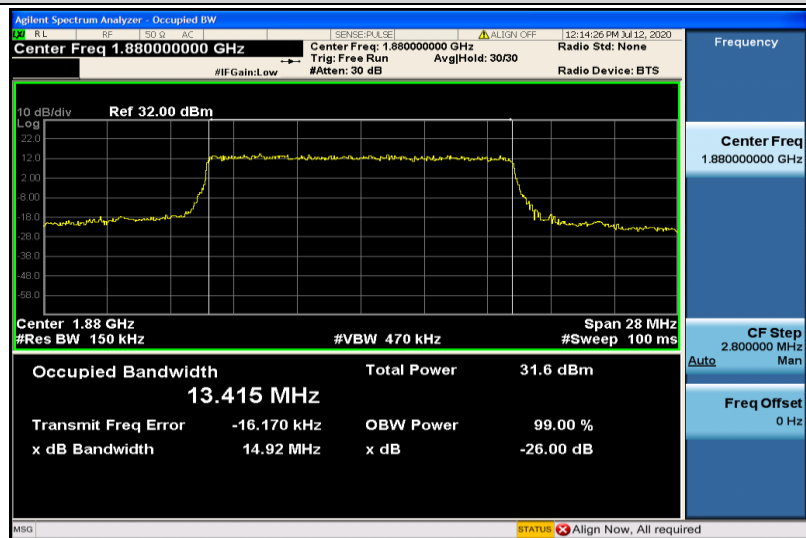
Band2-15MHz-QPSK-18900-75RB#0-13.415
