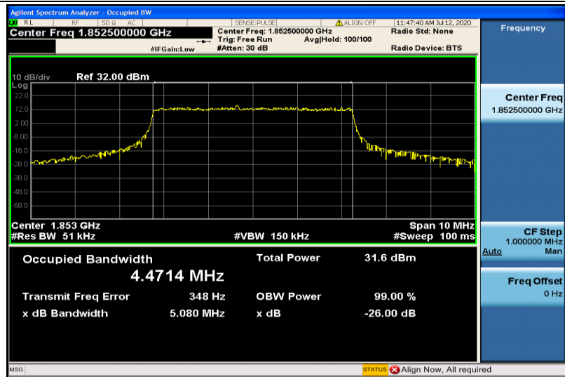
Band2-5MHz-QPSK-18625-25RB#0-4.4714
