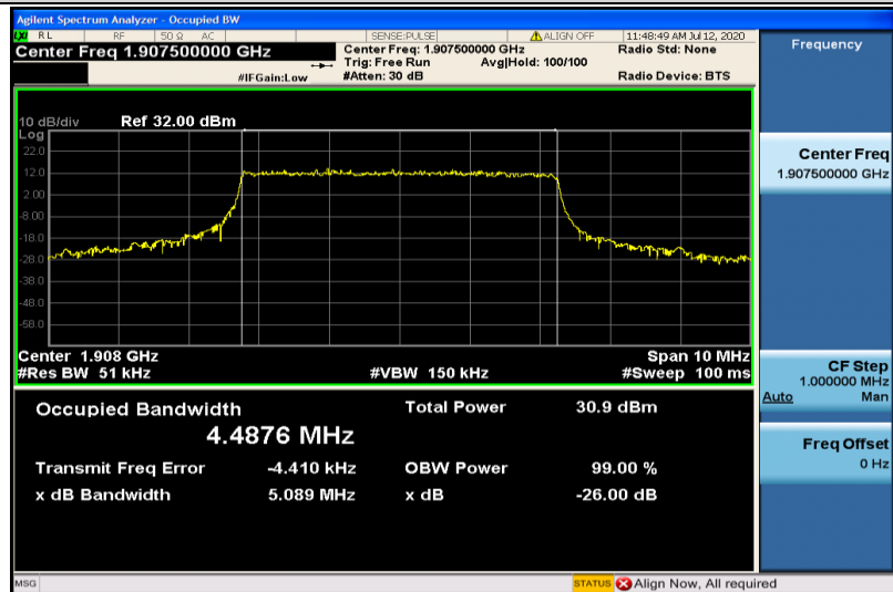
Band2-5MHz-QPSK-19175-25RB#0-4.4876
