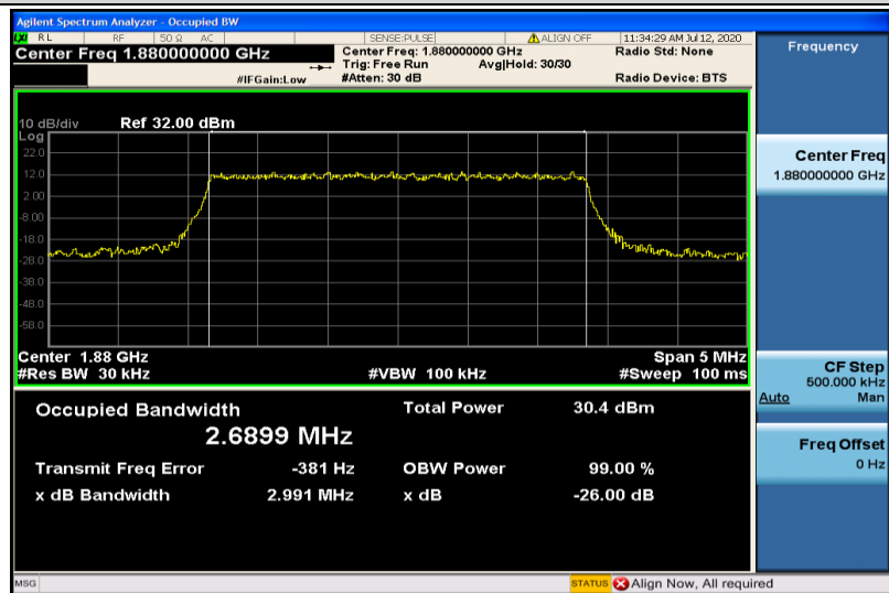
Band2-3MHz-QPSK-18900-15RB#0-2.6899
