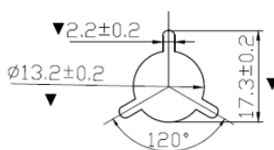
Figure 10.4. Central Axis Dimensions
