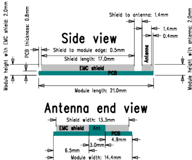
Figure 8.2. Side View Dimensions for WGM110 Module - Side and Antenna End Views
