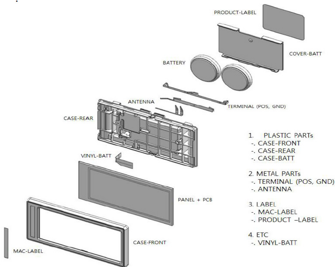
Figure 4 Exploded View
