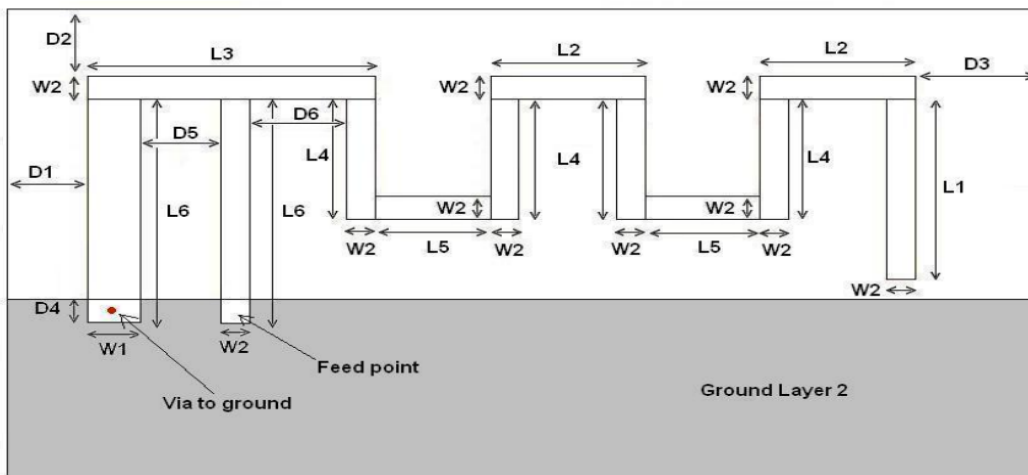
Figure 3: Antenna Dimensions
