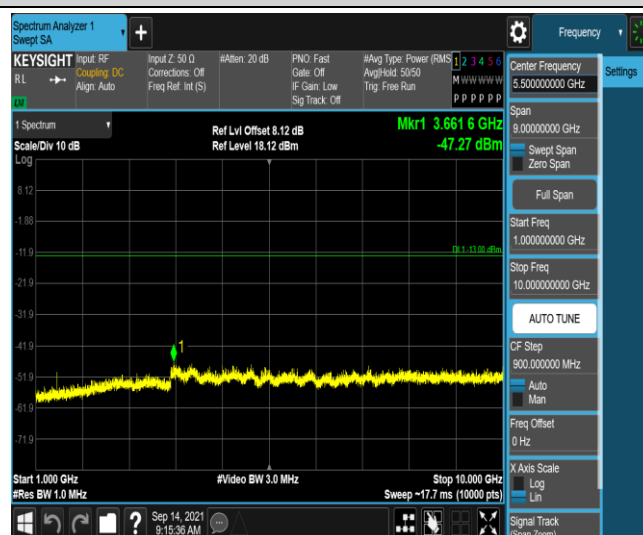
Band17-5MHz-QPSK-23755-1RB#0-Range4:1000~10000MHz
