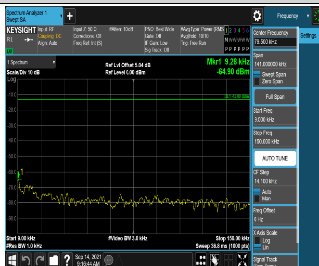
Band17-5MHz-QPSK-23790-1RB#0-Range1:0.009~0.15MHz
