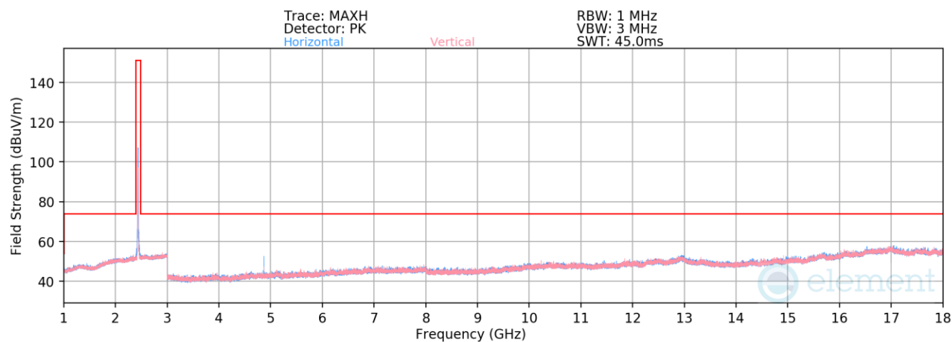
Plot 7-39. Radiated Spurious Plot above 1GHz (802.11b – Ch. 6)
