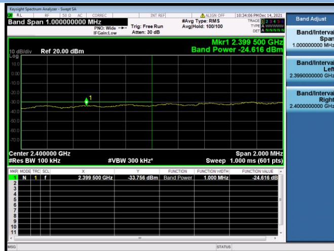
802.11n-20 MHz CHANNEL 1, Band Edge
