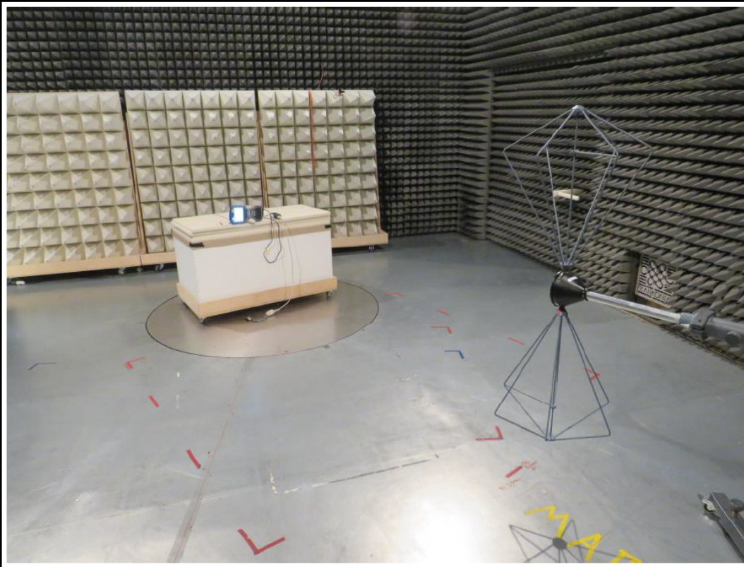
Test setup 30-200MHz
