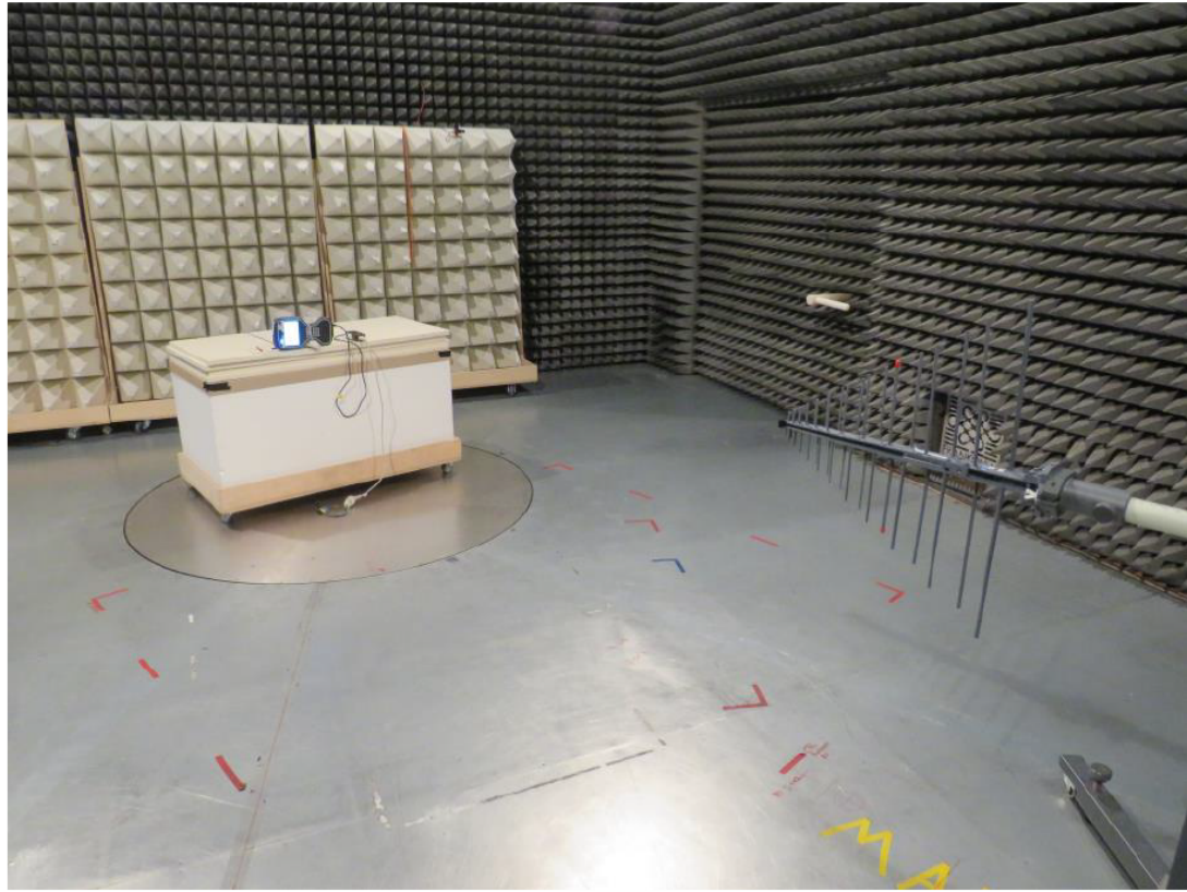
Test setup 200-1000MHz
