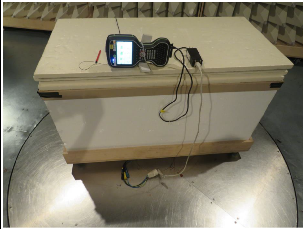
Test setup
