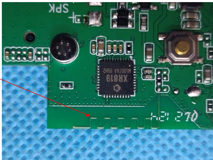
WIFI-PCB Antenna
