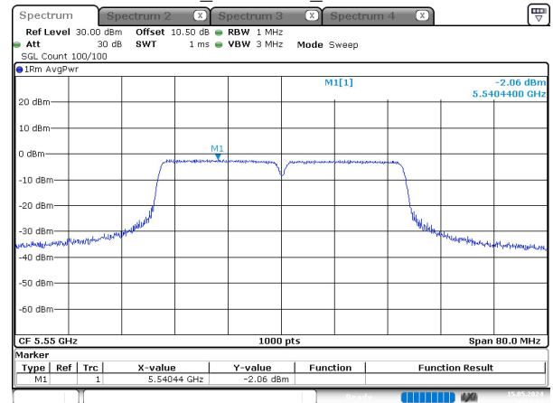
n40_5550MHz_Chain 0
