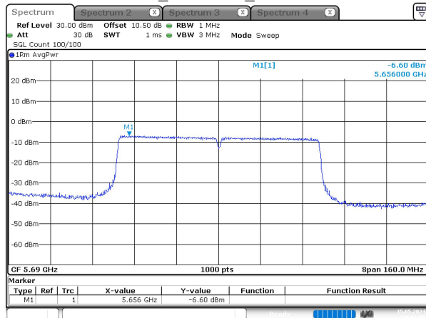
ac80_5690MHz_Chain 0
