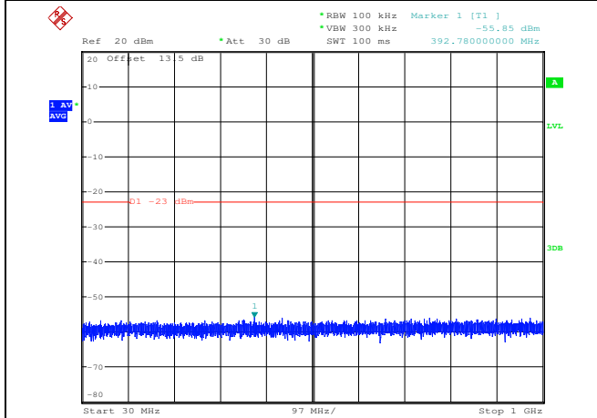
EGPRS1900-Middle Channel
