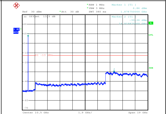
EGPRS1900-High Channel
