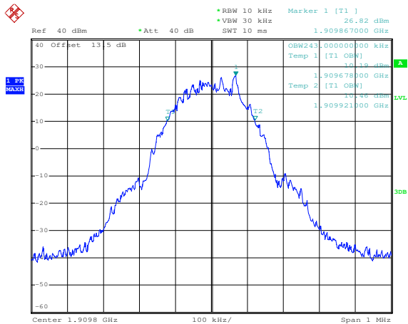
GSM1900-High Channel
