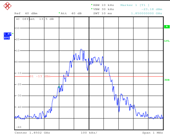
GSM1900-Low Channel
