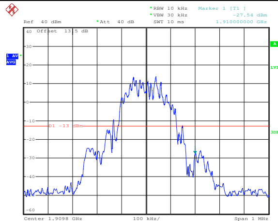
GSM1900-High Channel
