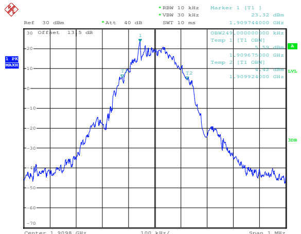
EGPRS1900-High Channel
