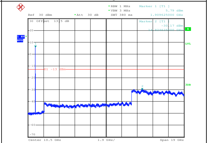
EGPRS1900-High Channel
