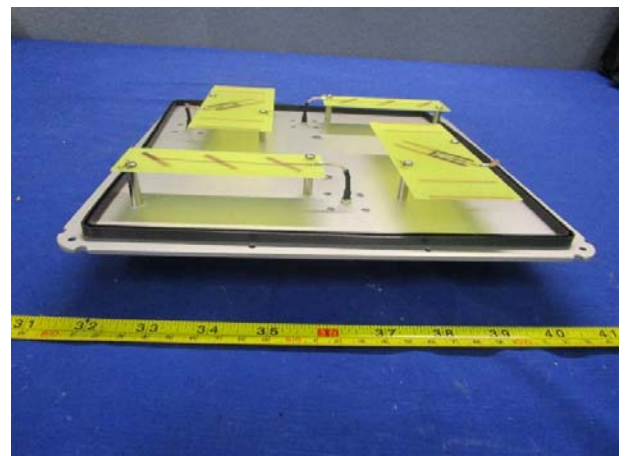
PCBA 1 Right Side View
