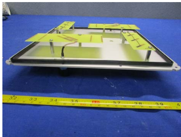
PCBA 1 Left Side View
