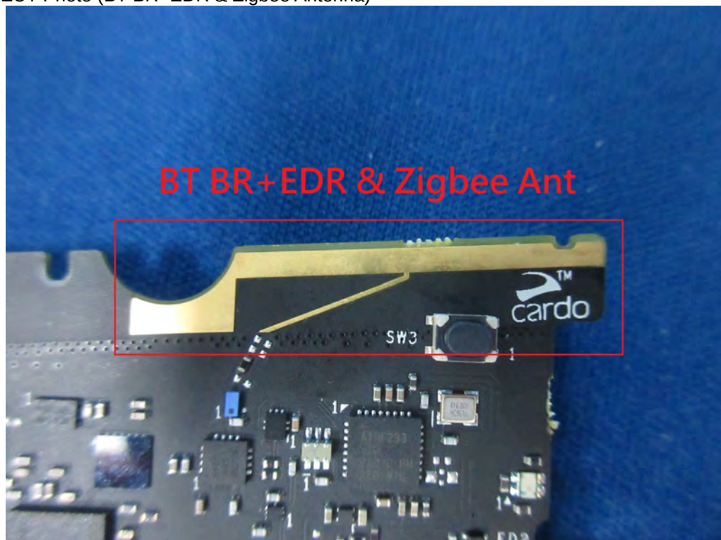
(8) EUT Photo (BT BR+EDR & Zigbee Antenna)
