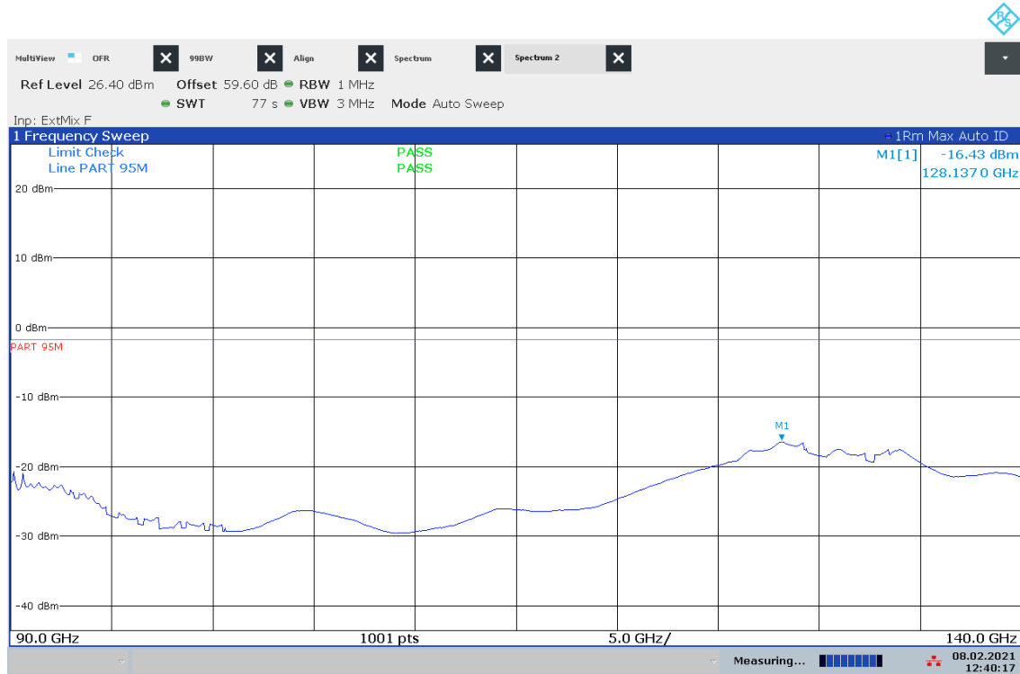
Plot 41: 90 GHz – 140 GHz, vertical / horizontal polarization, Mode 5
