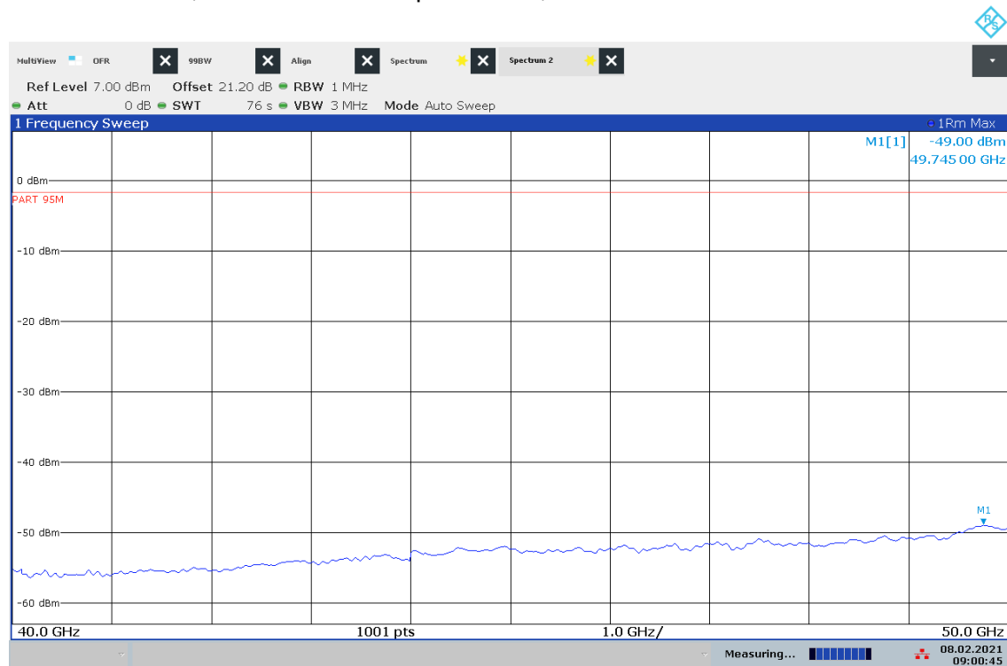
Plot 28: 40 GHz – 50 GHz, vertical / horizontal polarization, Mode 3
