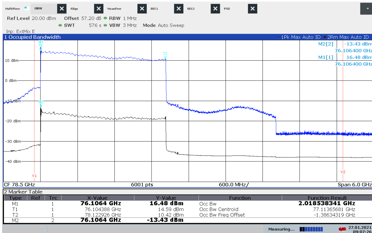
Plot 9: Mode 6 – OBW
