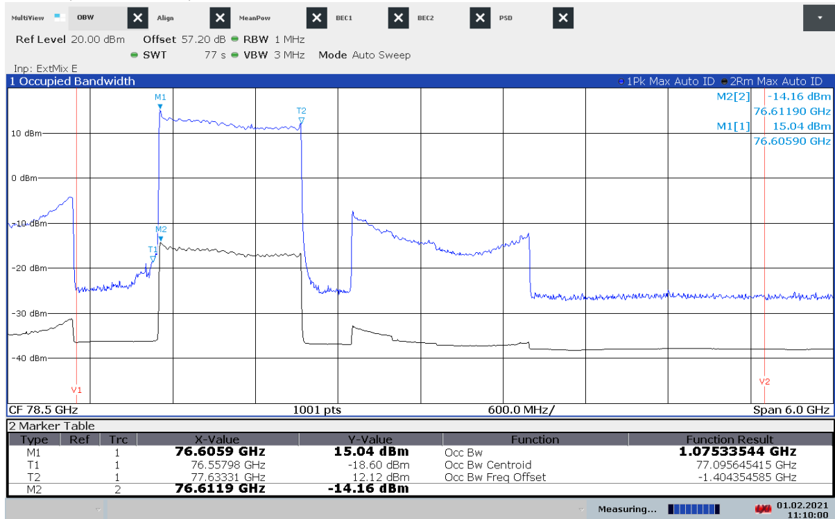
Plot 61: OBW, +20 °C / V_{nom} , Mode 3
