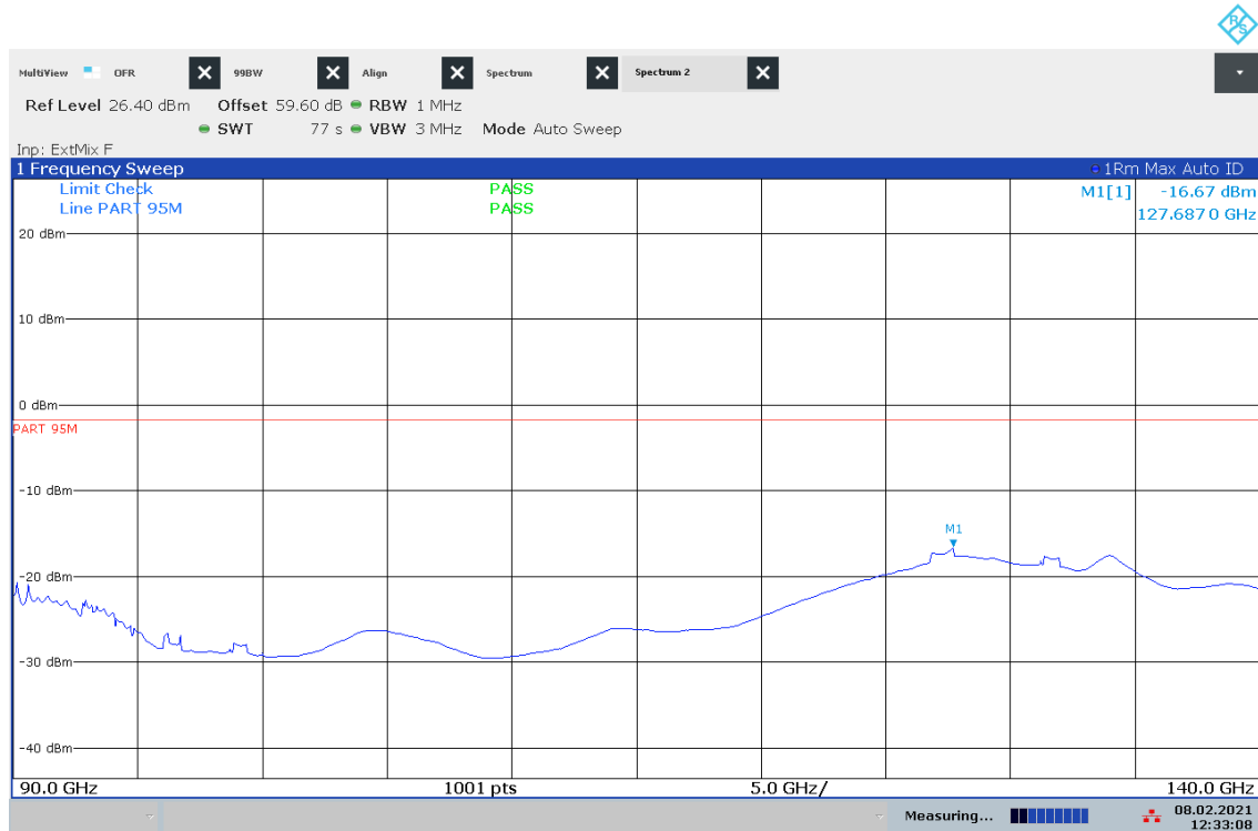
Plot 40: 90 GHz – 140 GHz, vertical / horizontal polarization, Mode 3
