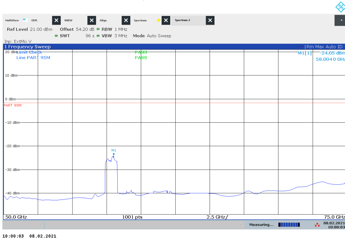
Plot 33: 50 GHz – 75 GHz, vertical / horizontal polarization, Mode 6
