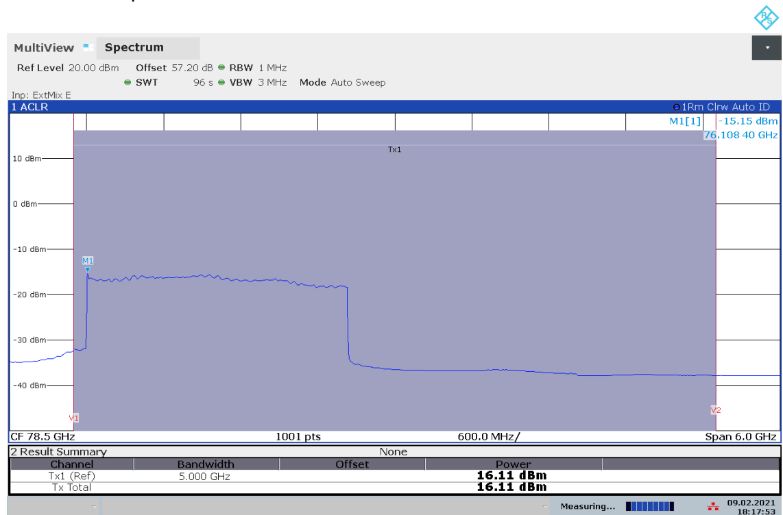
Plot 6: Mode 6 – Mean power
