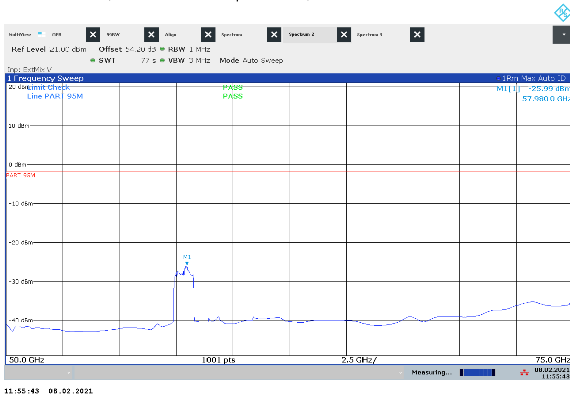
Plot 32: 50 GHz – 75 GHz, vertical / horizontal polarization, Mode 5
