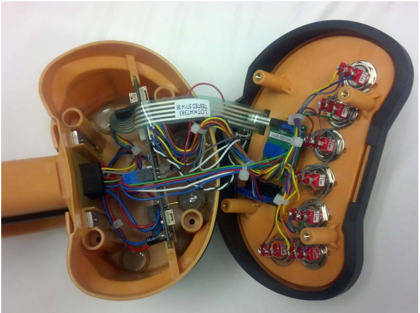
OVERVIEW OF INTERNAL CONSTRUCTION
