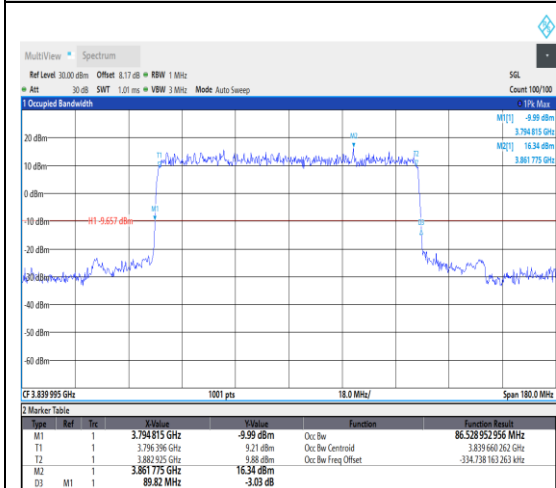
1-N77-3700-3980--30-90-M-2-DFT-PI2BPSK-Outer_Full-243@0-Ant1-86.529-89.820-≤90-PASS
