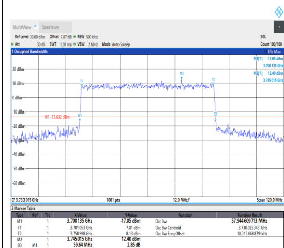
1-N77-3700-3980--30-60-L-6-CP-QPSK-Outer_Full-162@0-Ant1-57.945-59.640-≤60-PASS
