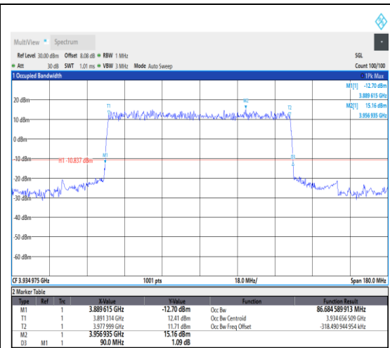
1-N77-3700-3980--30-90-H-2-DFT-PI2BPSK-Outer_Full-243@0-Ant1-86.685-90.000-≤90-PASS
