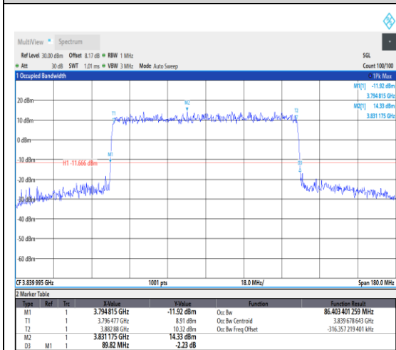
1-N77-3700-3980--30-90-M-4-DFT-64QAM-Outer_Full-243@0-Ant1-86.403-89.820-≤90-PA SS
