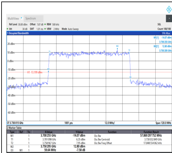
1-N77-3700-3980--30-60-L-4-DFT-64QAM-Outer_Full-162@0-Ant1-57.869-59.640-≤60-PA SS
