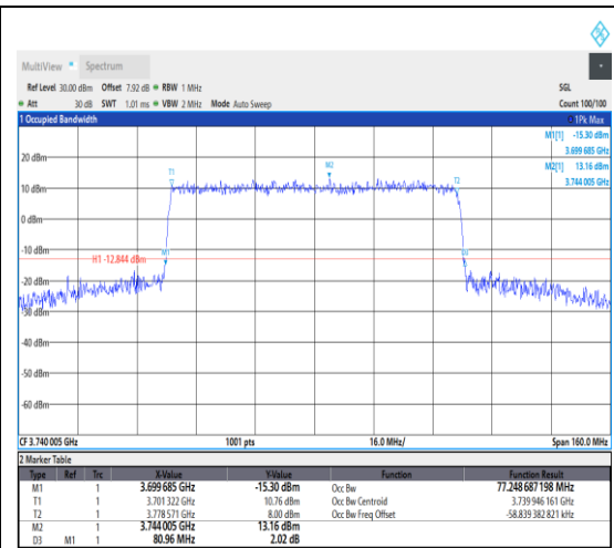
1-N77-3700-3980--30-80-L-7-CP-16QAM-Outer_Full-217@0-Ant1-77.249-80.960-≤80-PASS
