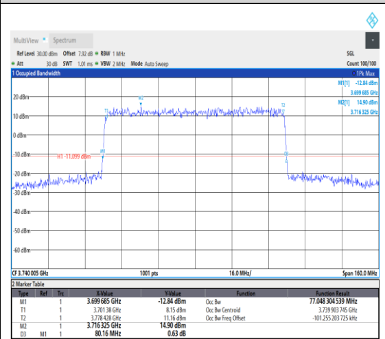
1-N77-3700-3980--30-80-L-1-DFT-QPSK-Out
