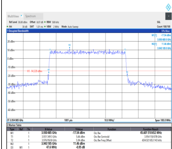
1-N77-3700-3980--30-50-H-5-DFT-256QAM-Out er_Full-128@0-Ant1-45.602-47.600-≤50-PASS
