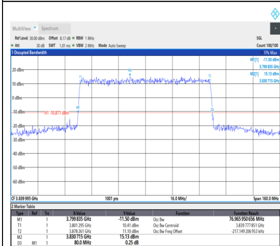
1-N77-3700-3980--30-80-M-1-DFT-QPSK-Outer_Full-217@0-Ant1-77.932-80.656-≤80-PASS
