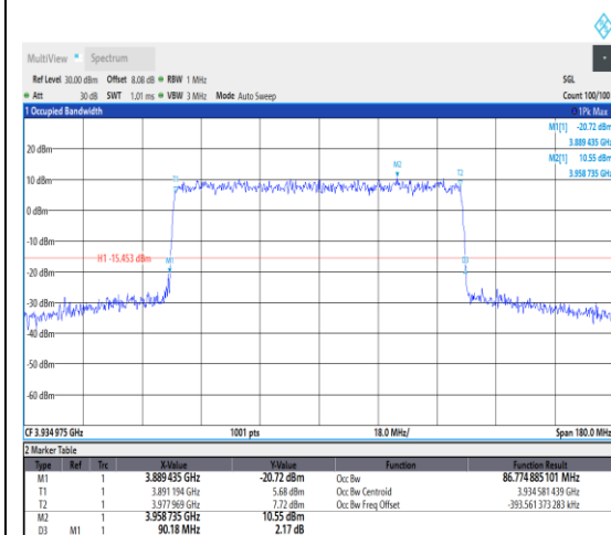
1-N77-3700-3980--30-90-H-5-DFT-256QAM-
