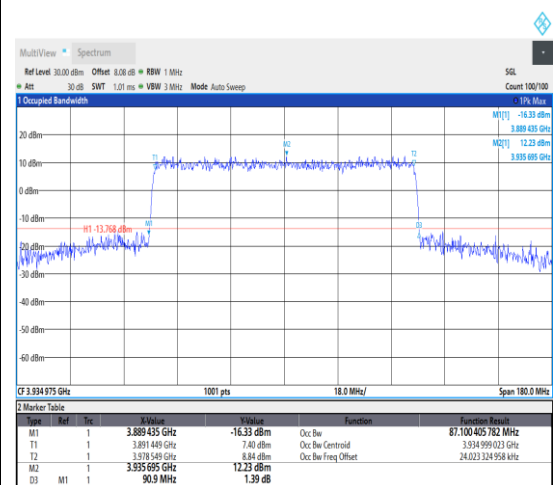
1-N77-3700-3980--30-90-H-6-CP-QPSK-Out
