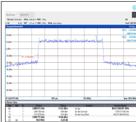
1-N77-3700-3980--30-90-H-1-DFT-QPSK-Outer_Full-243@0-Ant1-86.613-90.000-≤90-PA SS
