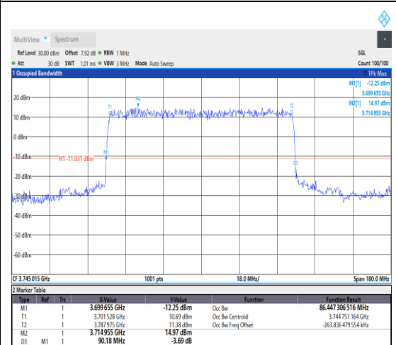
1-N77-3700-3980--30-90-L-2-DFT-PI2BPSK-Outer_Full-243@0-Ant1-86.447-90.180-≤90-PASS PASS
