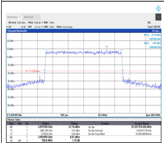
1-N77-3700-3980--30-100-H-9-CP-256QAM-
