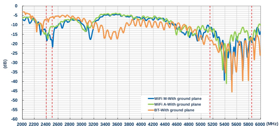
S11 (dB) – WiFi M & WiFi A & BT
