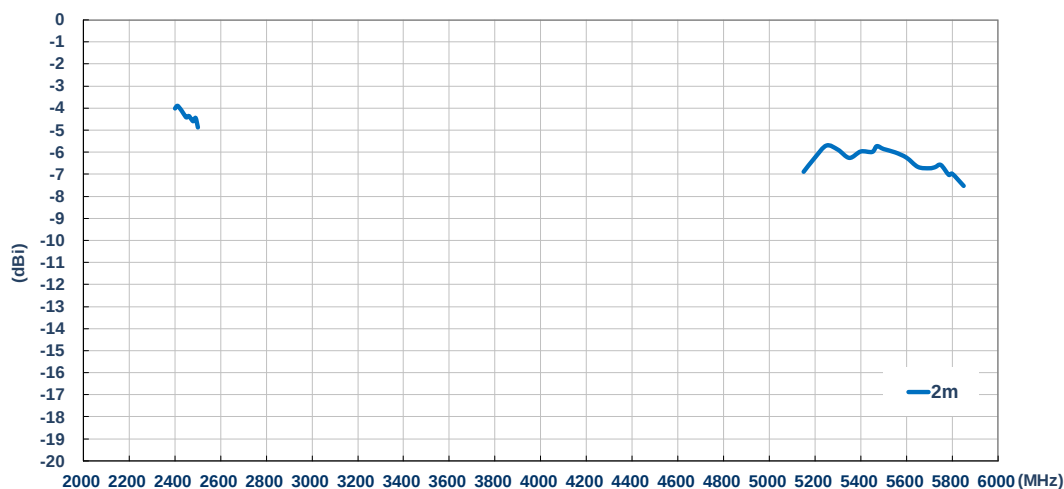
Peak Gain (dBi) – WiFi M
