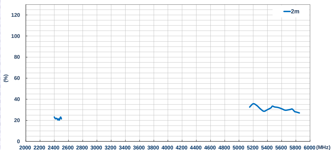
Efficiency (%) – BT
