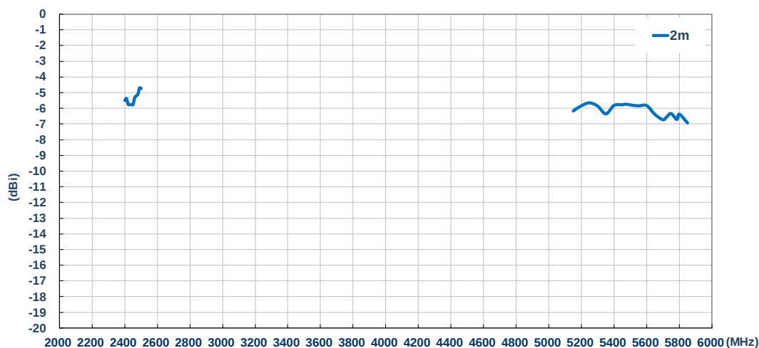
Peak Gain (dBi) – WiFi A
