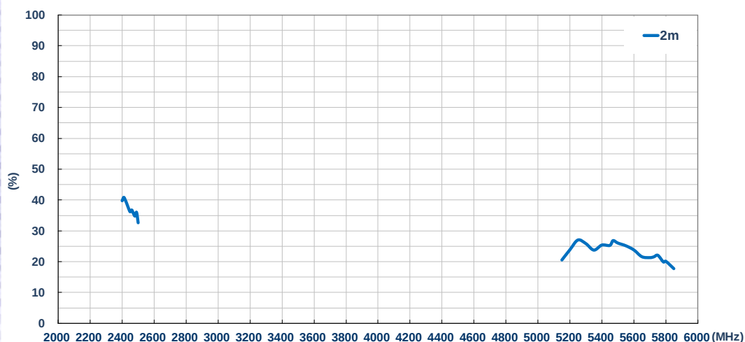
Efficiency (%) – WiFi M
