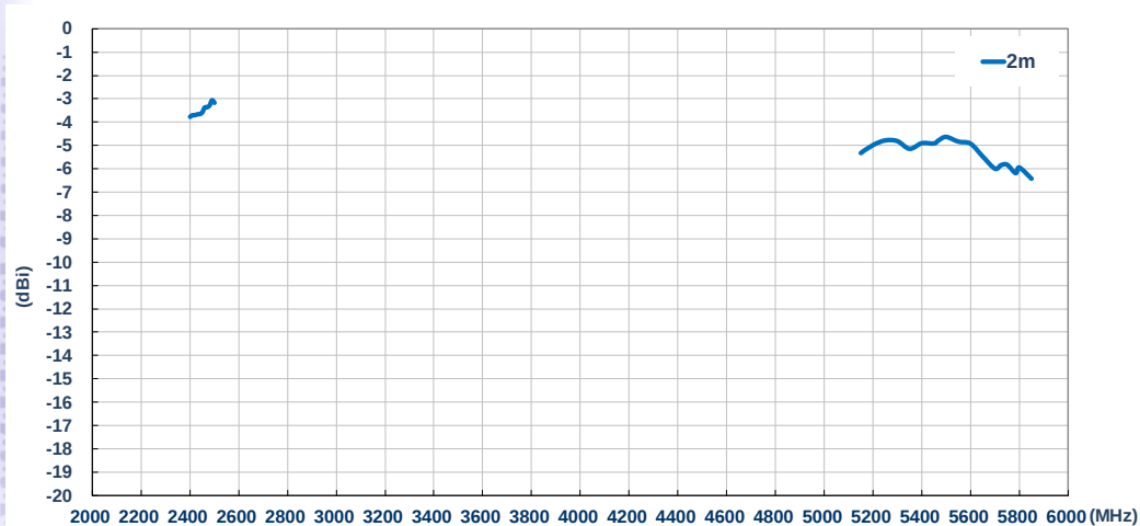
Average Gain (dBi) – WiFi A
