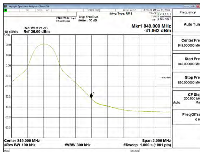
Bandedge B26 10M CH26990 QPSK(1,49)
