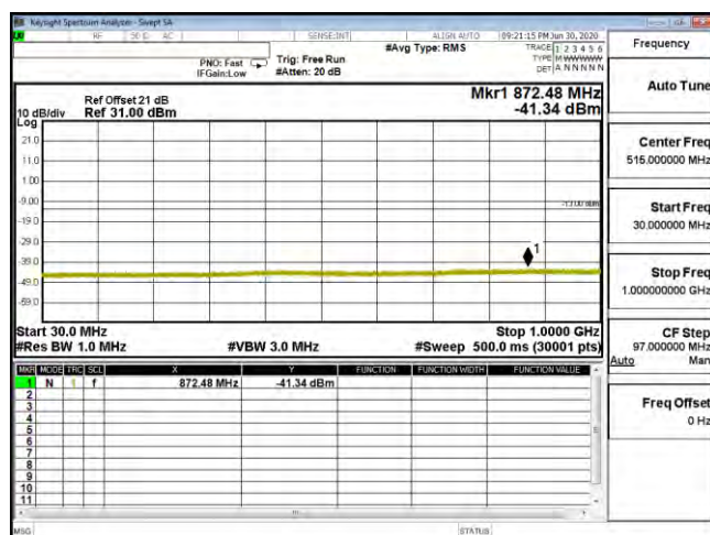
CSE B4 10M CH20000 QPSK(1,25) 30M-1G
