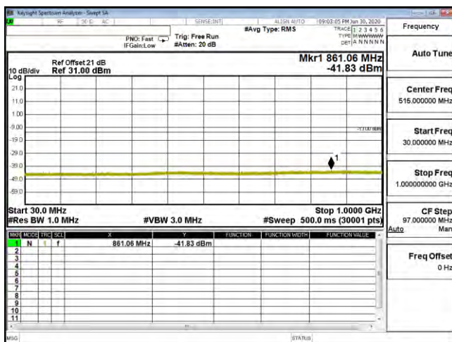
CSE B4 3M CH20385 16QAM(1,0) 30M-1G
