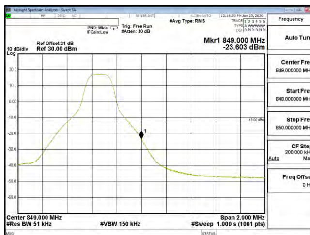
Bandedge B26 5M CH27015 16QAM(1,24)
