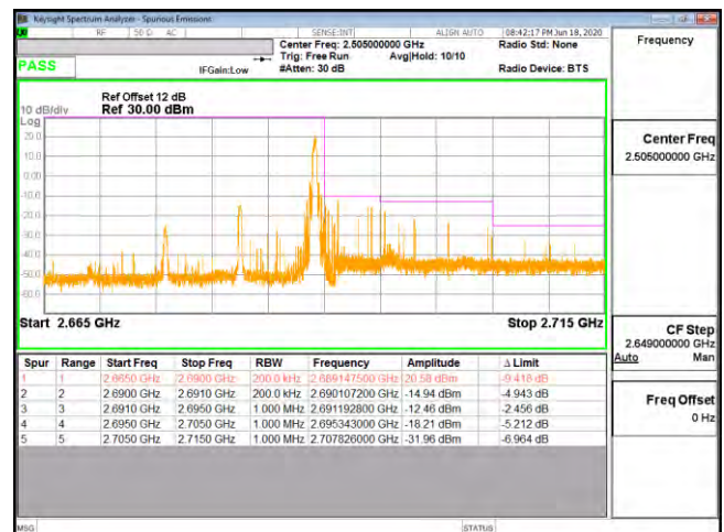
Bandedge B41 15M CH41515 64QAM(1,74)
