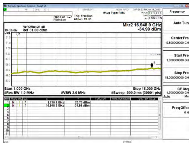
CSE B4 10M CH20000 QPSK(1,25) 1G-18G
