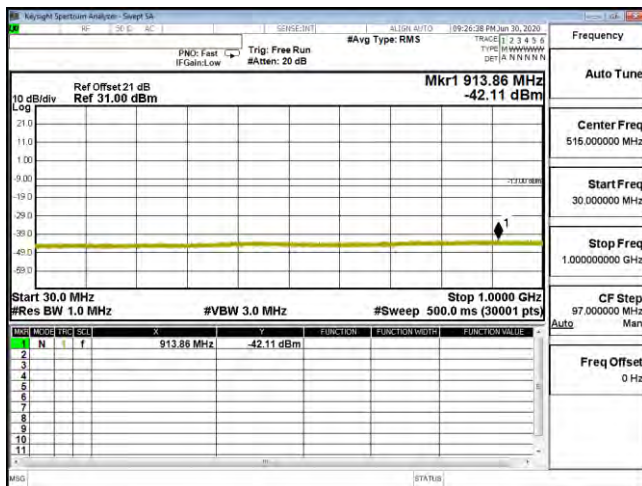
CSE B4 15M CH20175 16QAM(1,74) 30M-1G
