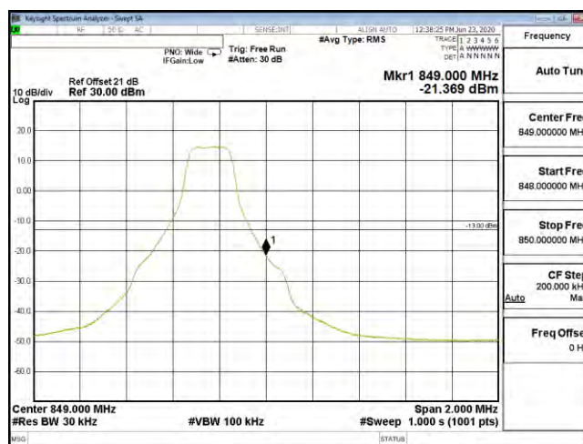
Bandedge B26 3M CH27025 16QAM(1,14)
