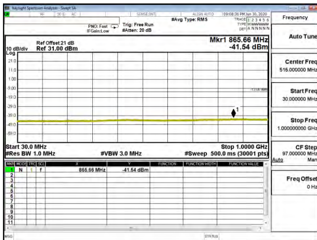
CSE B4 5M CH20175 16QAM(1,0) 30M-1G
