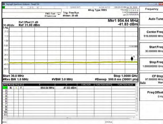
CSE B4 10M CH20350 16QAM(1,25) 30M-1G
