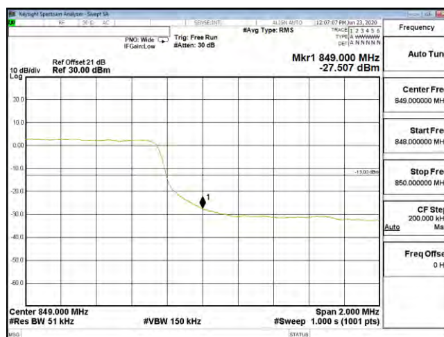
Bandedge B26 5M CH27015 QPSK(25,0)
