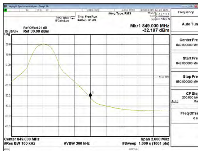
Bandedge B26 10M CH26990 16QAM(1,49)
