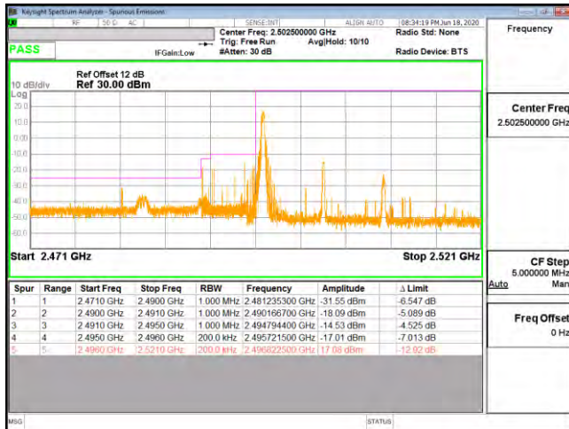
Bandedge B41 15M CH39725 QPSK(1,0)
