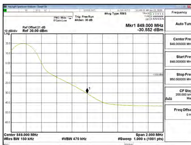
Bandedge B26 15M CH26965 64QAM(1,74)
