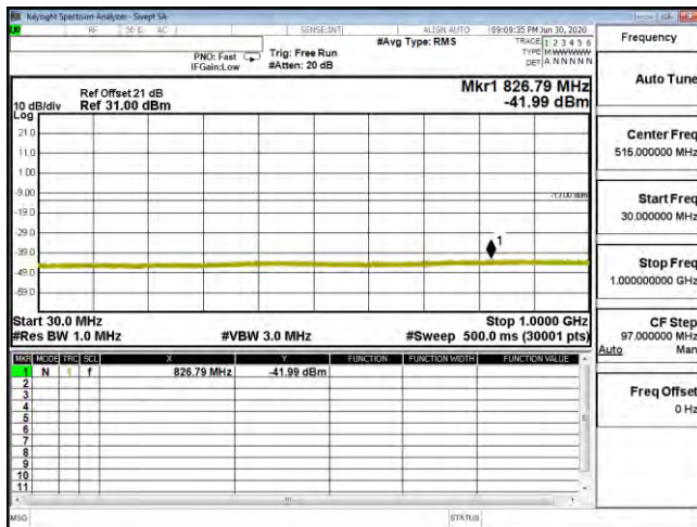
CSE B4 5M CH20375 QPSK(1,12) 30M-1G
