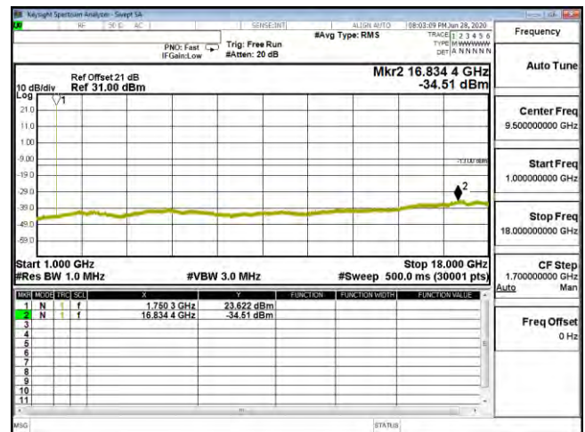
CSE B4 10M CH20350 16QAM(1,25) 1G-18G
