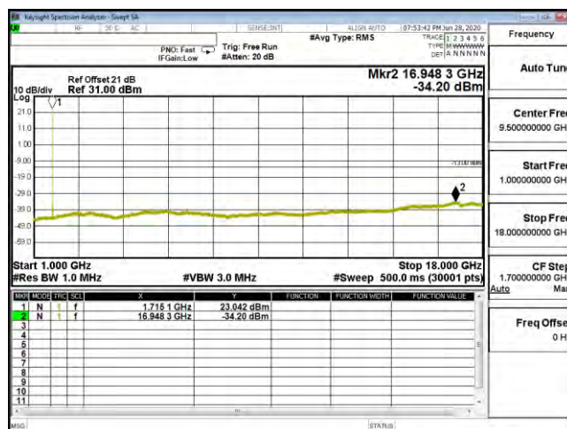
CSE B4 10M CH20000 64QAM(1,25) 1G-18G
