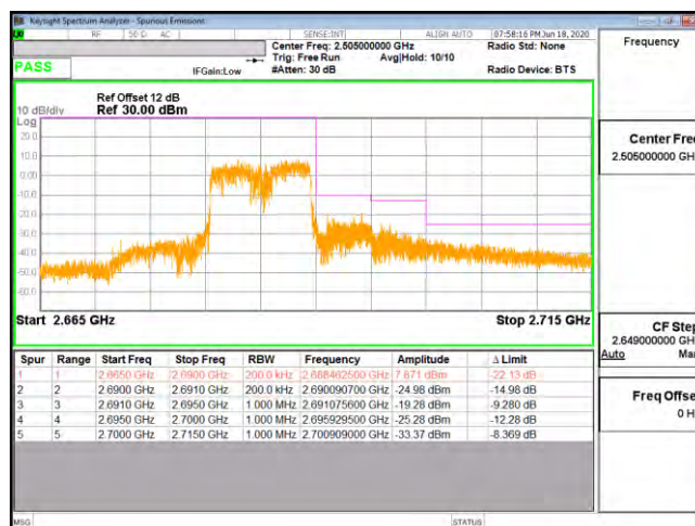
Bandedge B41 10M CH41450 64QAM(50,0)
