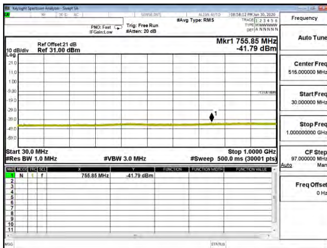
CSE B4 1.4M CH20393 16QAM(1,0) 30M-1G
