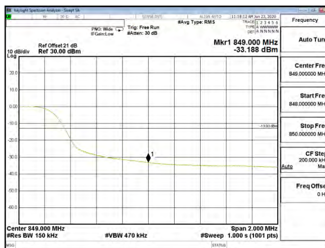
Bandedge B26 15M CH26965 16QAM(75,0)
