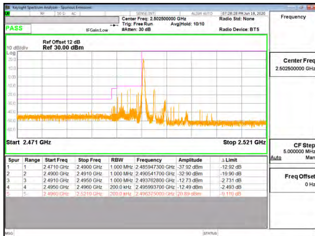
Bandedge B41 5M CH39675 16QAM(1,0)
