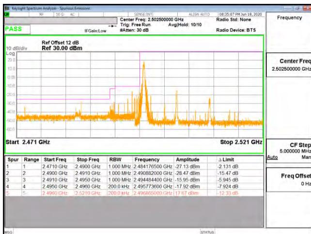
Bandedge B41 15M CH39725 64QAM(1,0)
