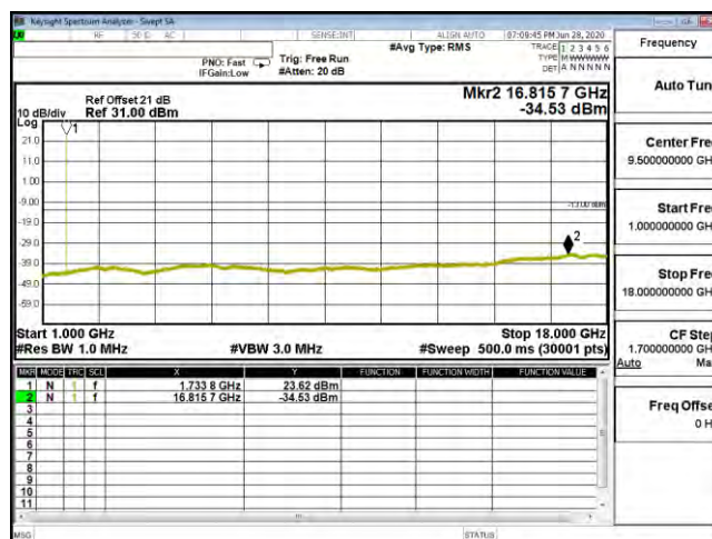
CSE B4 3M CH20175 64QAM(1,14) 1G-18G
