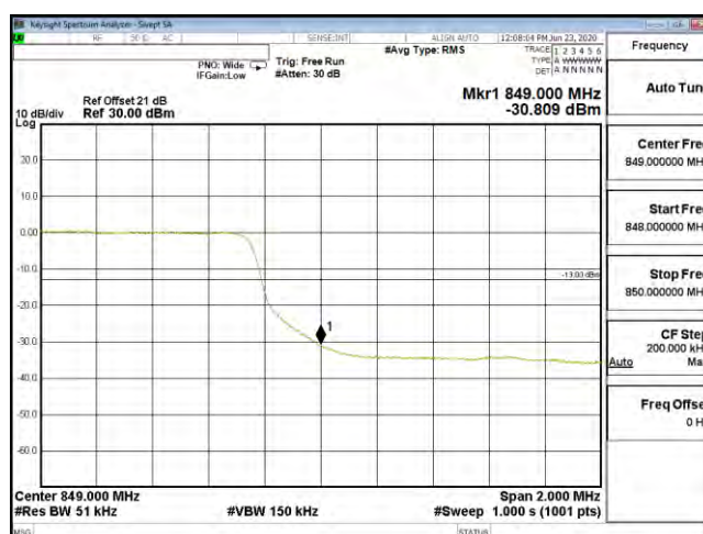
Bandedge B26 5M CH27015 64QAM(25,0)
