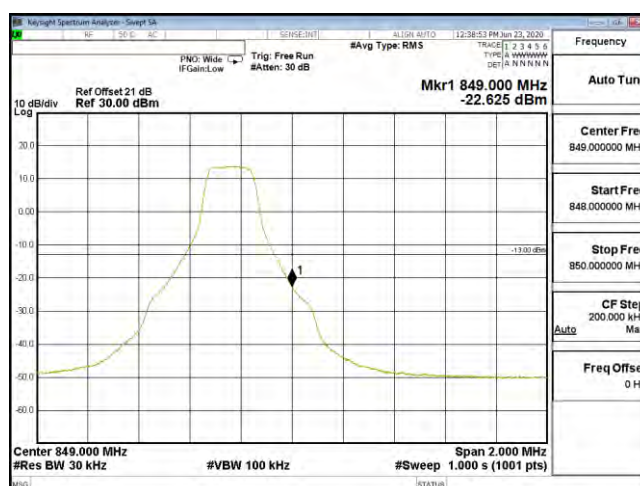
Bandedge B26 3M CH27025 64QAM(1,14)
