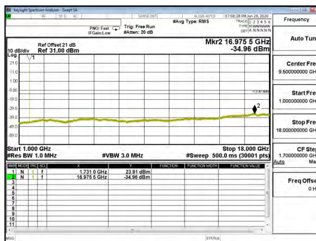
CSE B4 3M CH20175 16QAM(1,0) 1G-18G
