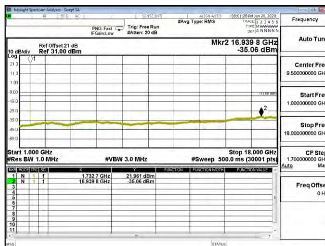
CSE B4 10M CH20175 64QAM(1,25) 1G-18G
