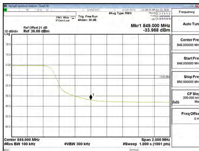
Bandedge B26 10M CH26990 64QAM(50,0)
