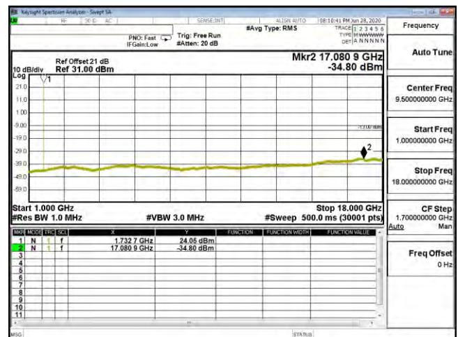
CSE B4 15M CH20175 64QAM(1,37) 1G-18G
