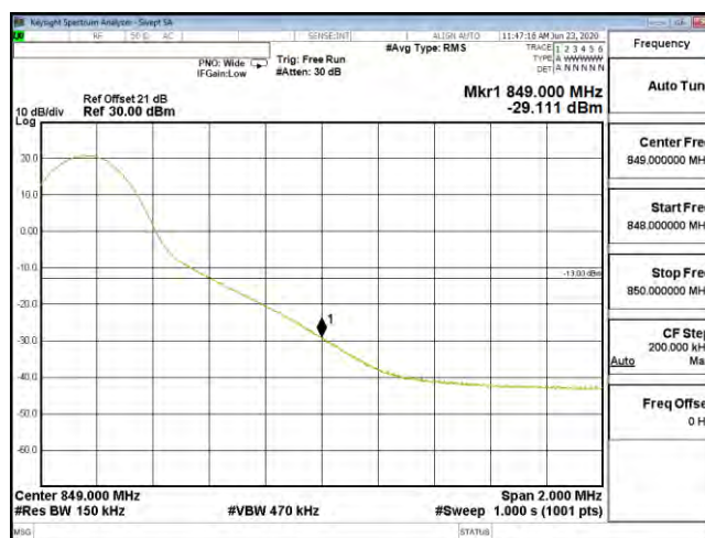
Bandedge B26 15M CH26965 16QAM(1,74)
