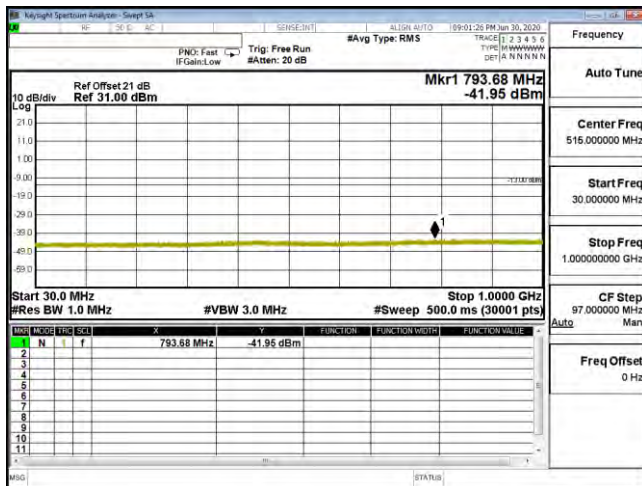
CSE B4 3M CH19965 QPSK(1,14) 30M-1G
