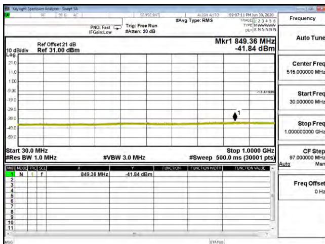
CSE B4 5M CH19975 64QAM(1,12) 30M-1G
