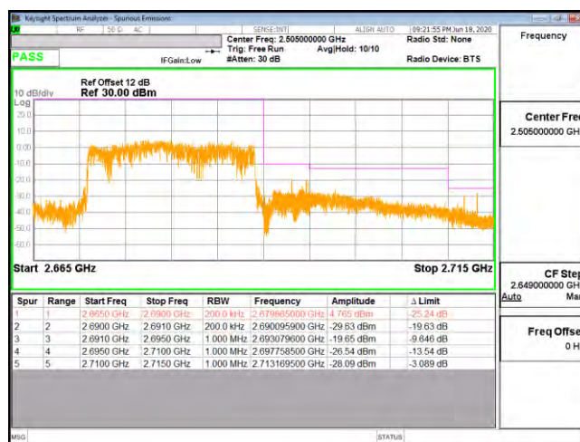
Bandedge B41 20M CH41490 16QAM(100,0)
