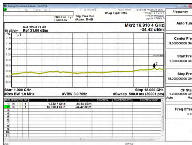
CSE B4 10M CH20175 QPSK(1,25) 1G-18G
