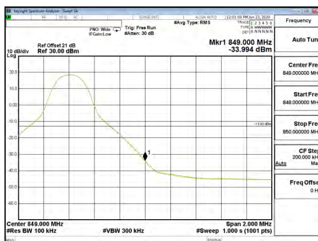
Bandedge B26 10M CH26990 64QAM(1,49)
