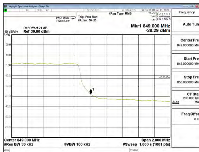
Bandedge B26 3M CH27025 16QAM(15,0)
