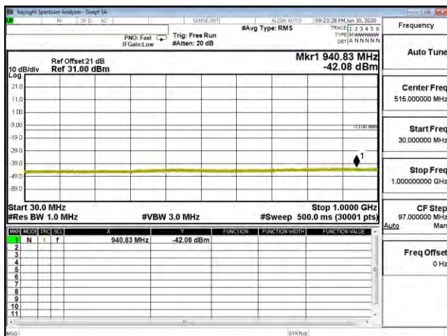
CSE B4 10M CH20350 64QAM(1,25) 30M-1G
