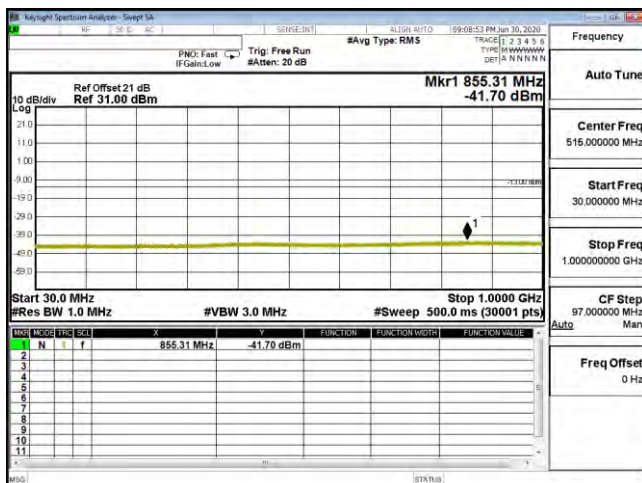
CSE B4 5M CH20175 64QAM(1,12) 30M-1G
