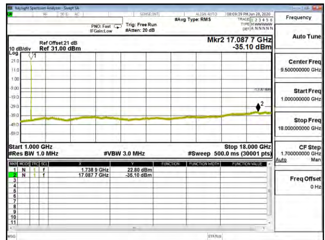
CSE B4 15M CH20175 16QAM(1,74) 1G-18G
