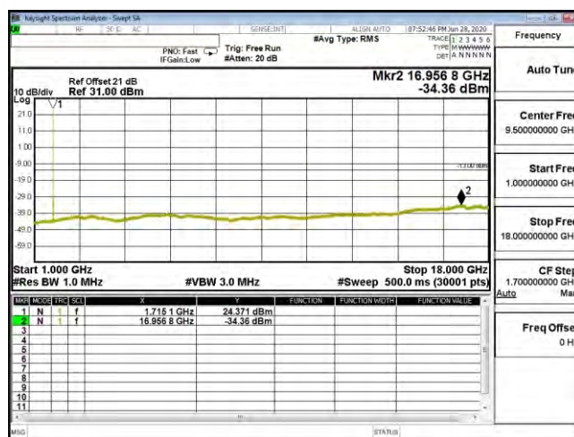
CSE B4 10M CH20000 16QAM(1,25) 1G-18G
