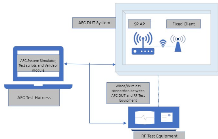
Diagram 2: AFC DUT Setup for Standard Power Access Point (non-standalone) with Proxy
