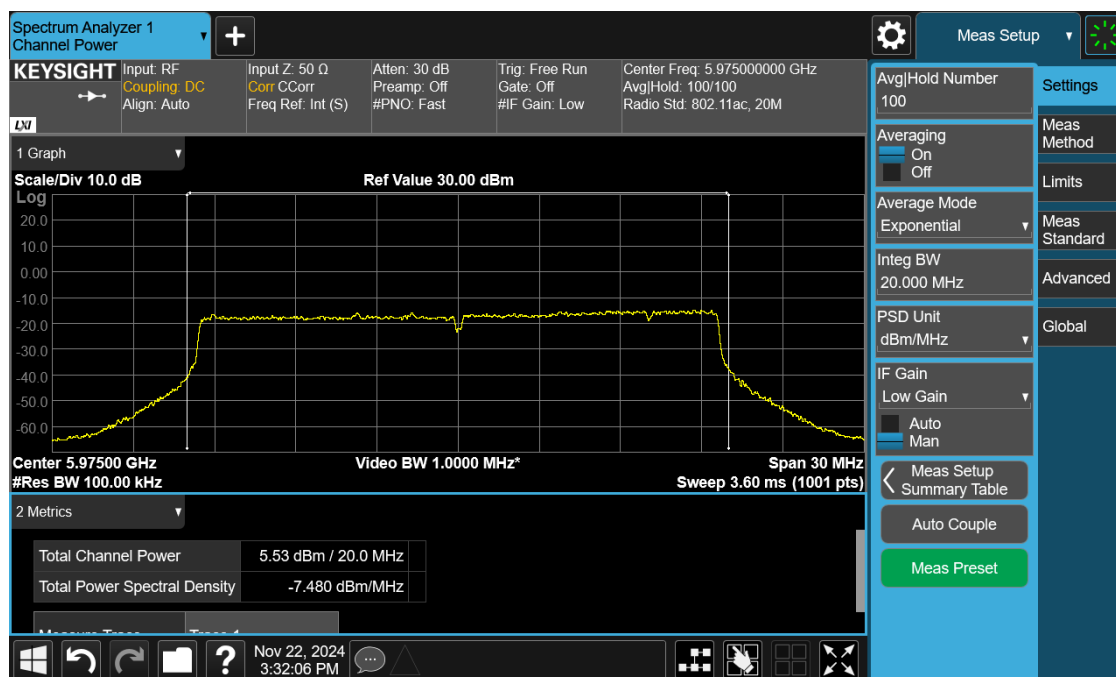
Plot 3: Power and PSD for Standard Power – 5975 MHz
