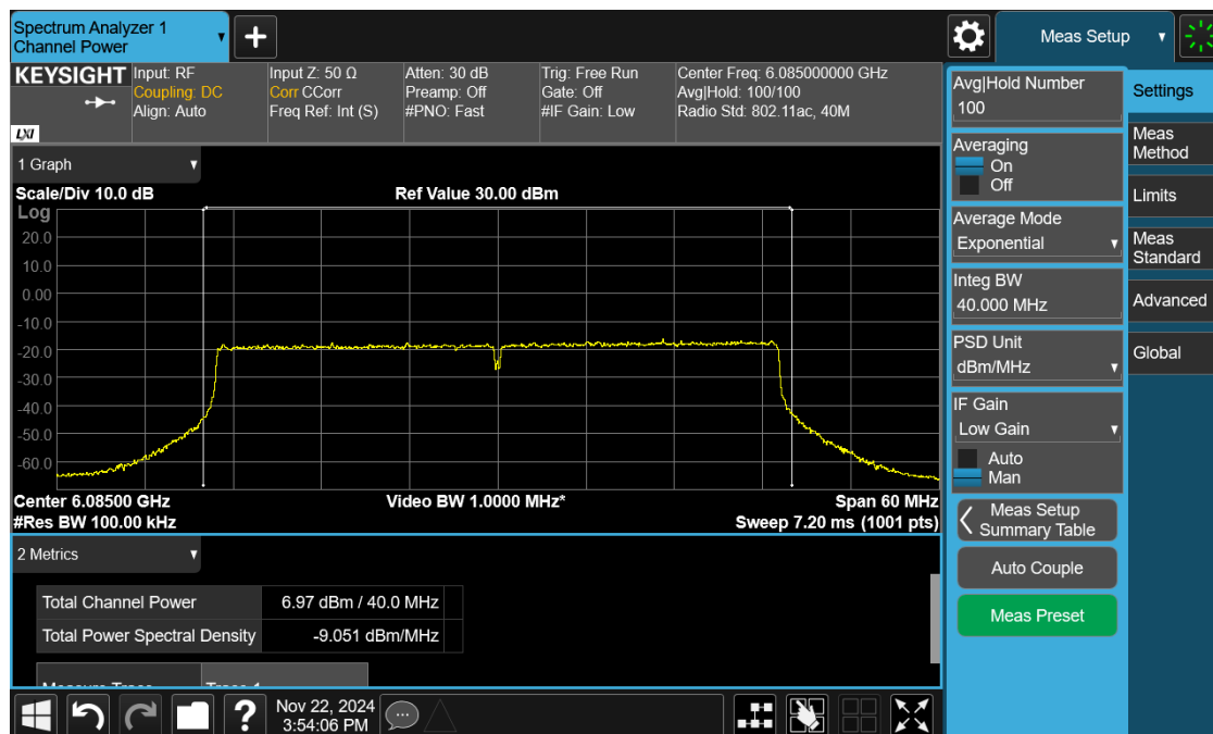
Plot 5: Power and PSD for Standard Power – 6085 MHz
