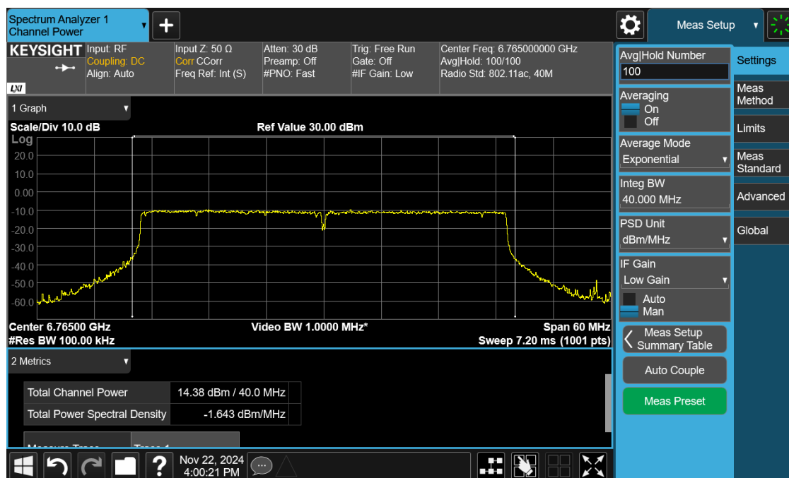
Plot 6: Power and PSD for Standard Power – 6765 MHz
