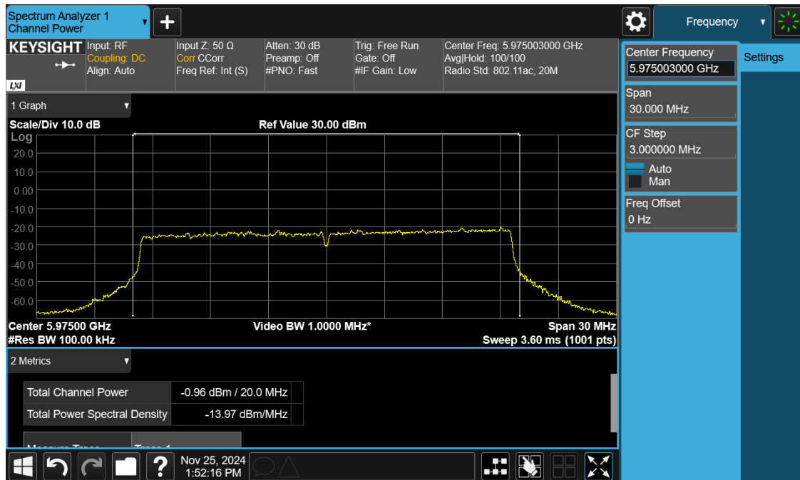
Plot 20: Power and PSD for Low-Power Indoor – 5975 MHz
