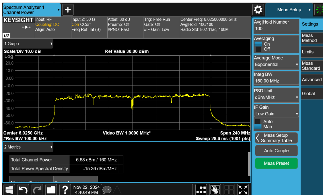
Plot 10: Power and PSD for Low-Power Indoor – 6025 MHz
