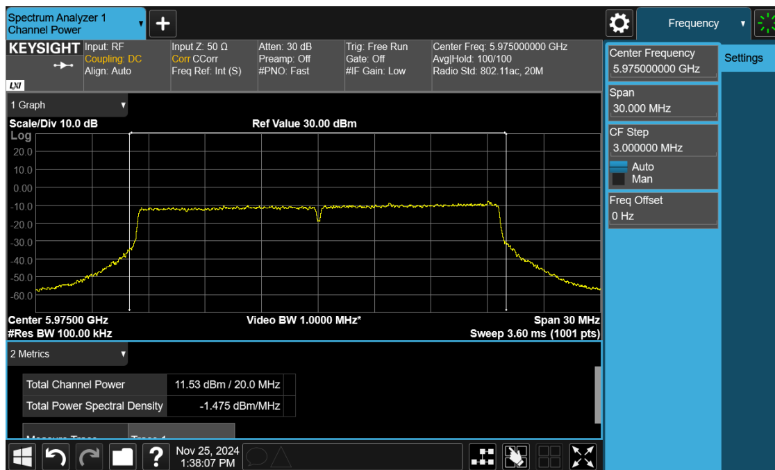
Plot 19: Power and PSD for Standard Power – 5975 MHz
