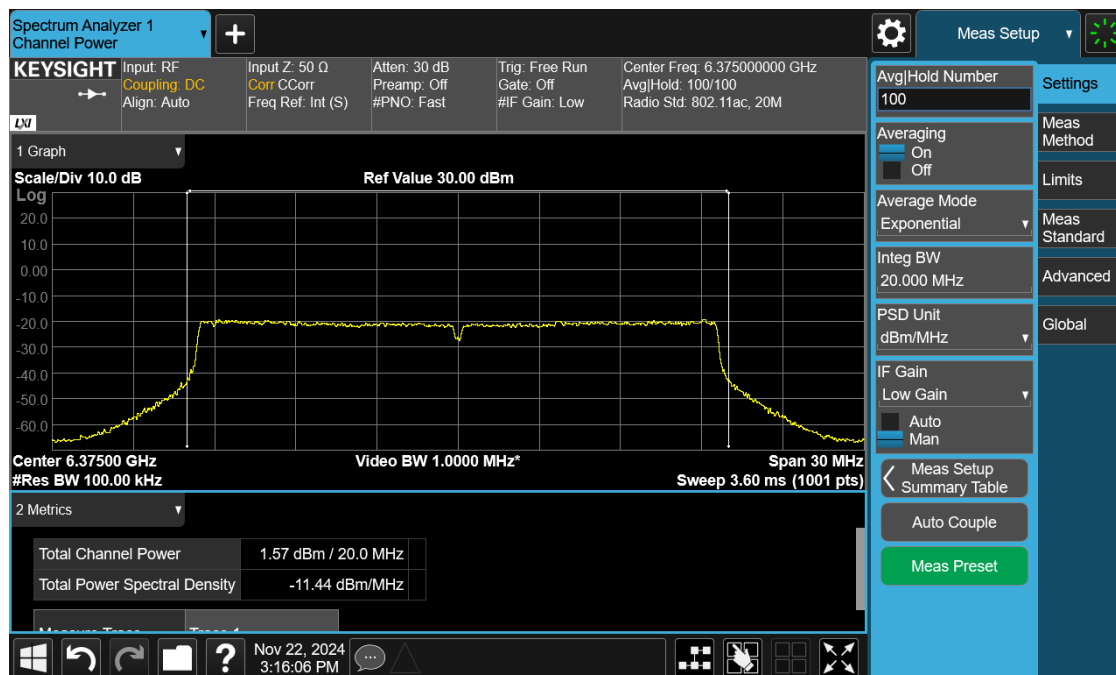
Plot 2: Power and PSD for Standard Power – 6375 MHz
