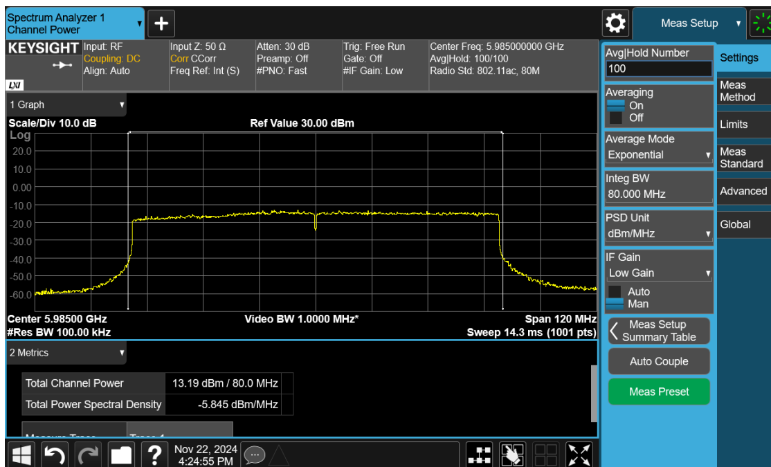
Plot 8: Power and PSD for Standard Power – 5985 MHz
