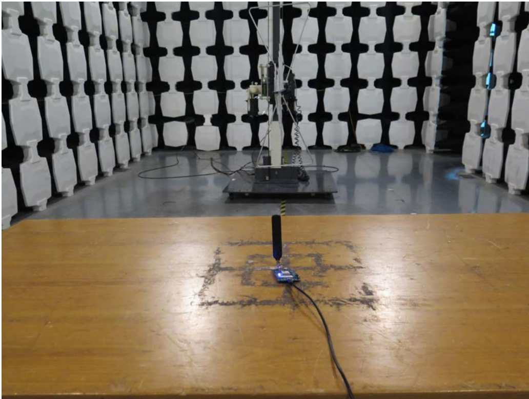
Pic1. Radiated emissions
