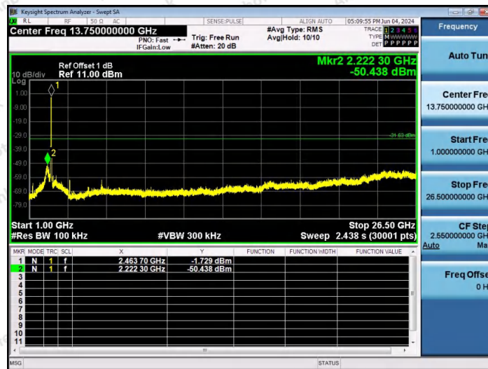
11AX40SISO-Ant1-2452-1000~26500-PASS
