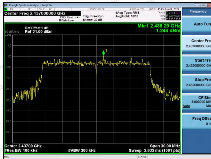
11AX20SISO-Ant1-2437-0~Reference-PASS
