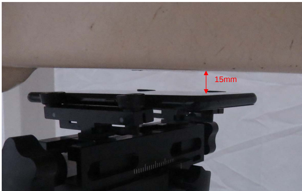
Picture 8: Front Side, the distance from handset to the bottom of the Phantom is 15mm
