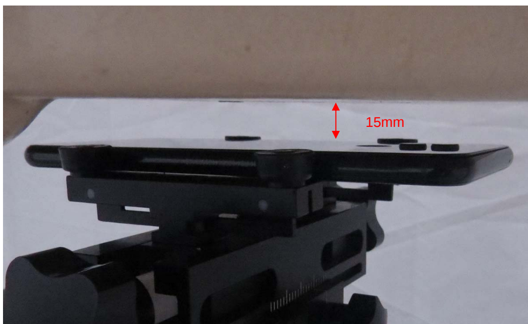
Picture 6: Back Side, the distance from handset to the bottom of the Phantom is 15mm
