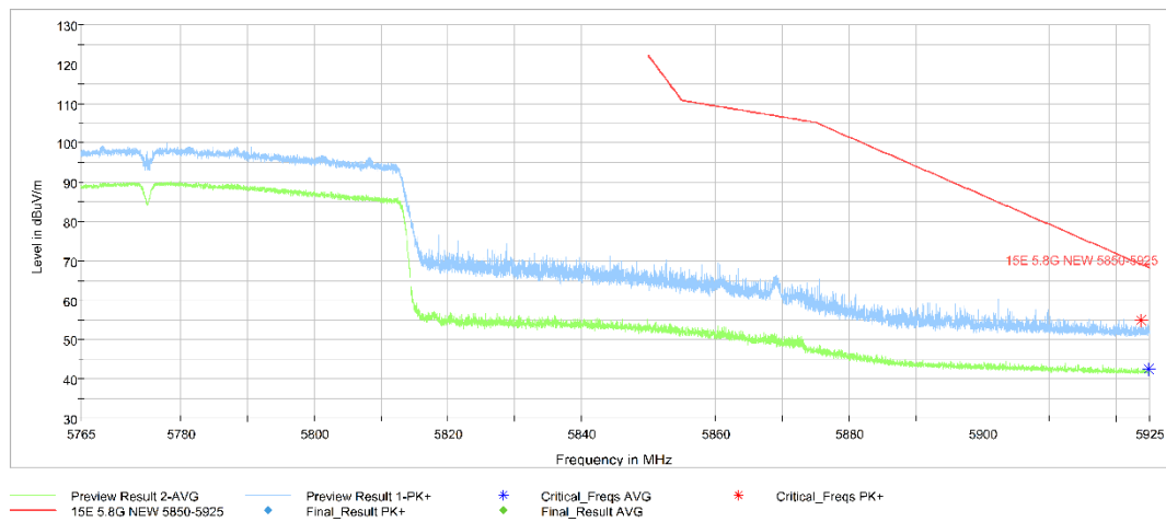
Fig. 12 Band Edges (802.11ac-HT80, 5775MHz)
