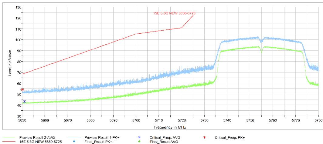
Fig. 9 Band Edges (802.11ac-HT40 Ch151, 5755MHz)
