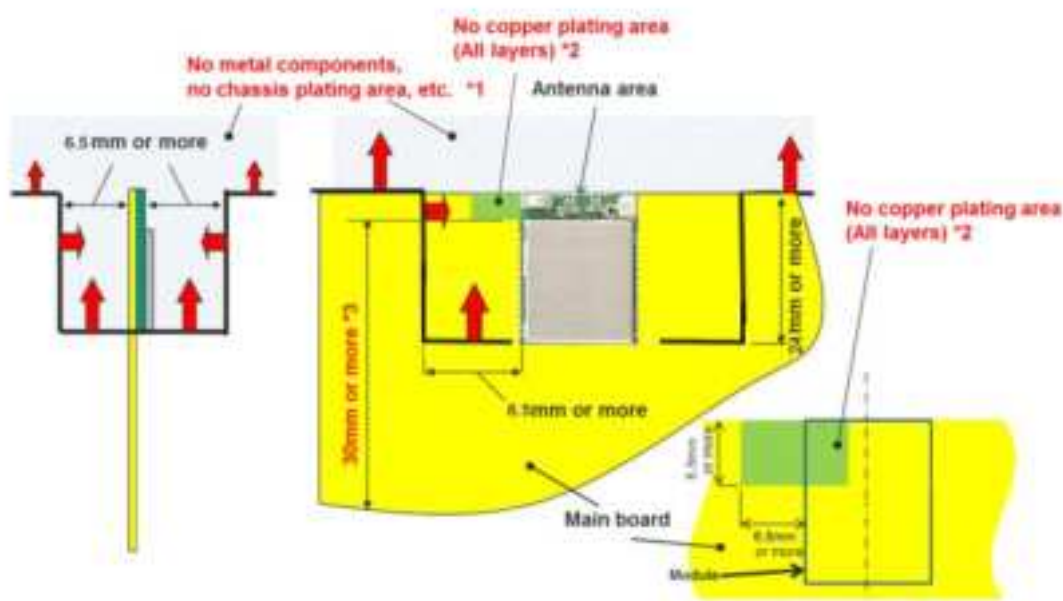
Figure 4: Module mounting example
