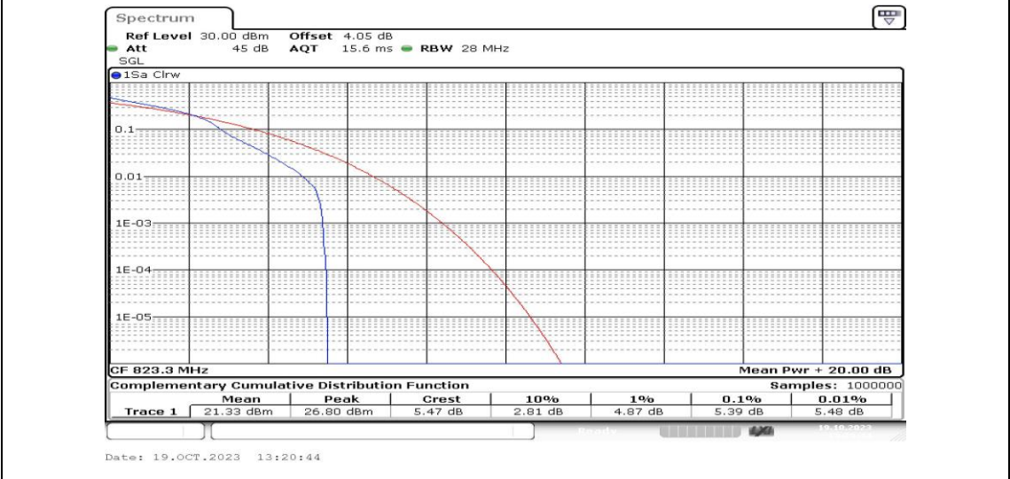
Band26-1.4MHz-16QAM-26783-1RB#0-PASS
