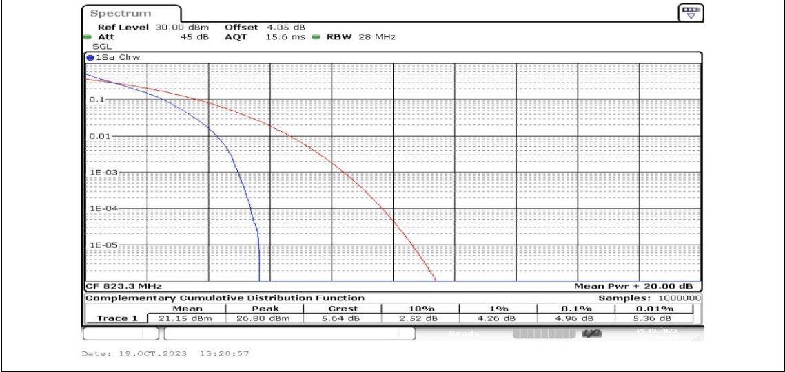
Band26-1.4MHz-QPSK-26783-6RB#0-PASS
