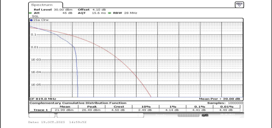
Band26-10MHz-QPSK-26740-1RB#0-PASS
