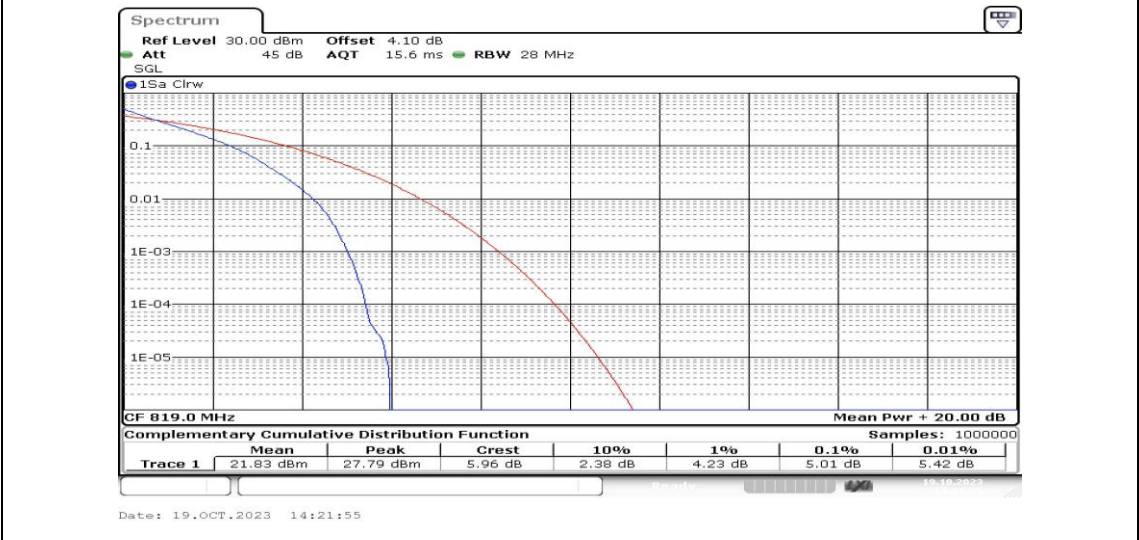
Band26-3MHz-QPSK-26740-15RB#0-PASS
