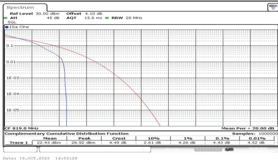
Band26-5MHz-QPSK-26740-1RB#0-PASS
