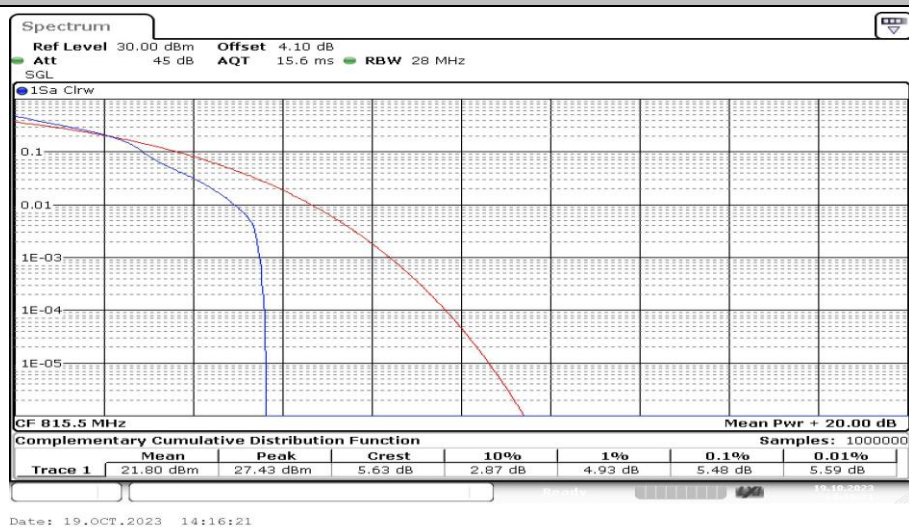
Band26-3MHz-16QAM-26705-1RB#0-PASS
