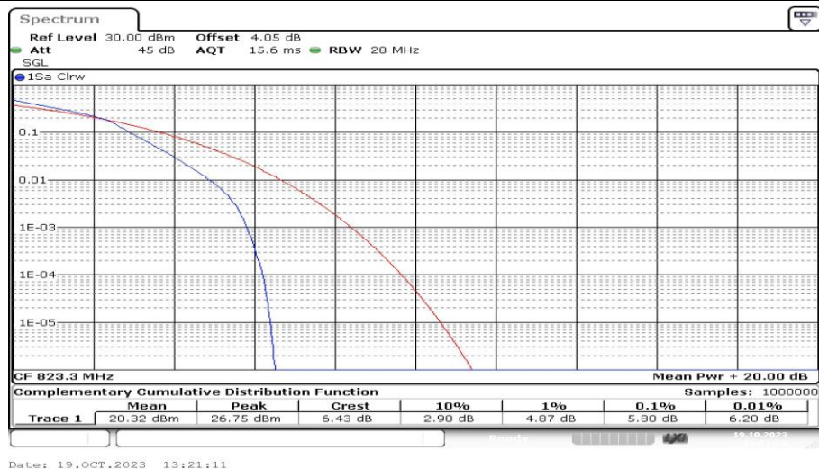
Band26-1.4MHz-16QAM-26783-6RB#0-PASS
