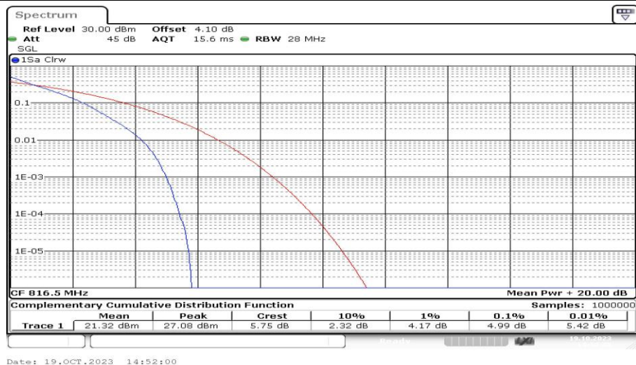
Band26-5MHz-QPSK-26715-25RB#0-PASS
