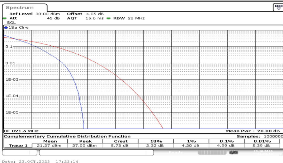
Band26-5MHz-QPSK-26765-25RB#0-PASS
