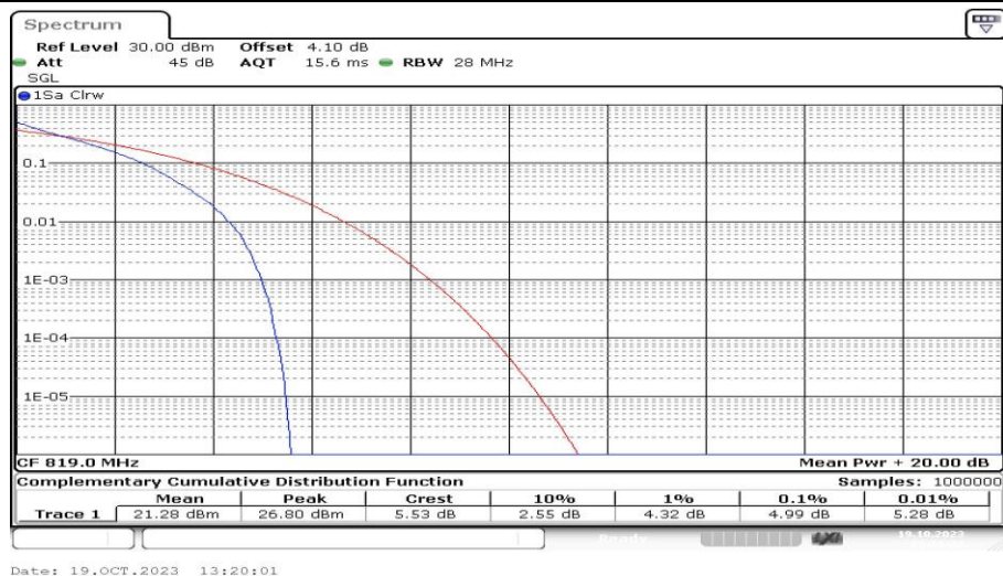
Band26-1.4MHz-QPSK-26740-6RB#0-PASS
