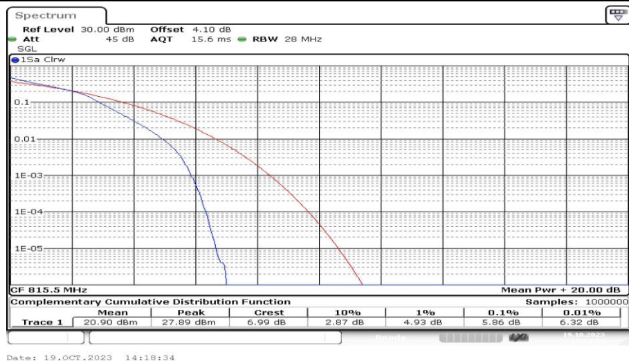
Band26-3MHz-16QAM-26705-15RB#0-PASS
