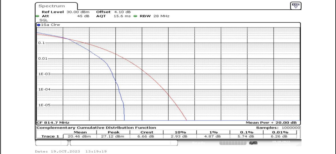
Band26-1.4MHz-16QAM-26697-6RB#0-PASS
