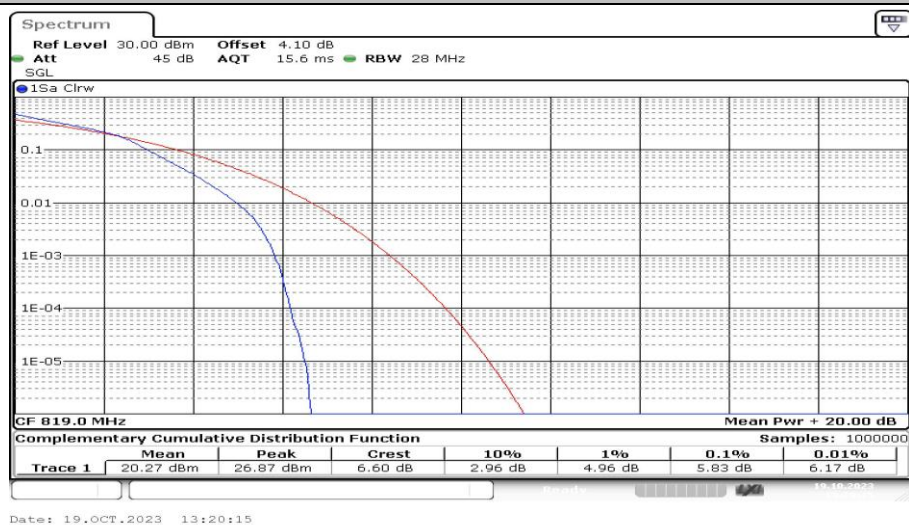
Band26-1.4MHz-16QAM-26740-6RB#0-PASS
