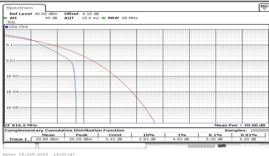
Band26-5MHz-16QAM-26715-1RB#0-PASS
