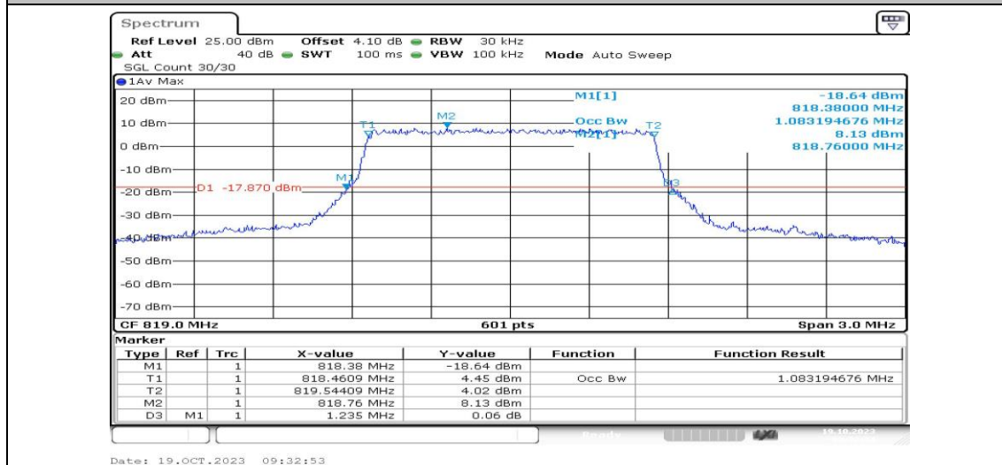
Band26-1.4MHz-16QAM-26740-6RB#0-PASS
