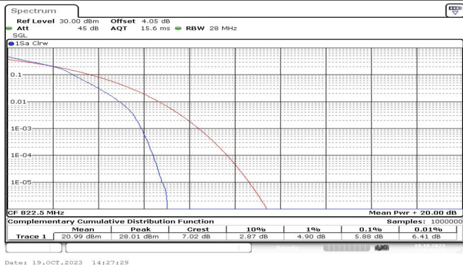
Band26-3MHz-16QAM-26775-15RB#0-PASS
