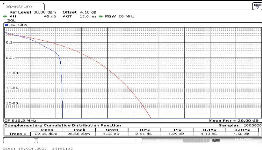
Band26-5MHz-QPSK-26715-1RB#0-PASS
