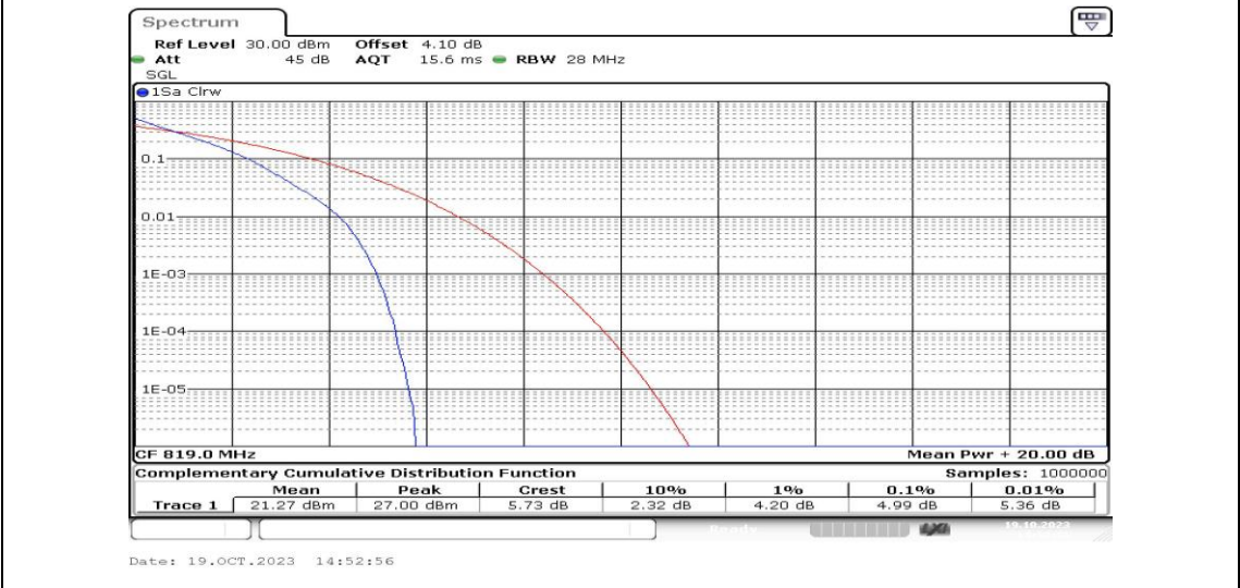
Band26-5MHz-QPSK-26740-25RB#0-PASS
