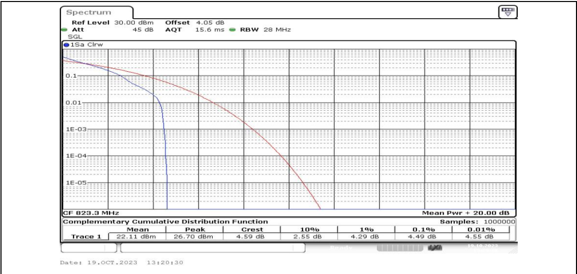
Band26-1.4MHz-QPSK-26783-1RB#0-PASS
