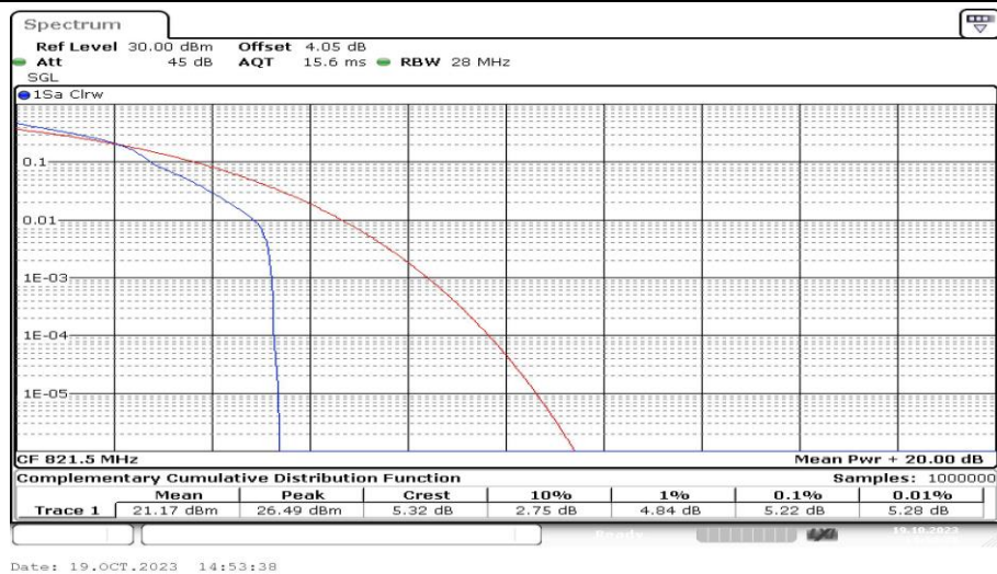
Band26-5MHz-16QAM-26765-1RB#0-PASS
