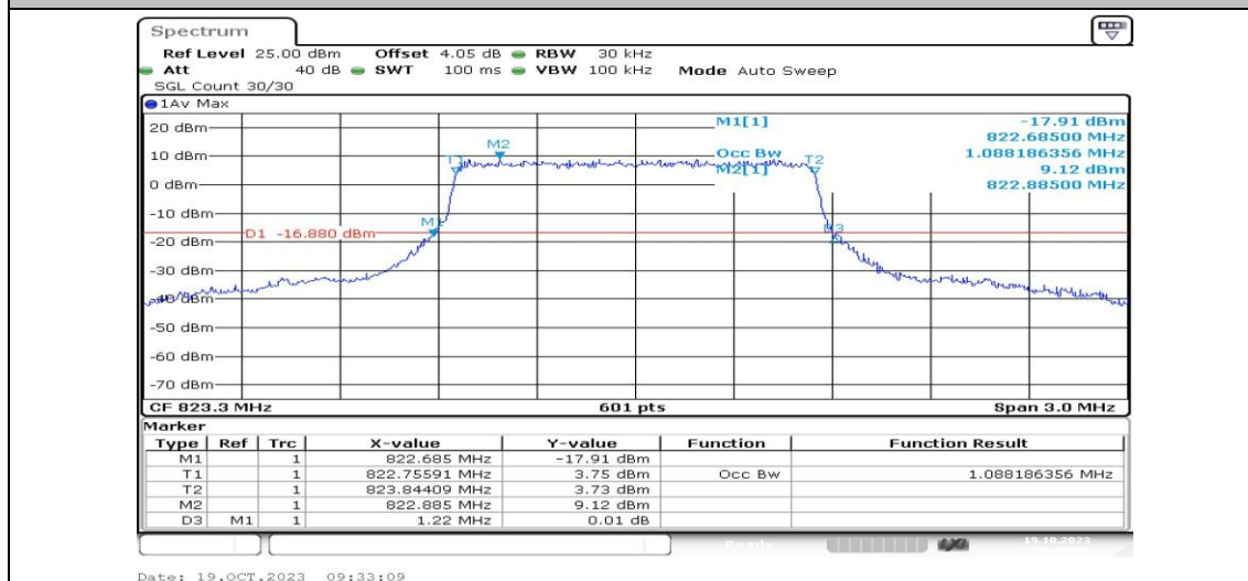
Band26-1.4MHz-QPSK-26783-6RB#0-PASS
