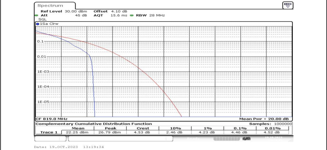
Band26-1.4MHz-QPSK-26740-1RB#0-PASS
