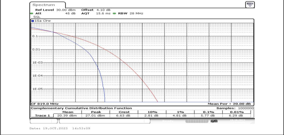
Band26-5MHz-16QAM-26740-25RB#0-PASS
