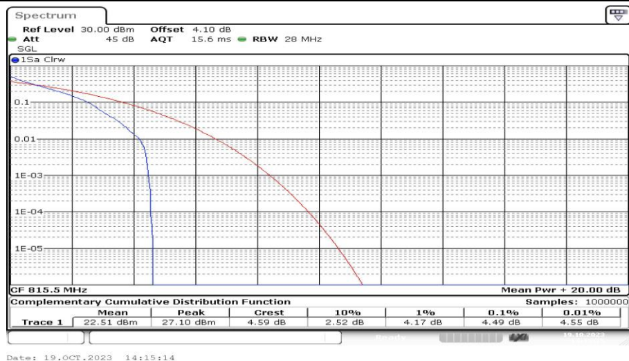
Band26-3MHz-QPSK-26705-1RB#0-PASS
