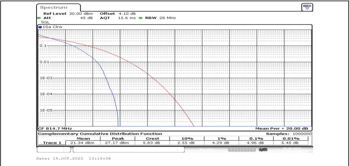
Band26-1.4MHz-QPSK-26697-6RB#0-PASS
