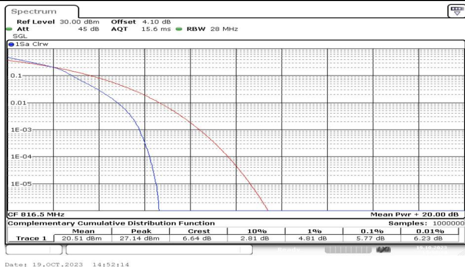
Band26-5MHz-16QAM-26715-25RB#0-PASS
