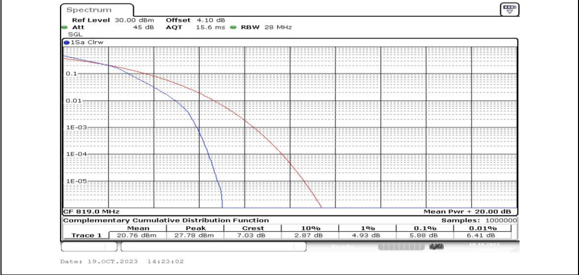
Band26-3MHz-16QAM-26740-15RB#0-PASS
