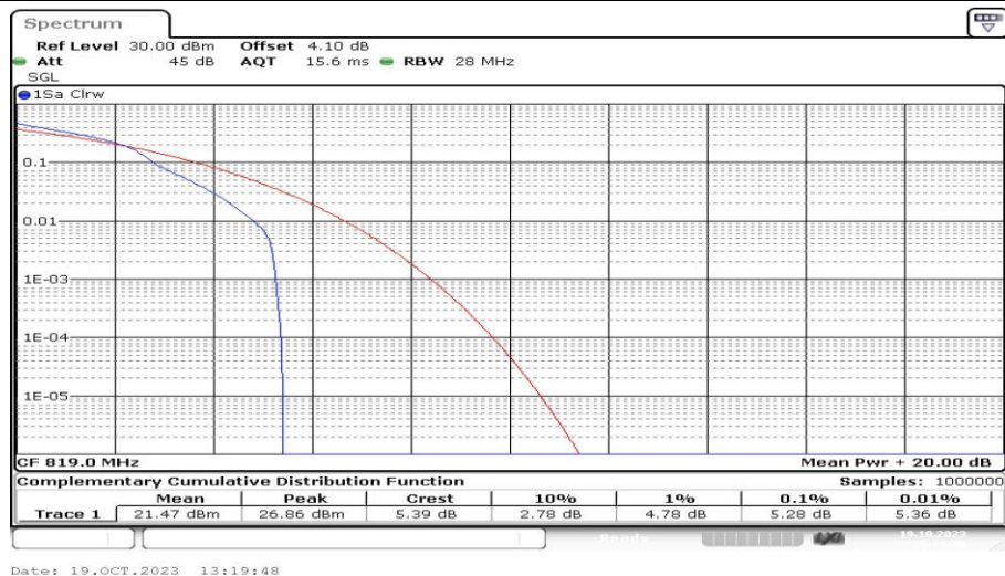
Band26-1.4MHz-16QAM-26740-1RB#0-PASS
