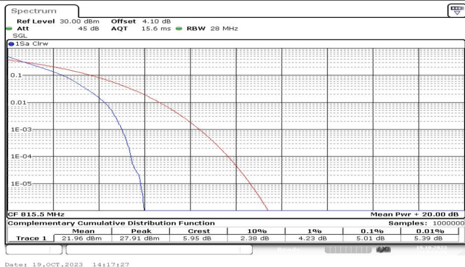
Band26-3MHz-QPSK-26705-15RB#0-PASS
