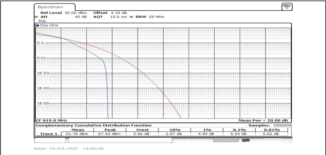
Band26-3MHz-16QAM-26740-1RB#0-PASS
