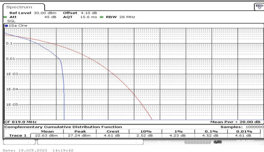
Band26-3MHz-QPSK-26740-1RB#0-PASS
