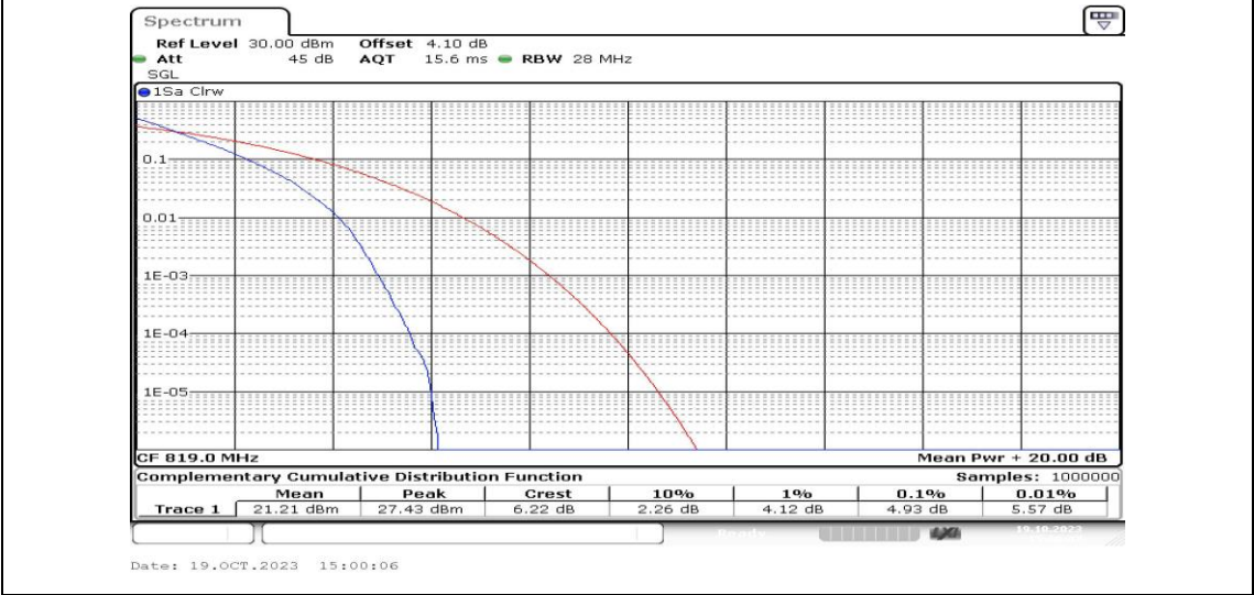
Band26-10MHz-QPSK-26740-50RB#0-PASS
