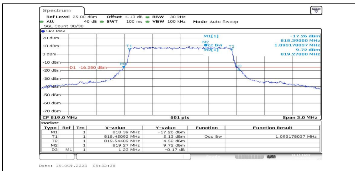
Band26-1.4MHz-QPSK-26740-6RB#0-PASS
