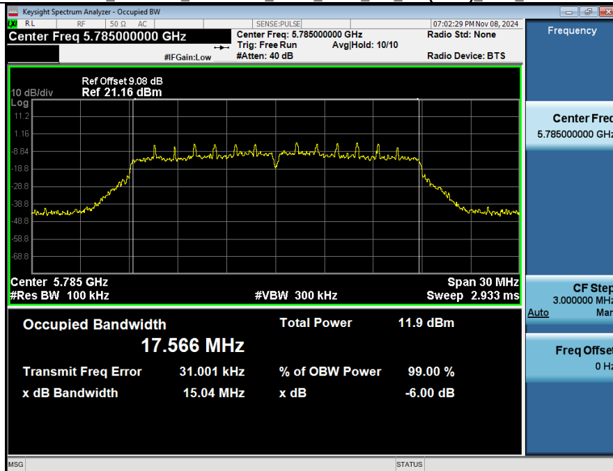
-6dB_Emission_Bandwidth_NVNT_ANT2_802_11n(HT20)_5785_20M
