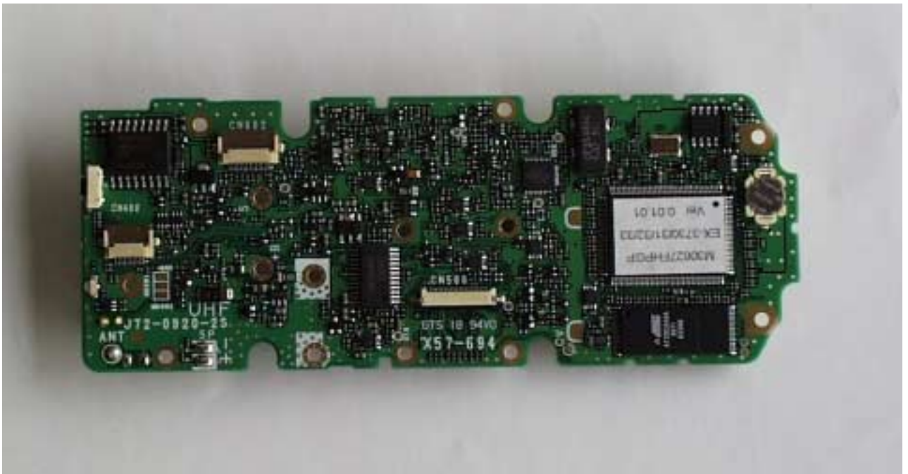
TXRX Foil Side View
