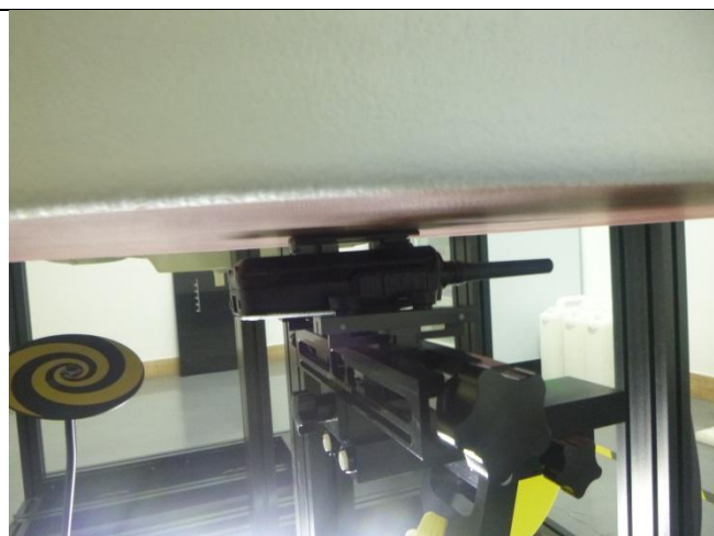
Body-worn(0mm)
