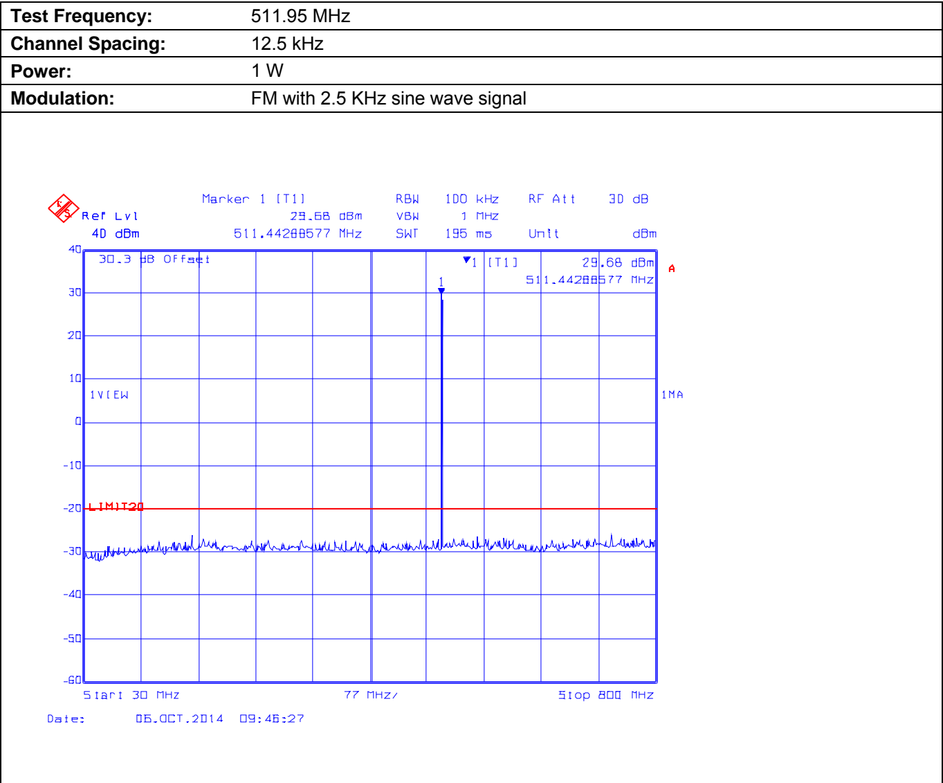
Plot 5.9.4.3.3. Conducted Transmitter Spurious Emissions for 511.95 MHz, Low Power, 30 MHz - 800 MHz
