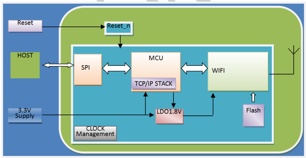
Figure 1-1 RAK49X System Diagram
