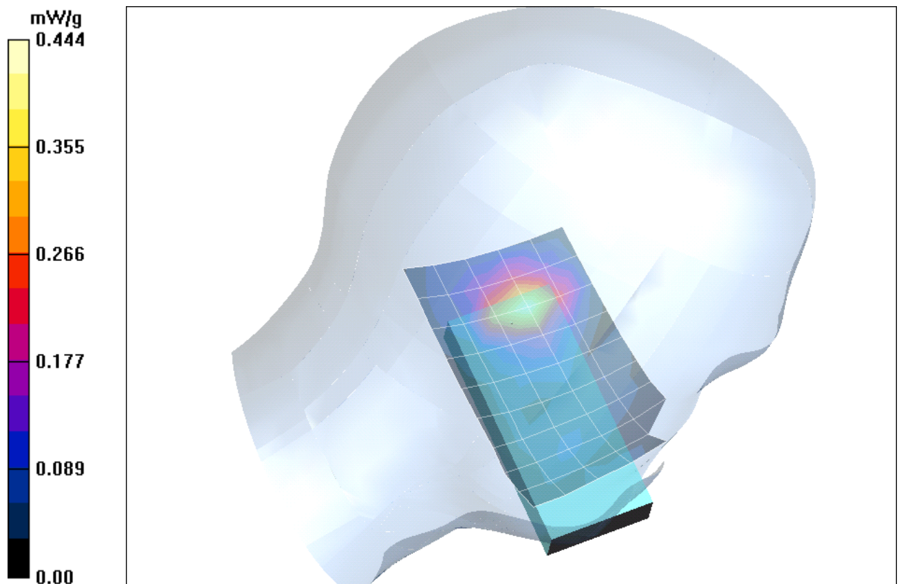
Fig. 2: SAR distribution for PCS 1900, channel 661, tilted position, left side of head (05.13.2005; Ambient Temperature: 21.1° C; Liquid Temperature: 20.6° C).
